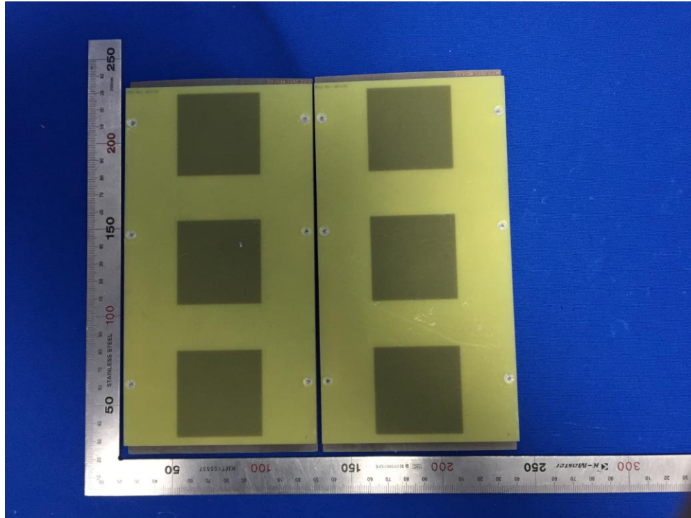
(7) EUT Photo (Panel Antenna)
