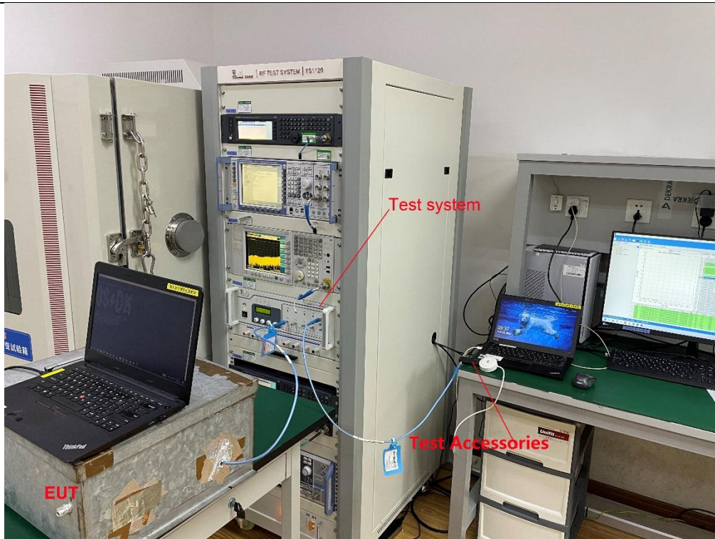
Description: DFS - EUT in shielding box
