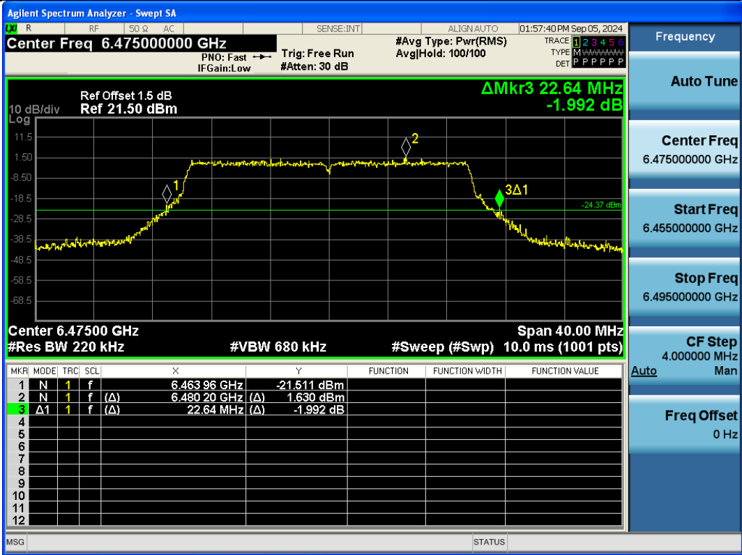
11AX20SISO-Ant1-6475
