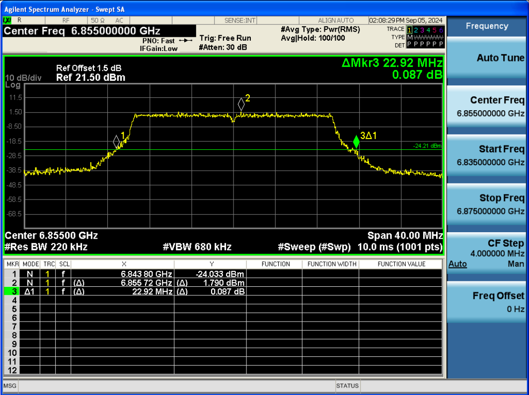
11AX20SISO-Ant1-6855
