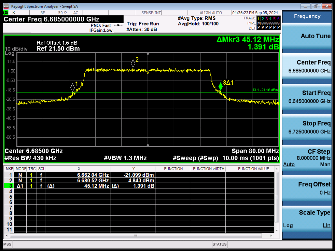
11AX40SISO-Ant1-6685
