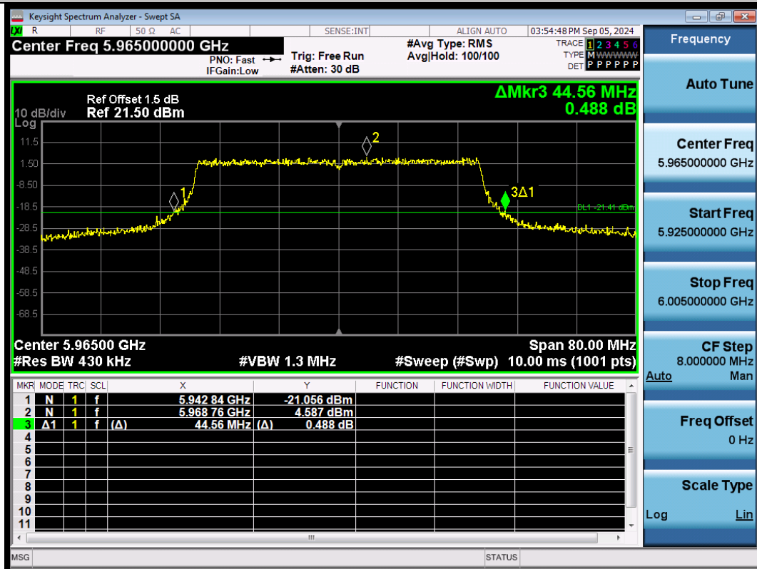
11AX40SISO-Ant1-5965
