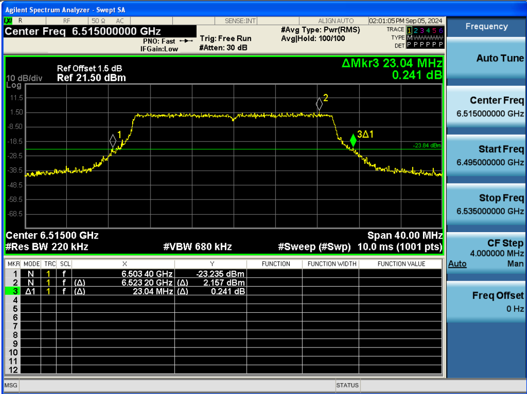
11AX20SISO-Ant1-6515
