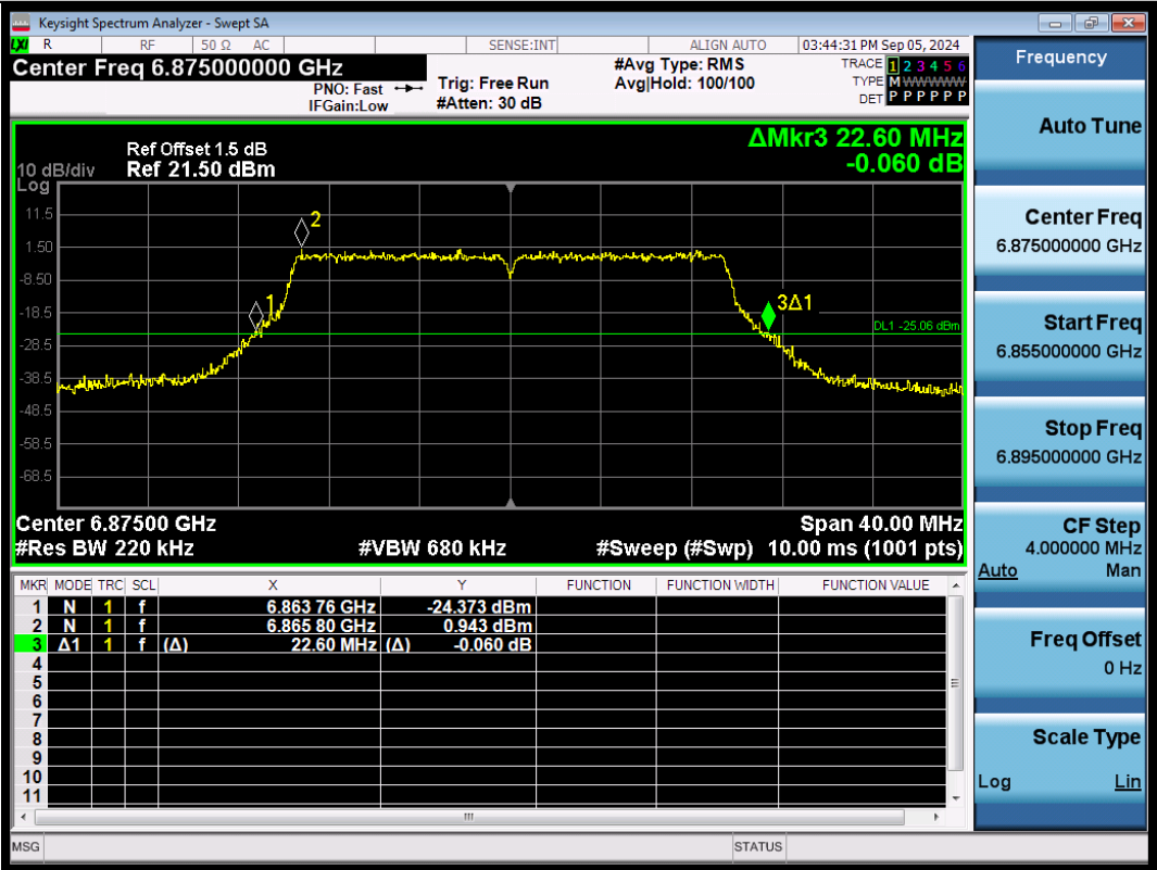
11AX20SISO-Ant1-6875
