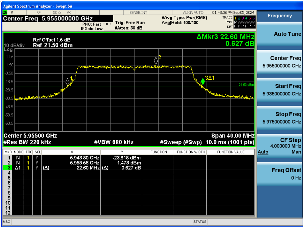
11AX20SISO-Ant1-5955
