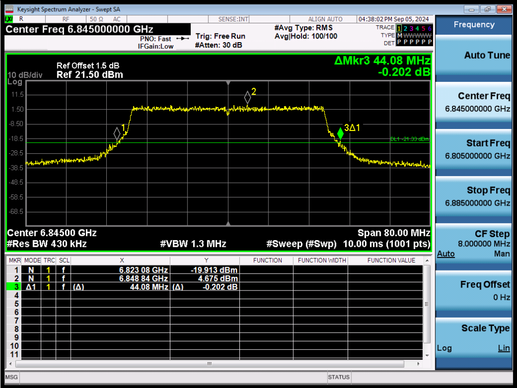
11AX40SISO-Ant1-6845
