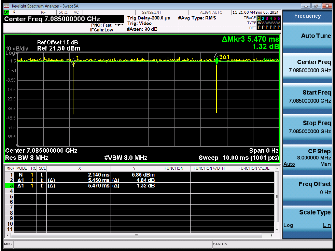
NTNV-11BE40SISO-Ant1-7085
