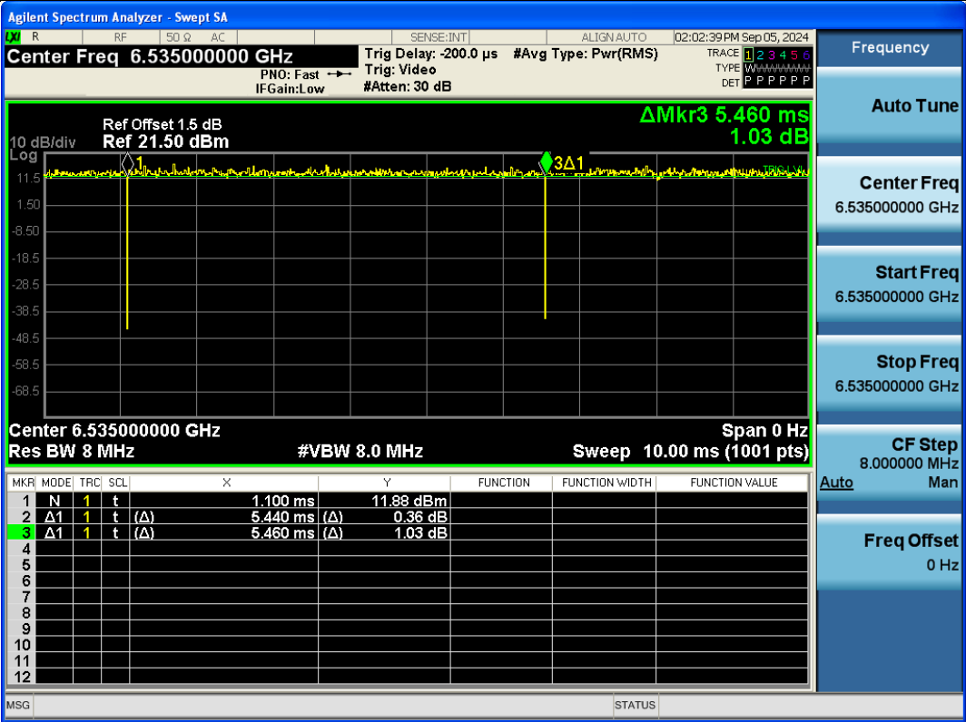
NTNV-11AX20SISO-Ant1-6535
