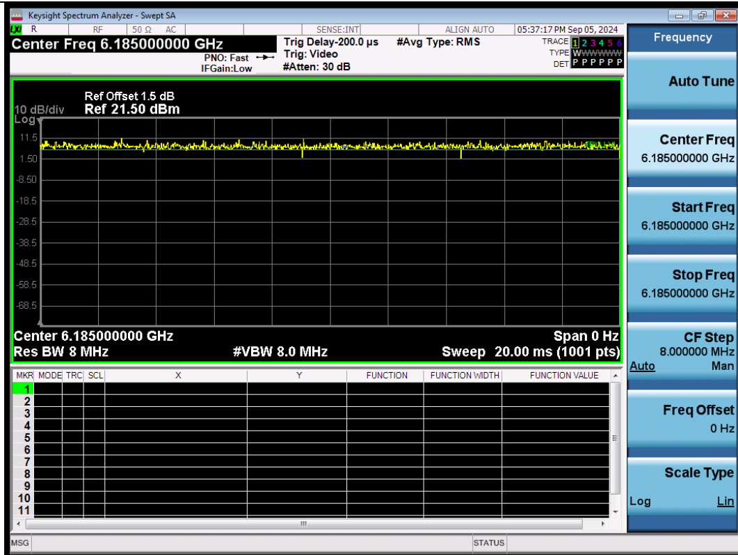
NTNV-11AX160SISO-Ant1-6185
