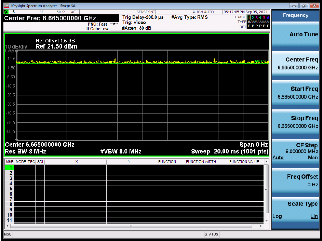
NTNV-11AX160SISO-Ant1-6665
