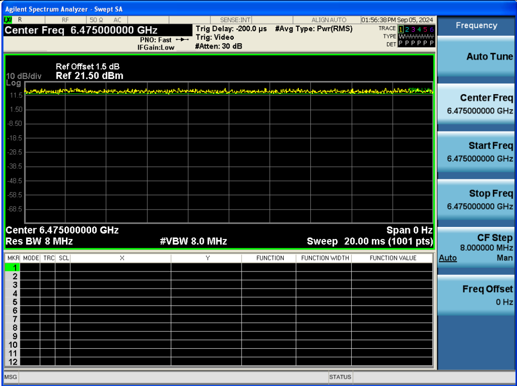
NTNV-11AX20SISO-Ant1-6475
