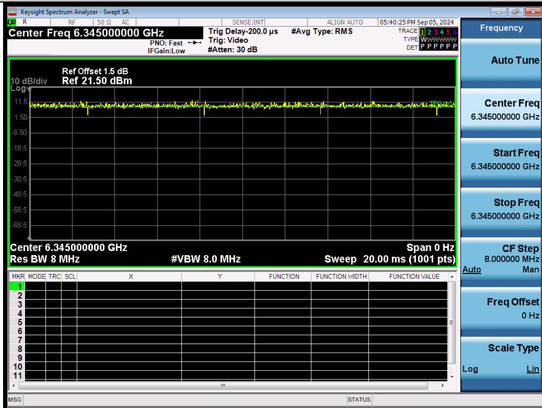
NTNV-11AX160SISO-Ant1-6345
