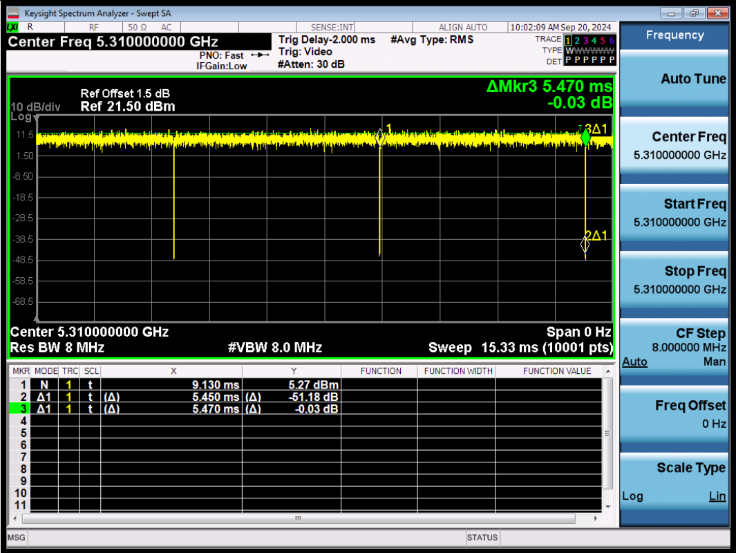
NTNV-11BE40SISO-Ant1-5310
