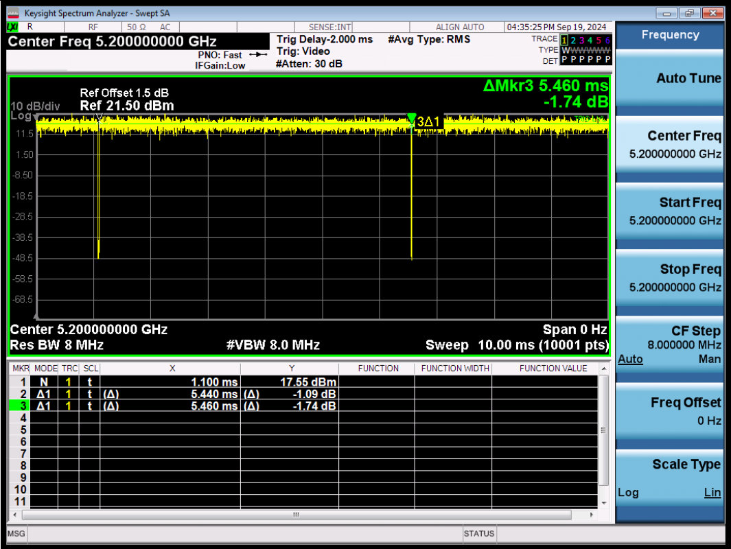
NTNV-11AX20SISO-Ant1-5200
