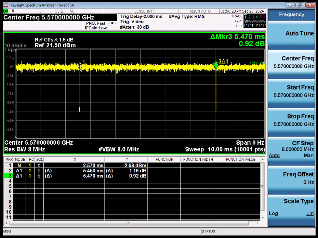
NTNV-11BE160SISO-Ant1-5570
