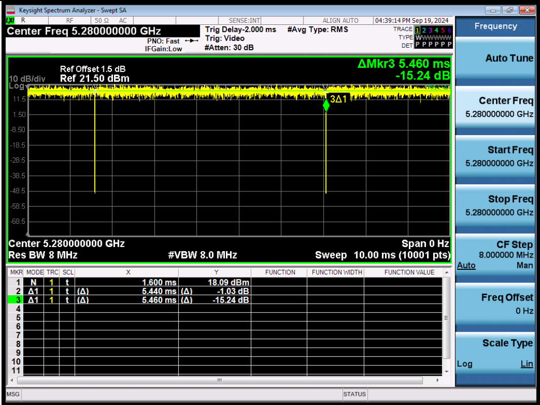
NTNV-11AX20SISO-Ant1-5280
