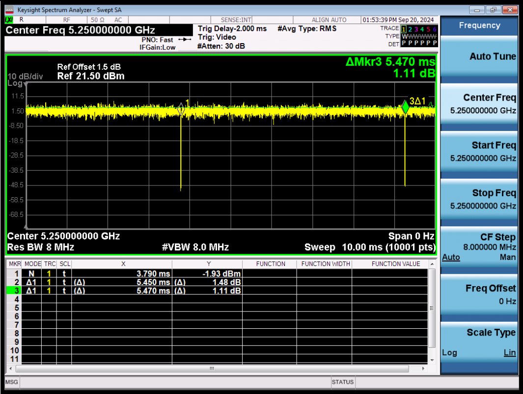
NTNV-11BE160SISO-Ant1-5250
