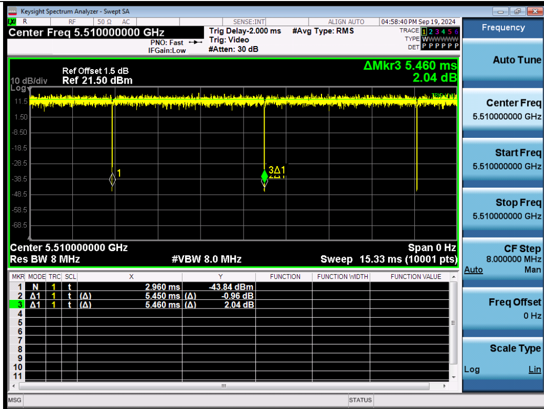
NTNV-11AX40SISO-Ant1-5510
