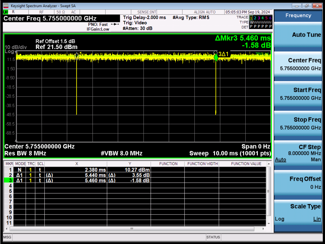
NTNV-11AX40SISO-Ant1-5755
