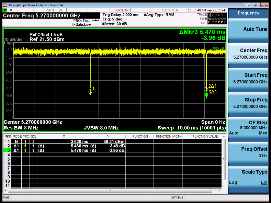
NTNV-11BE40SISO-Ant1-5270
