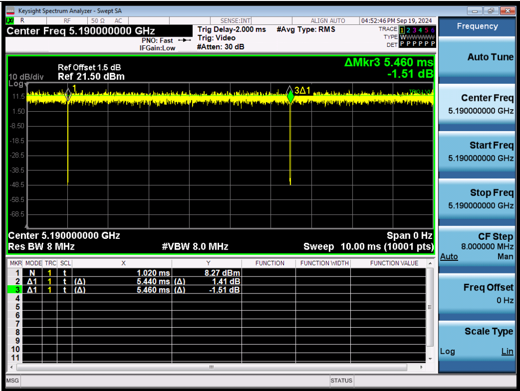
NTNV-11AX40SISO-Ant1-5190
