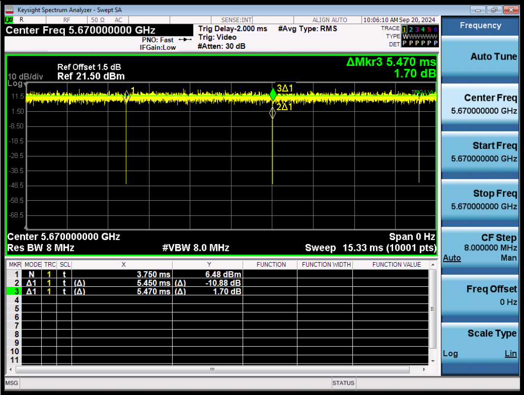
NTNV-11BE40SISO-Ant1-5670
