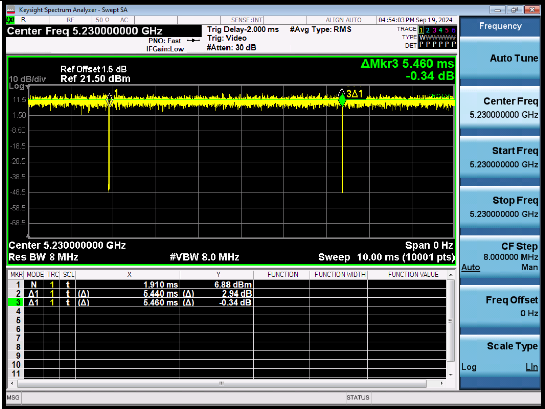
NTNV-11AX40SISO-Ant1-5230
