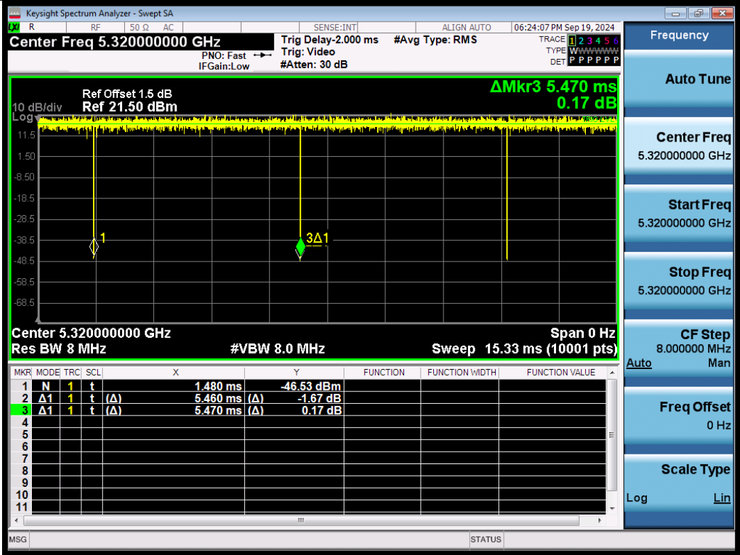
NTNV-11BE20SISO-Ant1-5320
