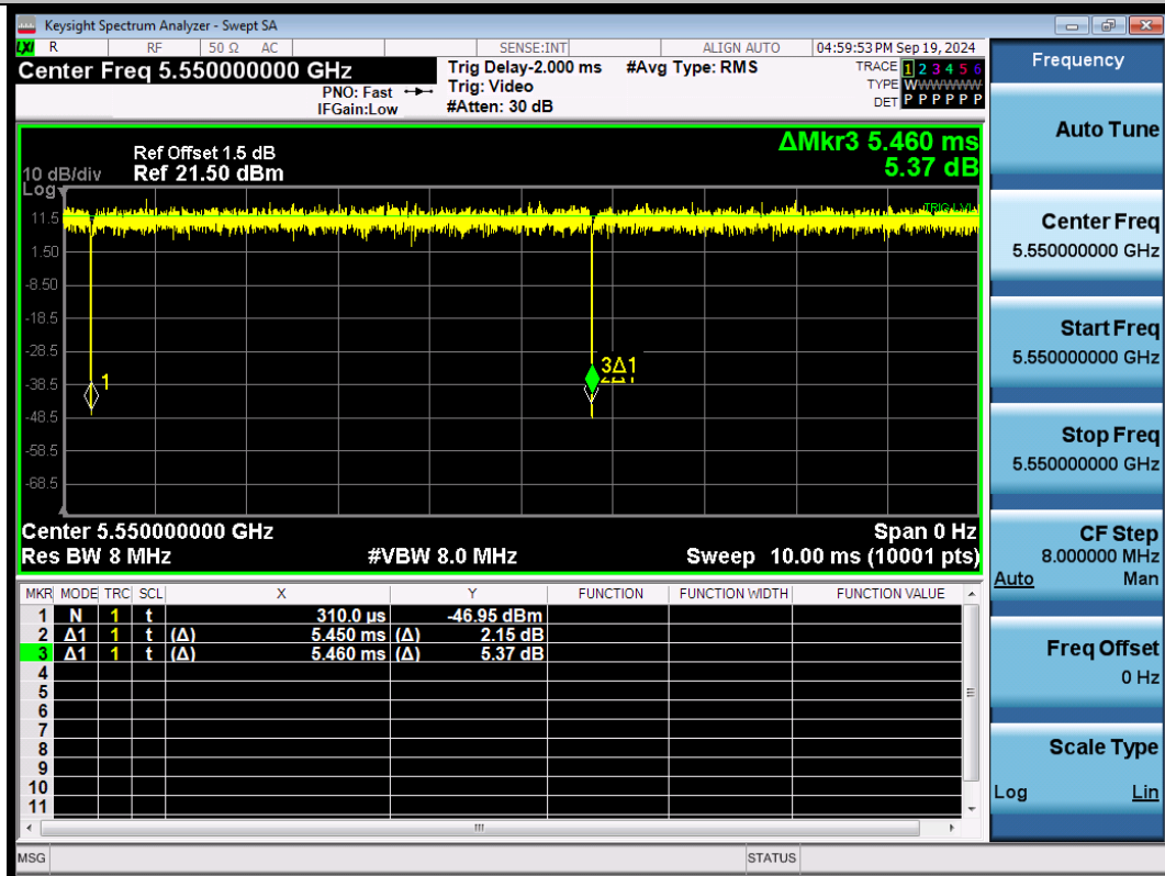
NTNV-11AX40SISO-Ant1-5550
