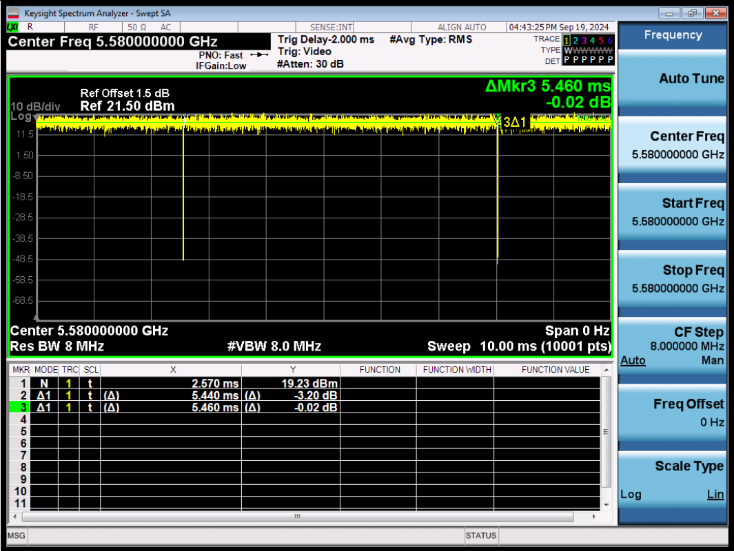
NTNV-11AX20SISO-Ant1-5580
