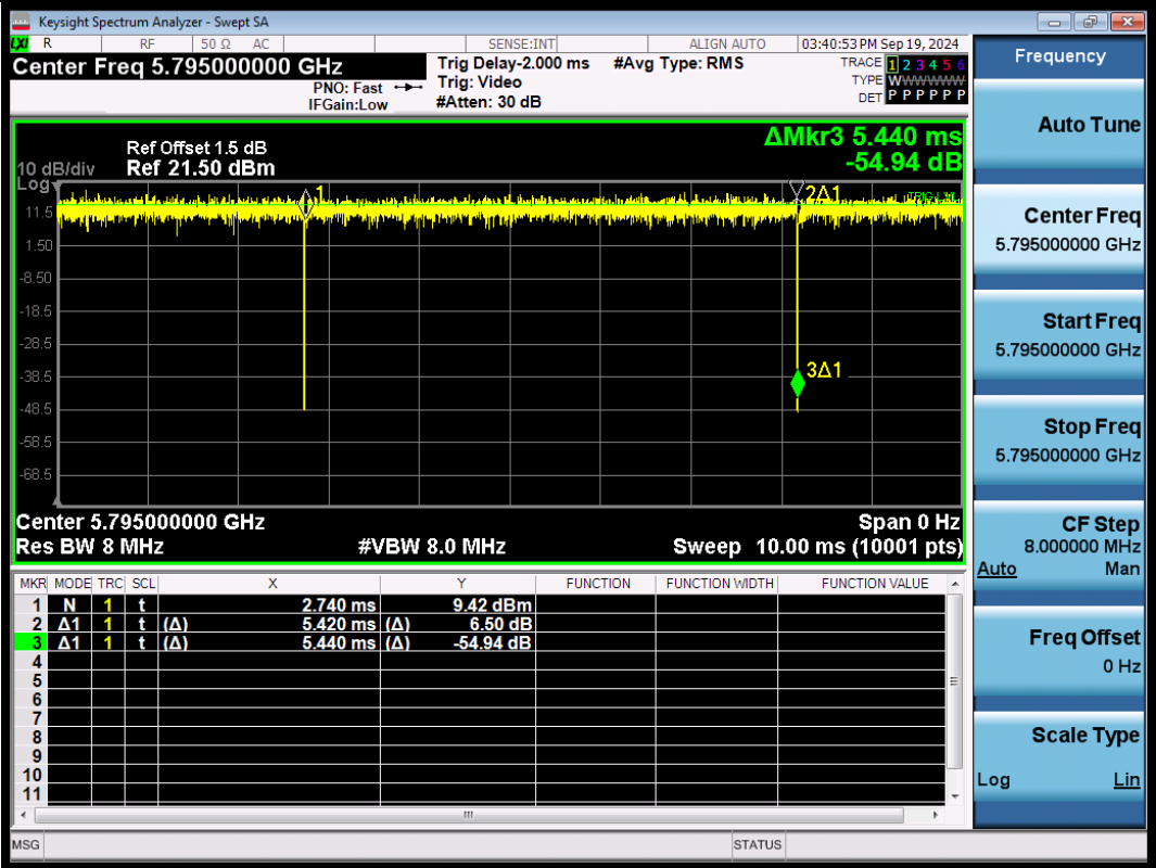
NTNV-11AC40SISO-Ant1-5795
