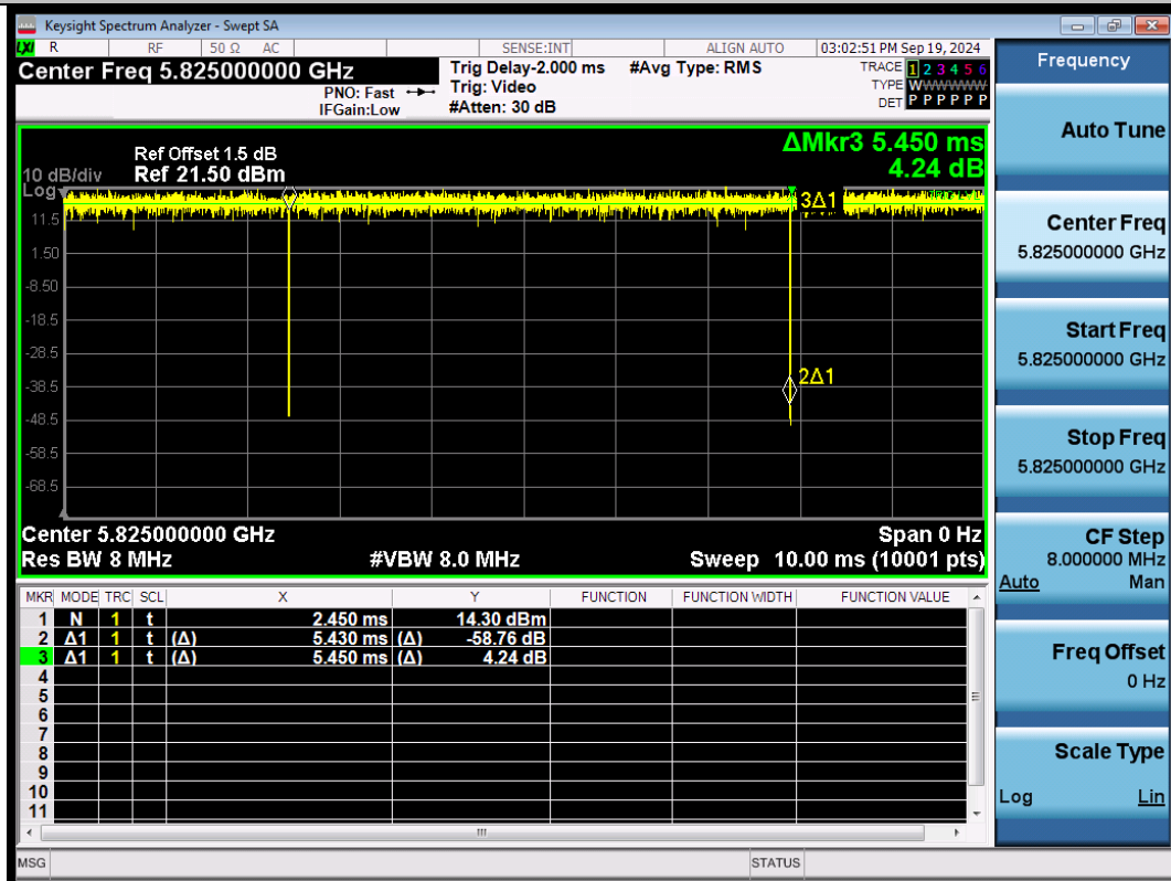
NTNV-11AC20SISO-Ant1-5825
