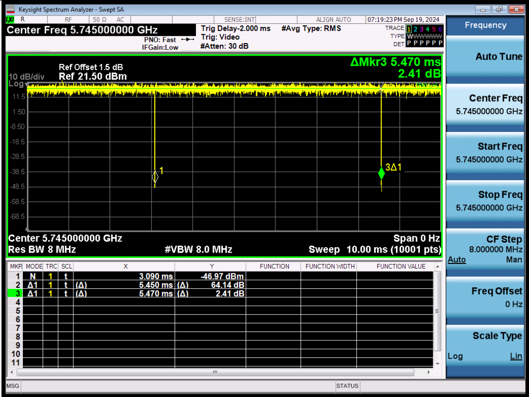
NTNV-11BE20SISO-Ant1-5745
