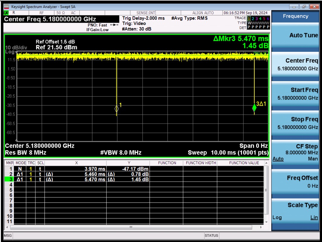
NTNV-11BE20SISO-Ant1-5180
