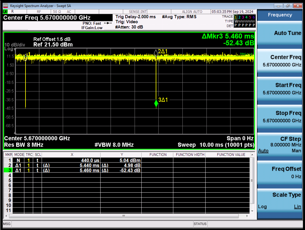
NTNV-11AX40SISO-Ant1-5670
