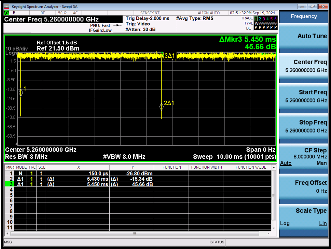
NTNV-11AC20SISO-Ant1-5260
