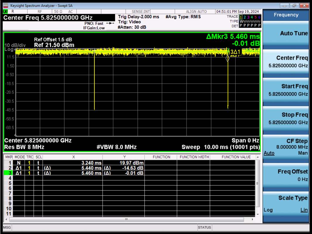
NTNV-11AX20SISO-Ant1-5825
