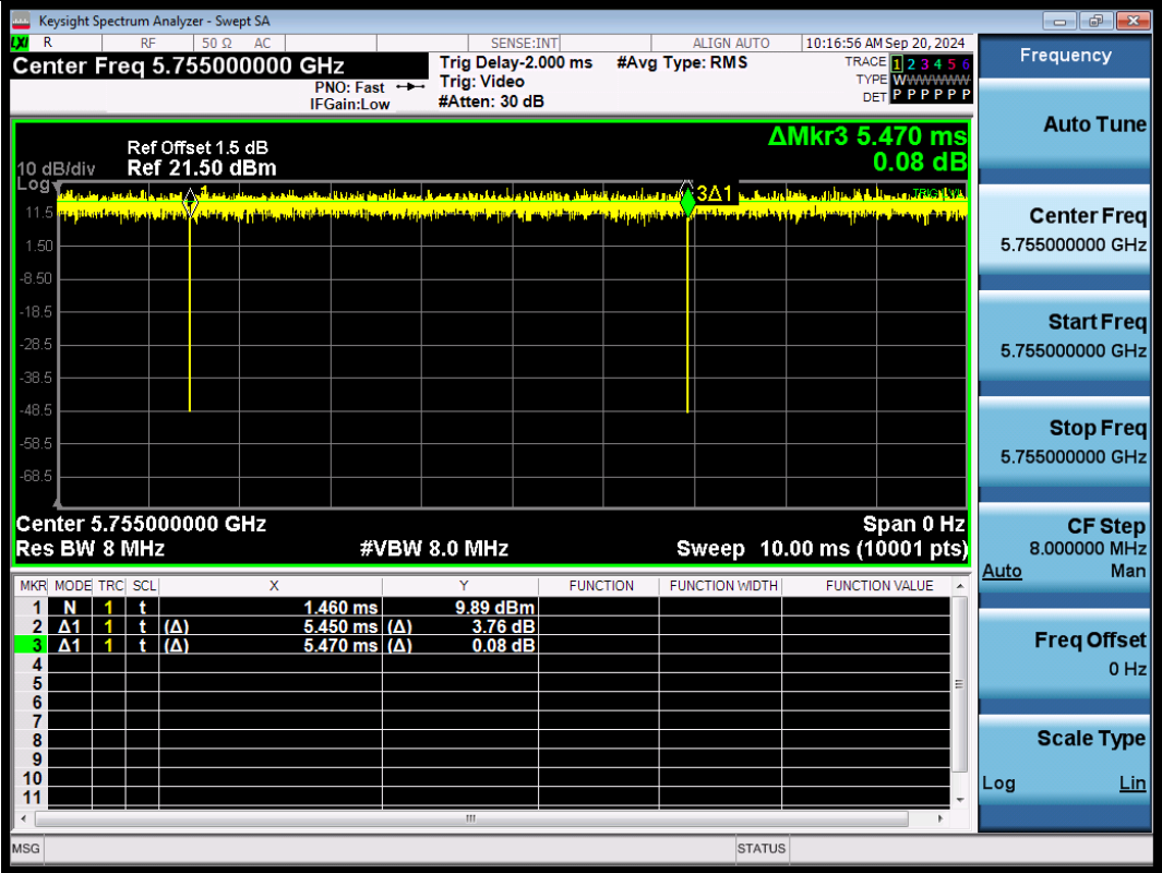
NTNV-11BE40SISO-Ant1-5755
