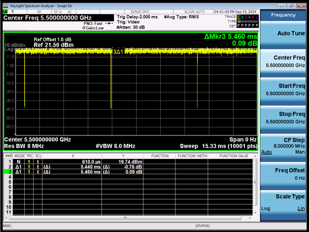
NTNV-11AX20SISO-Ant1-5500
