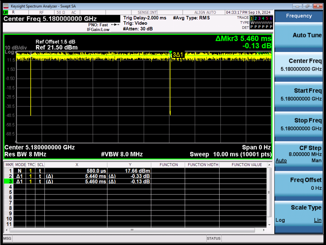
NTNV-11AX20SISO-Ant1-5180
