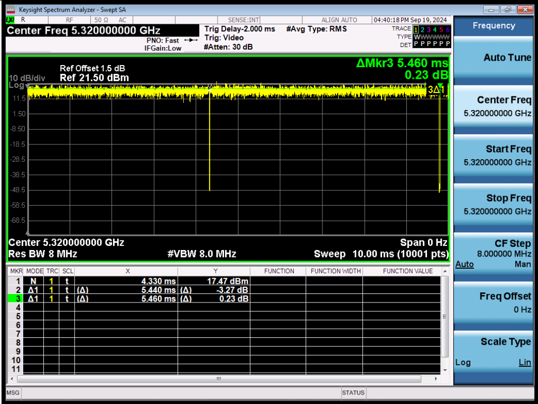
NTNV-11AX20SISO-Ant1-5320
