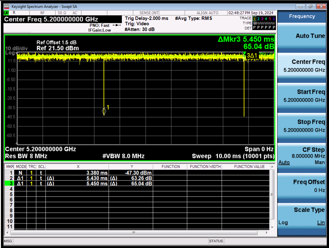
NTNV-11AC20SISO-Ant1-5200
