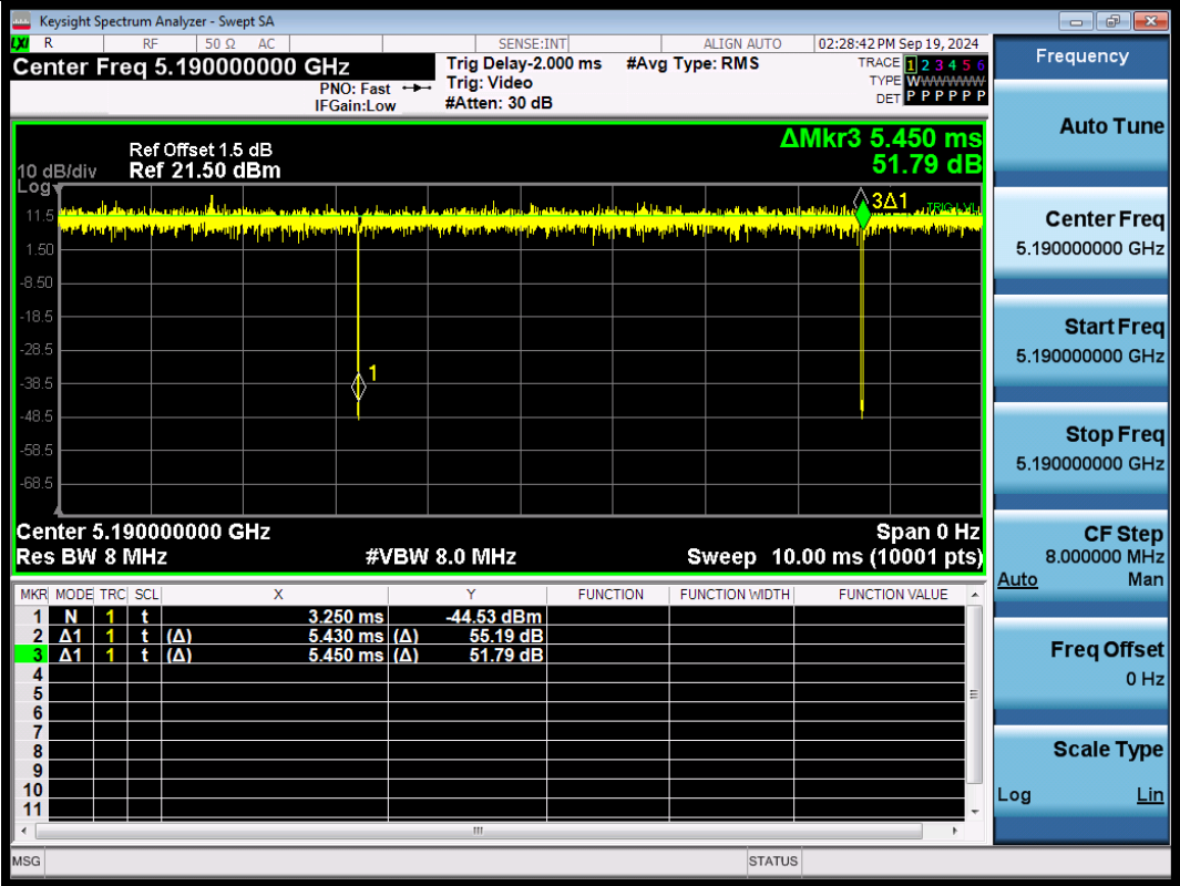
NTNV-11N40SISO-Ant1-5190
