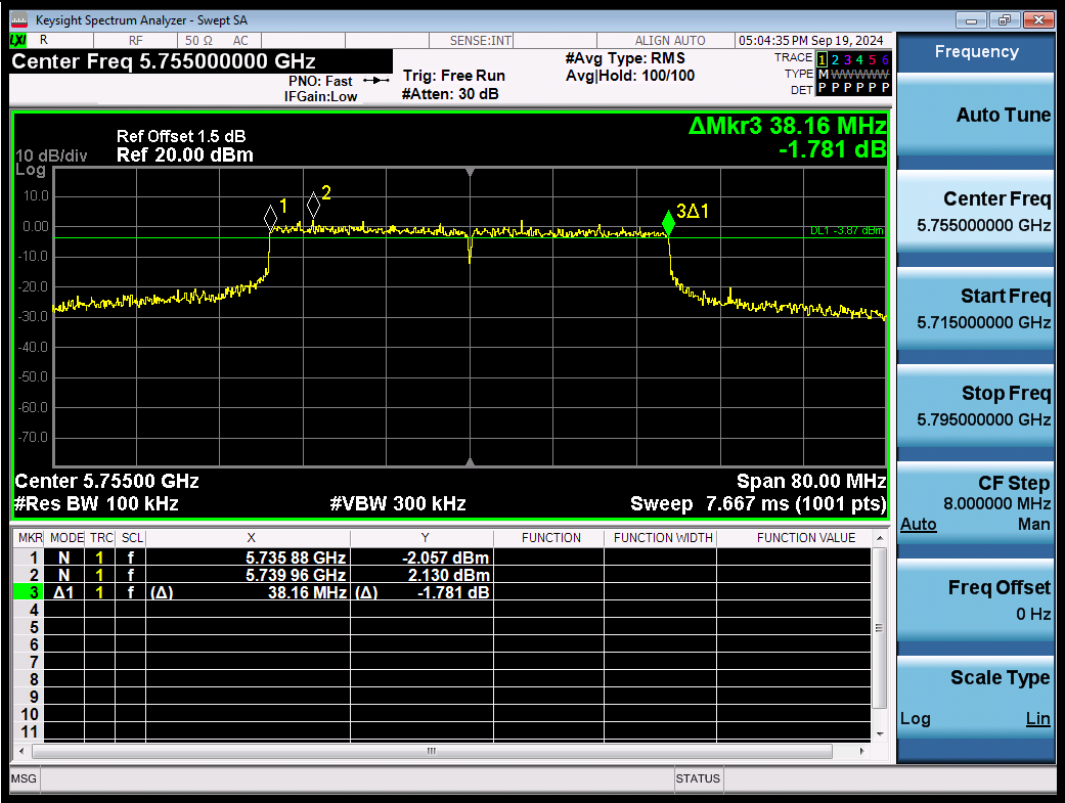
11AX40SISO-Ant1-5755-PASS
