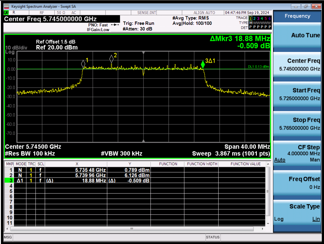
11AX20SISO-Ant1-5745-PASS
