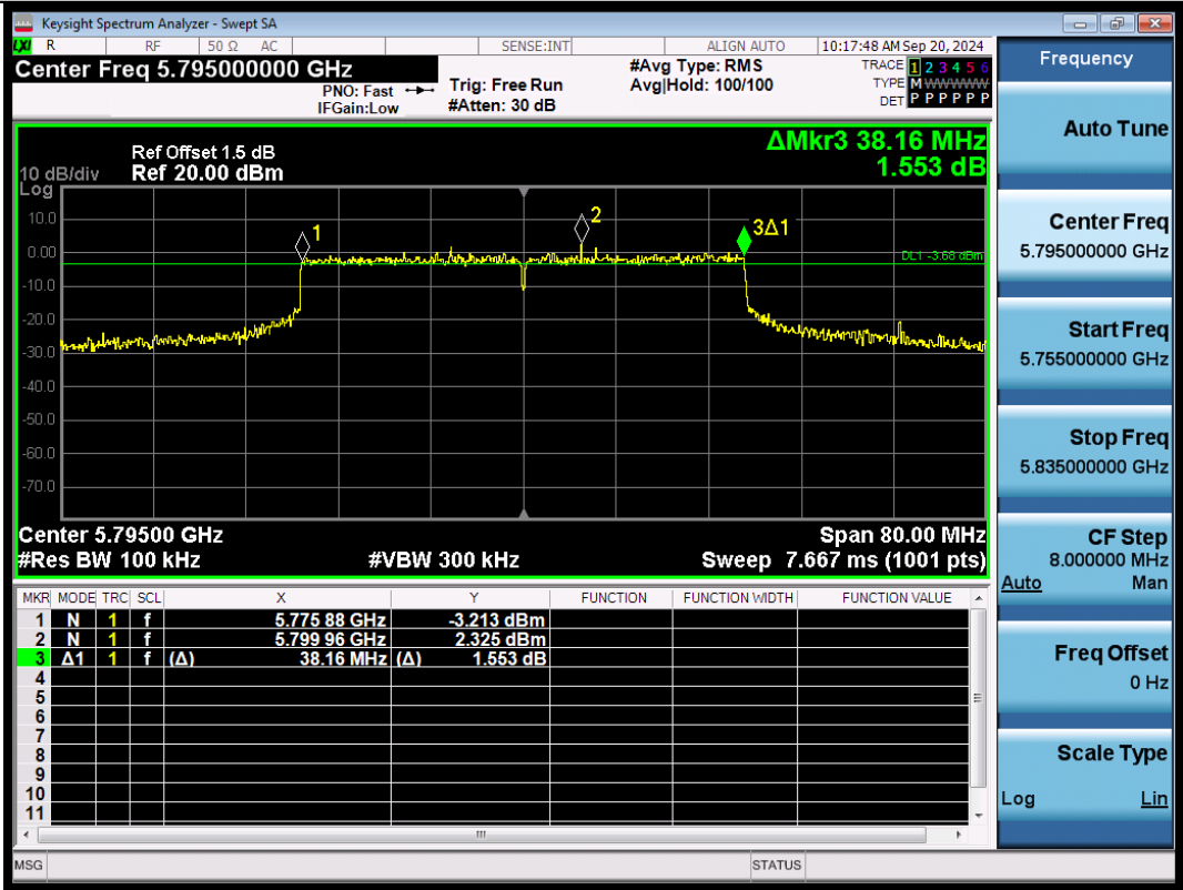
11BE40SISO-Ant1-5795-PASS
