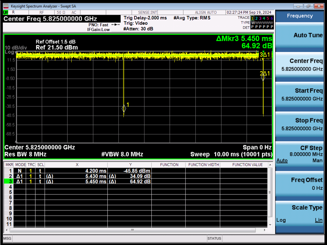
NTNV-11N20SISO-Ant1-5825
