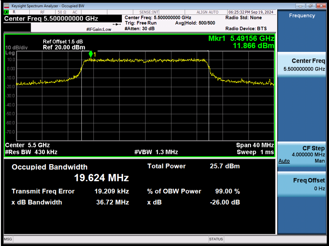
11BE20SISO-Ant1-5500
