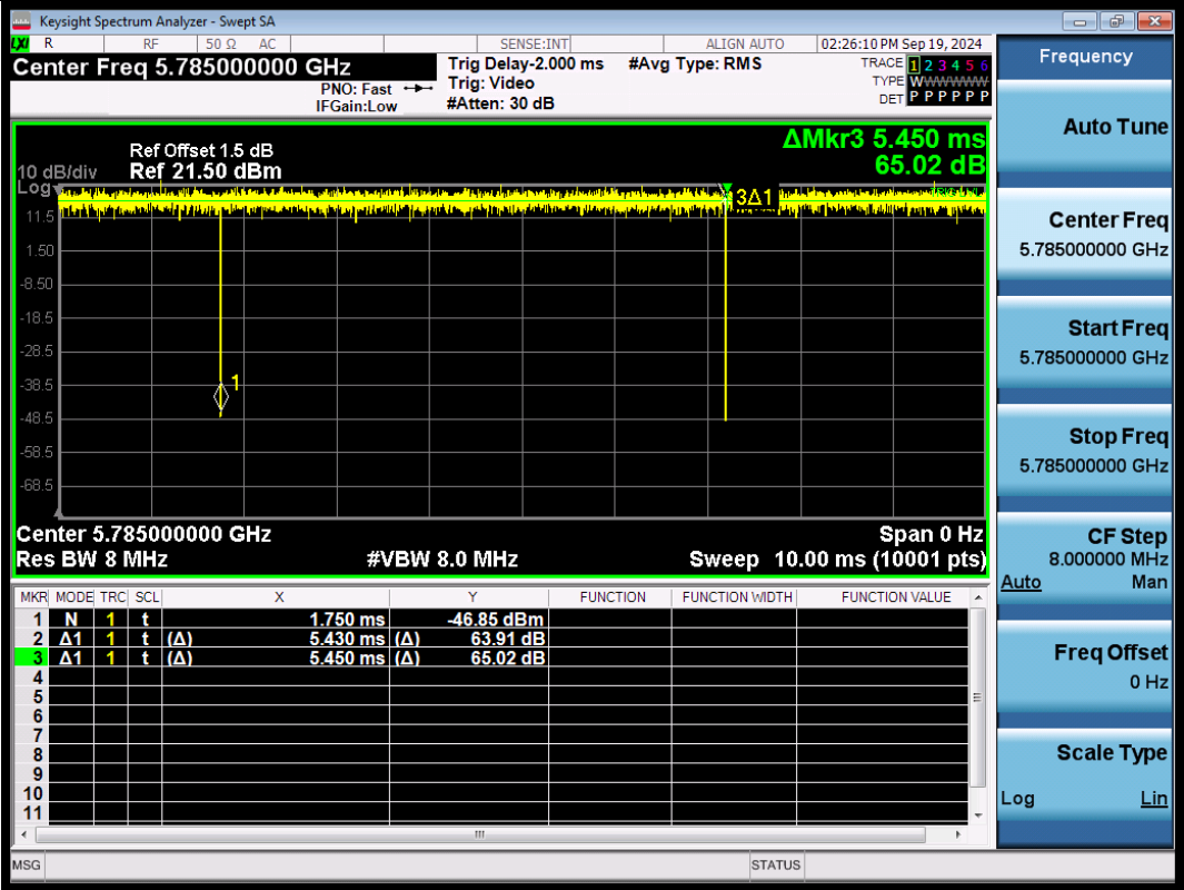
NTNV-11N20SISO-Ant1-5785
