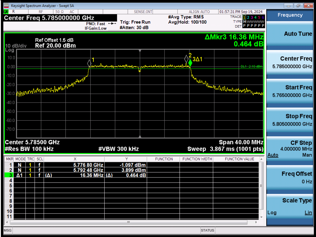
11A-Ant1-5785-PASS
