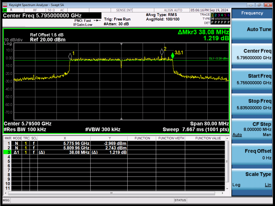
11AX40SISO-Ant1-5795-PASS
