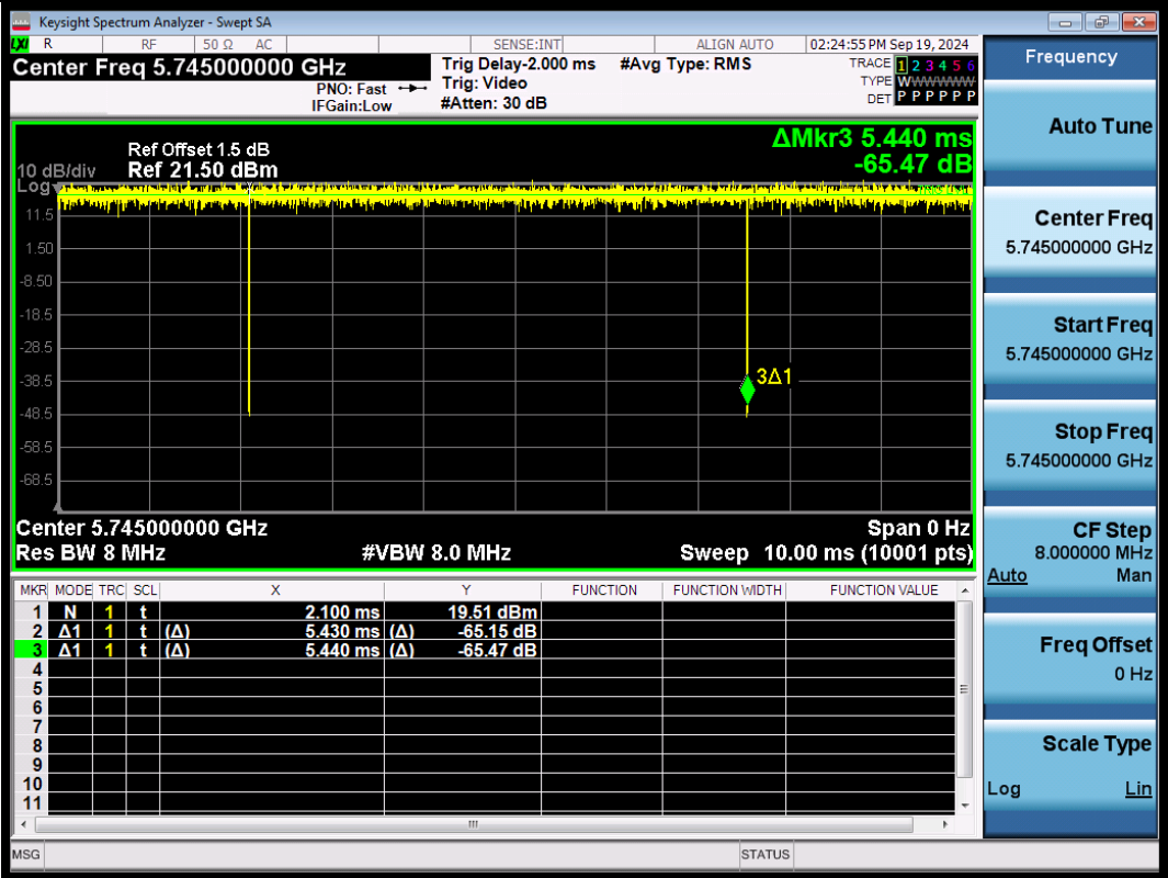
NTNV-11N20SISO-Ant1-5745
