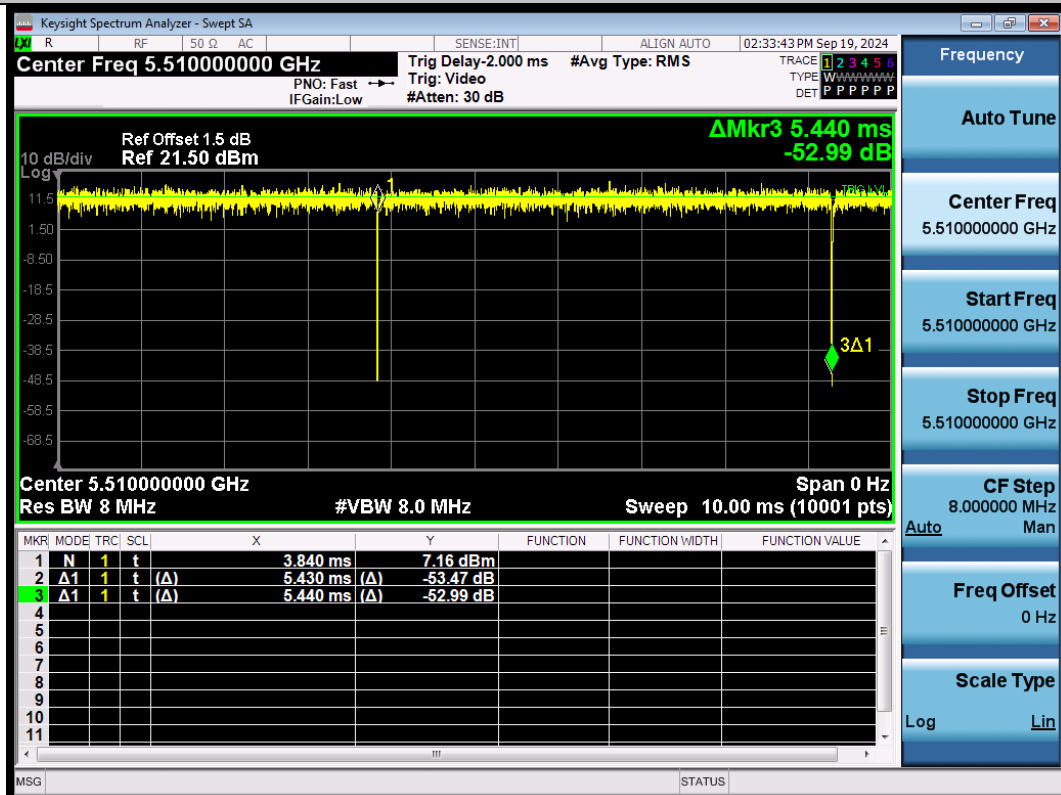
NTNV-11N40SISO-Ant1-5510
