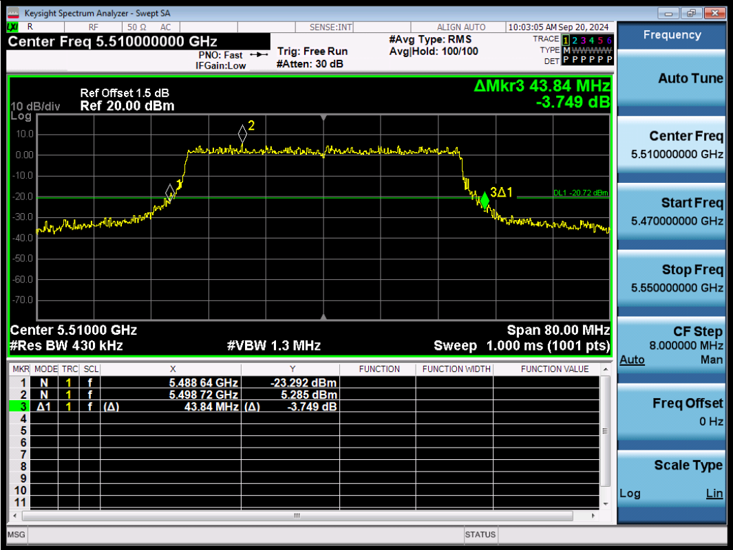
11BE40SISO-Ant1-5510
