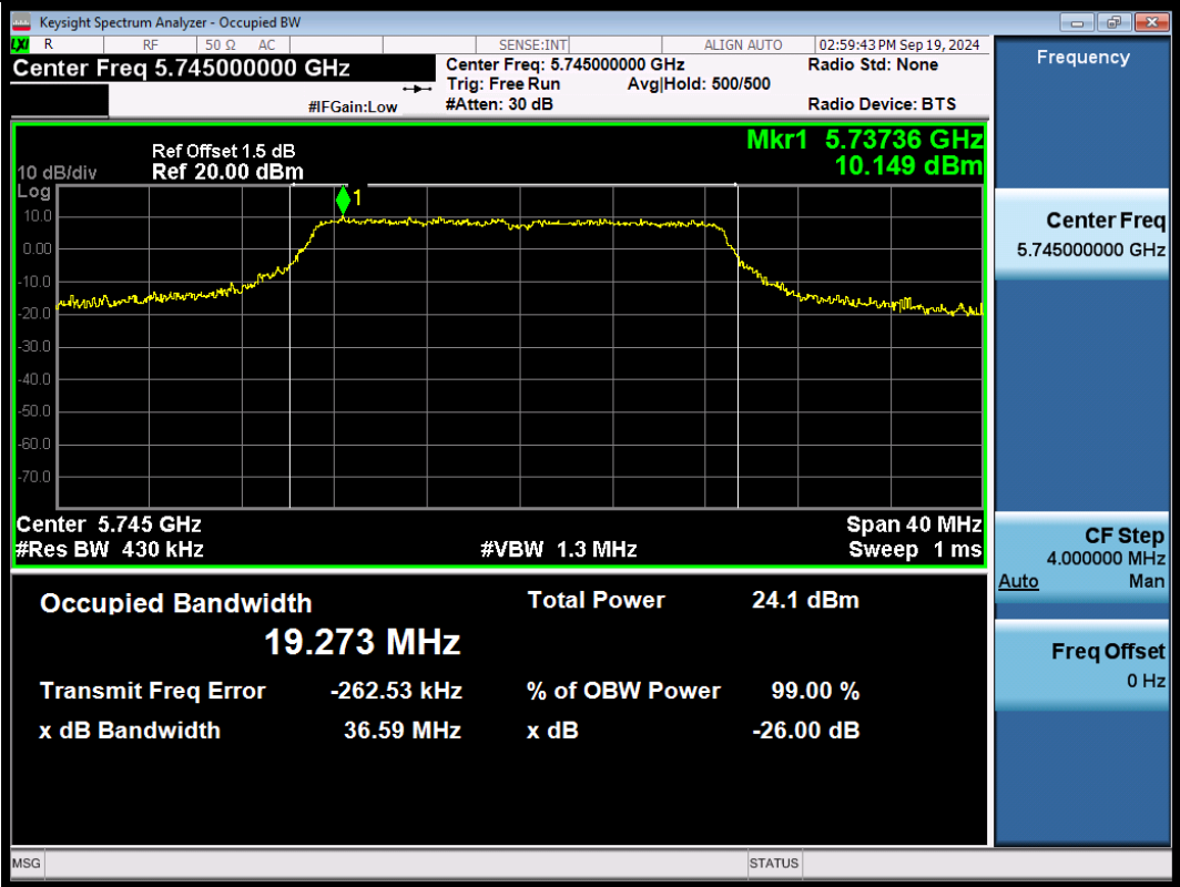
11AC20SISO-Ant1-5745
