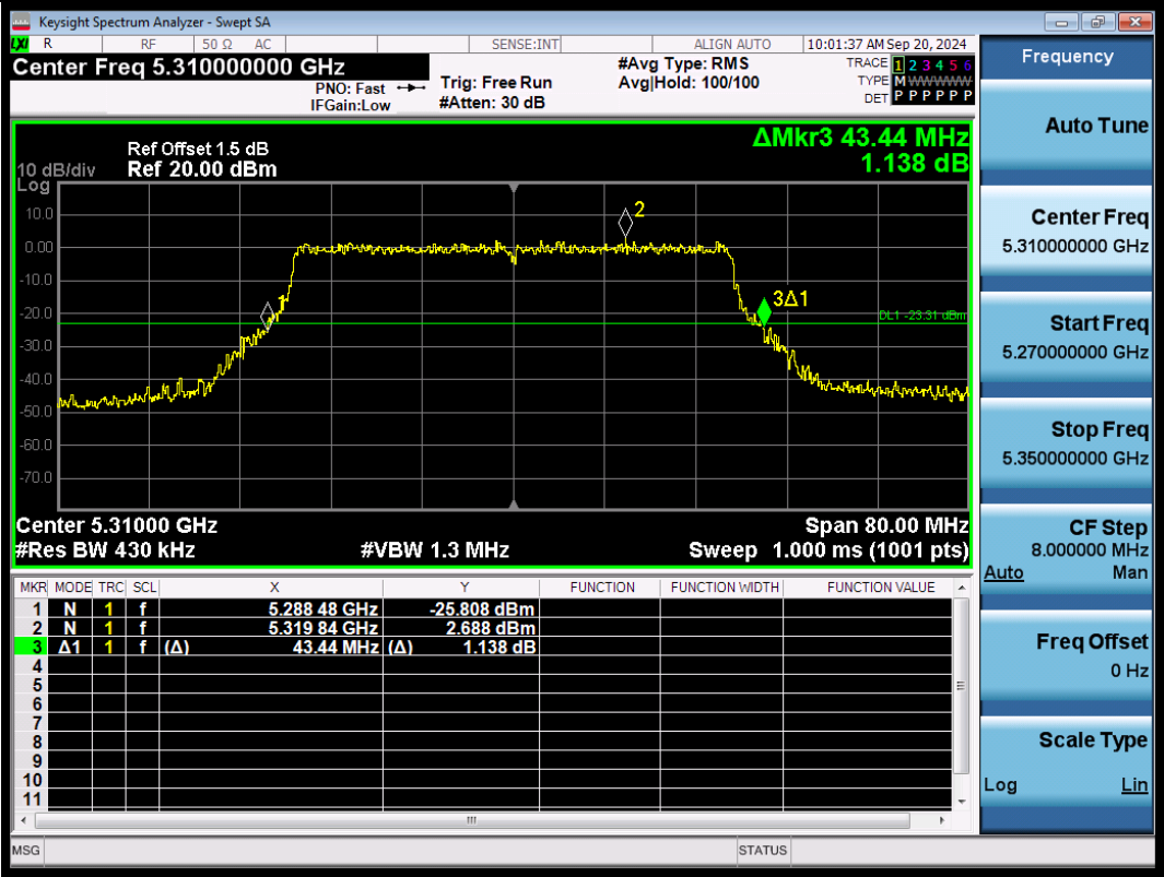
11BE40SISO-Ant1-5310
