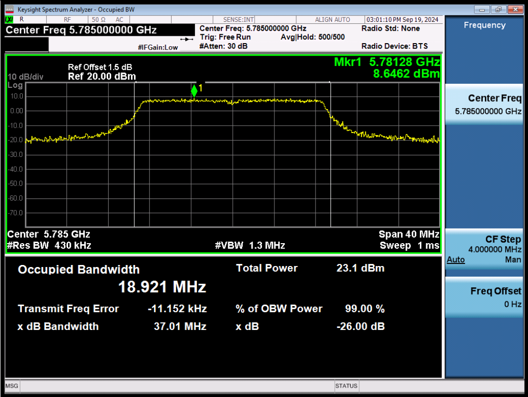
11AC20SISO-Ant1-5785
