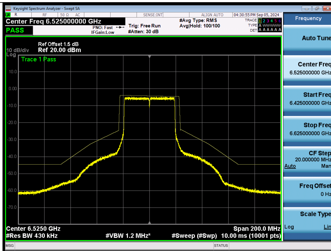
NTNV-11AX40SISO-Ant1-6525-PASS
