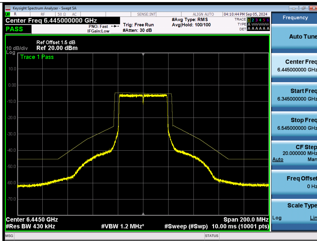
NTNV-11AX40SISO-Ant1-6445-PASS
