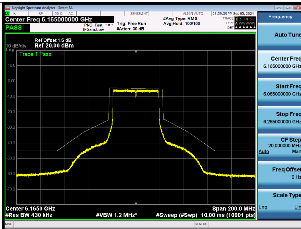
NTNV-11AX40SISO-Ant1-6165-PASS
