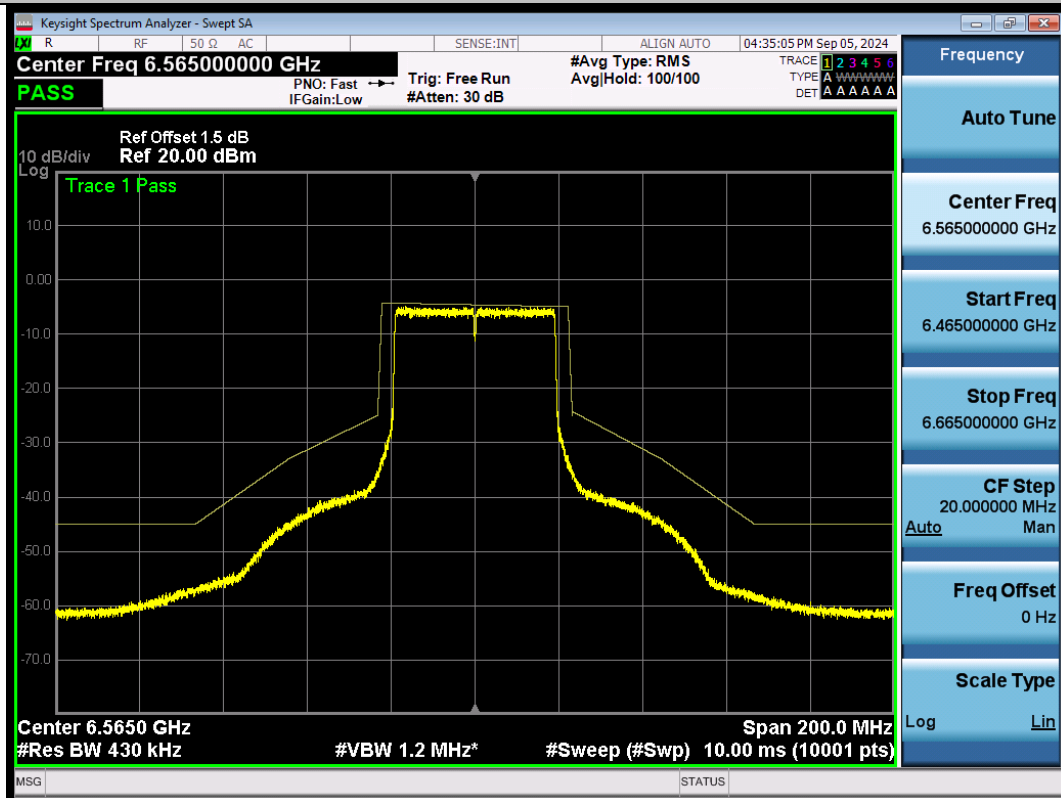
NTNV-11AX40SISO-Ant1-6565-PASS
