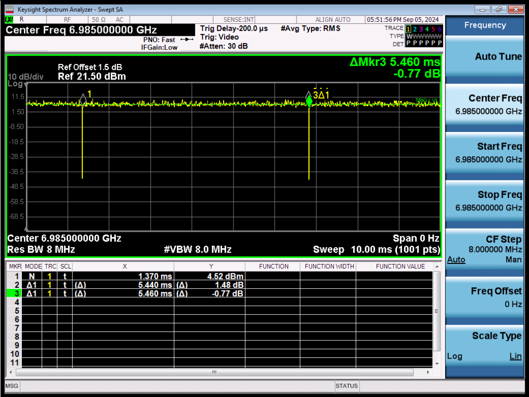
NTNV-11AX160SISO-Ant1-6985
