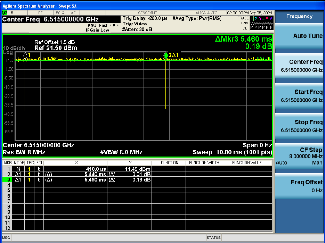
NTNV-11AX20SISO-Ant1-6515
