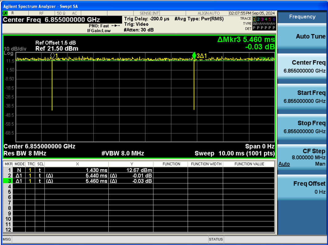
NTNV-11AX20SISO-Ant1-6855
