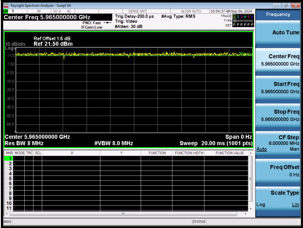
NTNV-11BE40SISO-Ant1-5965
