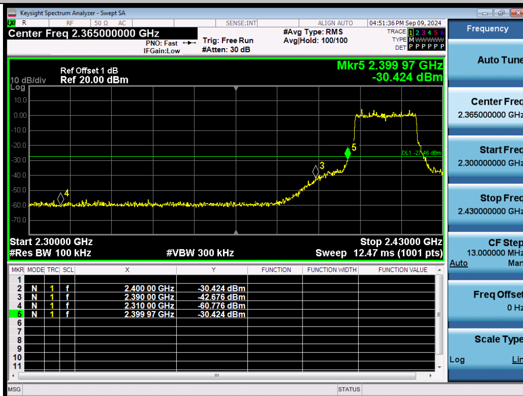
11BE20SISO-Ant1-2412-PASS
