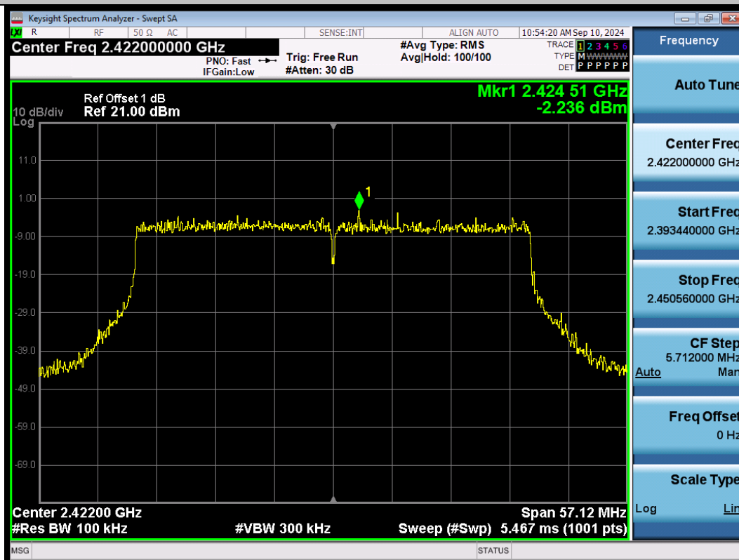
11AX40SISO-Ant1-2422-PASS
