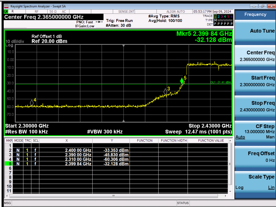
11BE40SISO-Ant1-2422-PASS
