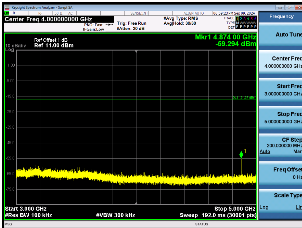
11B-Ant1-2437-3000~5000-PASS
