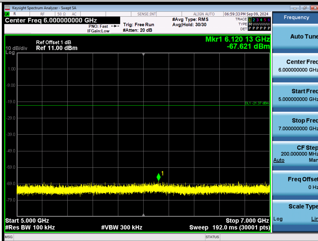
11B-Ant1-2437-5000~7000-PASS
