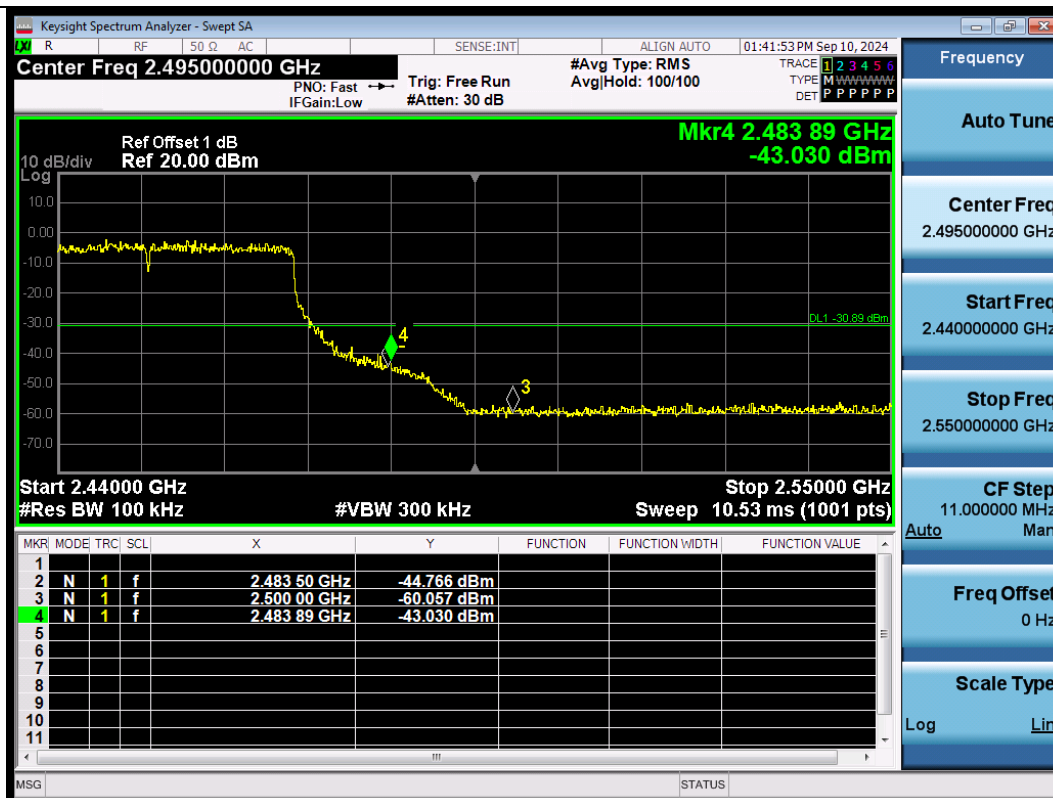
11AX40SISO-Ant1-2452-PASS
