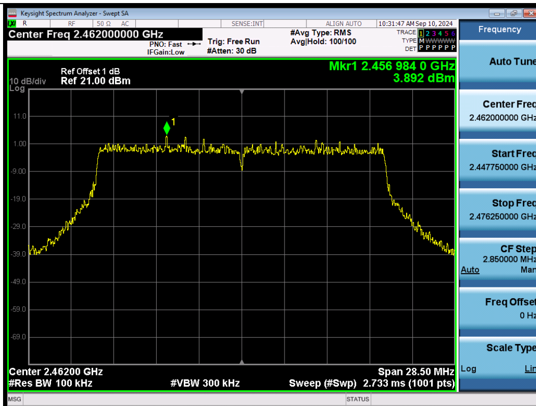
11AX20SISO-Ant1-2462-PASS
