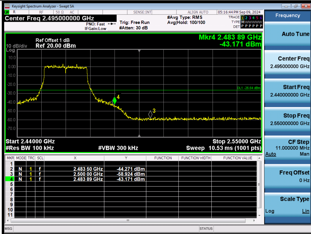
11BE20SISO-Ant1-2462-PASS
