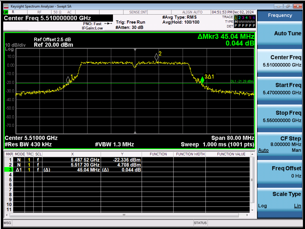
11AC40SISO-Ant3-5510
