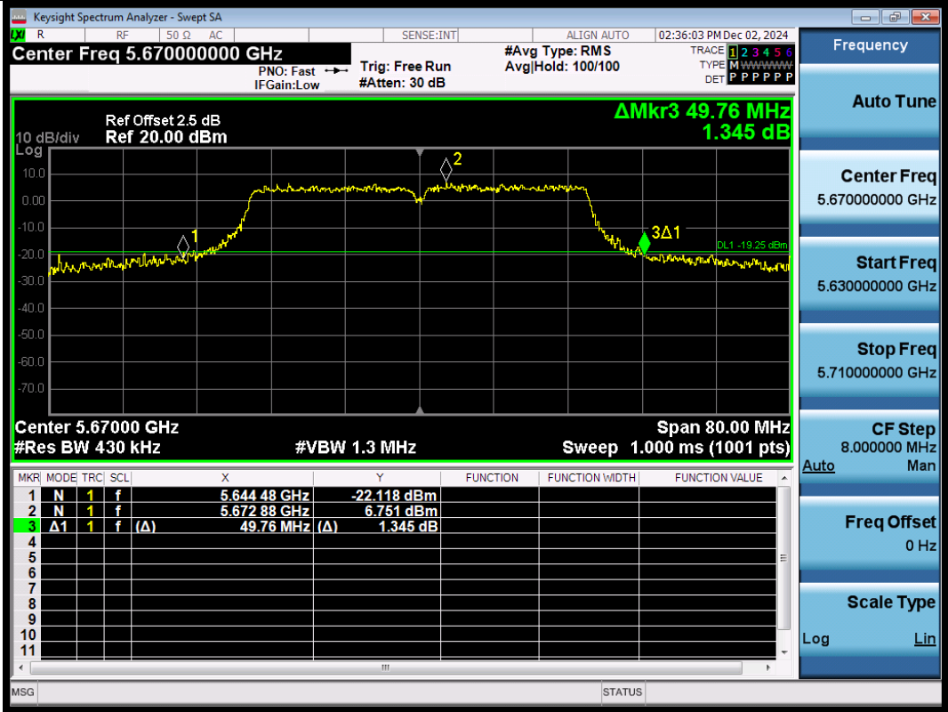
11N40SISO-Ant3-5670
