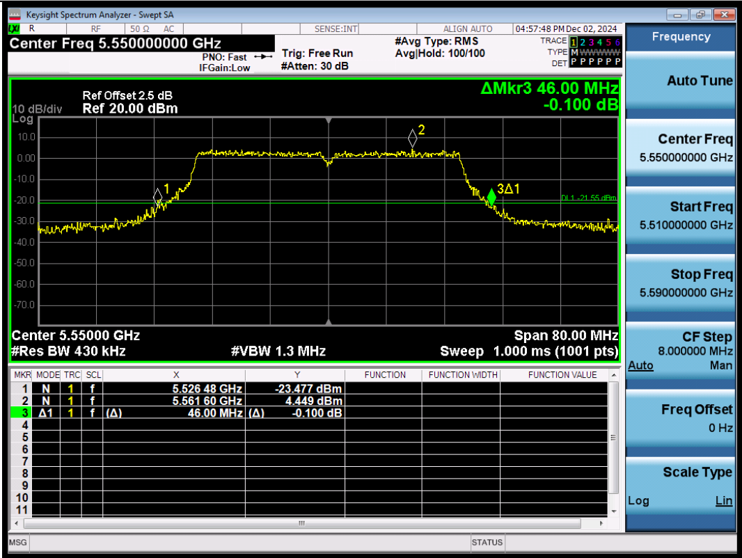
11AC40SISO-Ant3-5550
