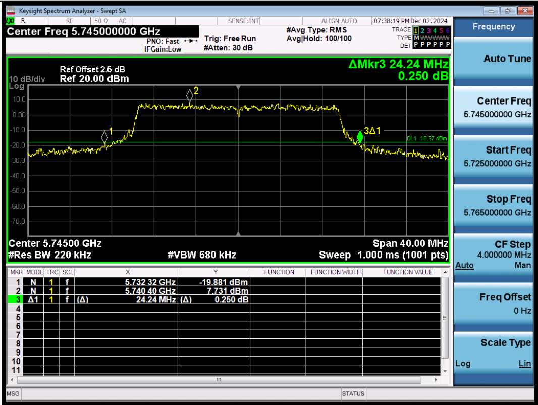
11AX20SISO-Ant3-5745
