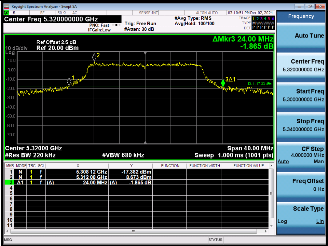
11AC20SISO-Ant3-5320
