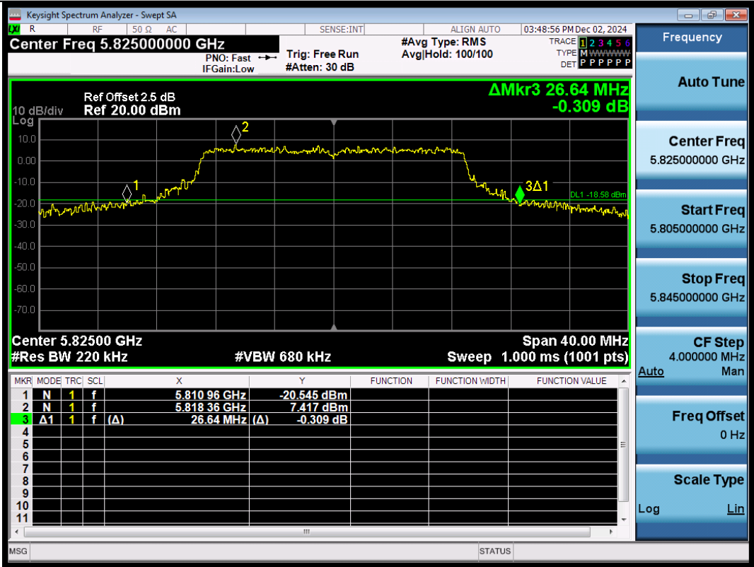
11AC20SISO-Ant3-5825
