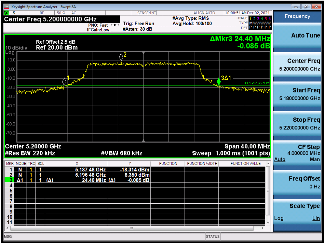
11N20SISO-Ant3-5200
