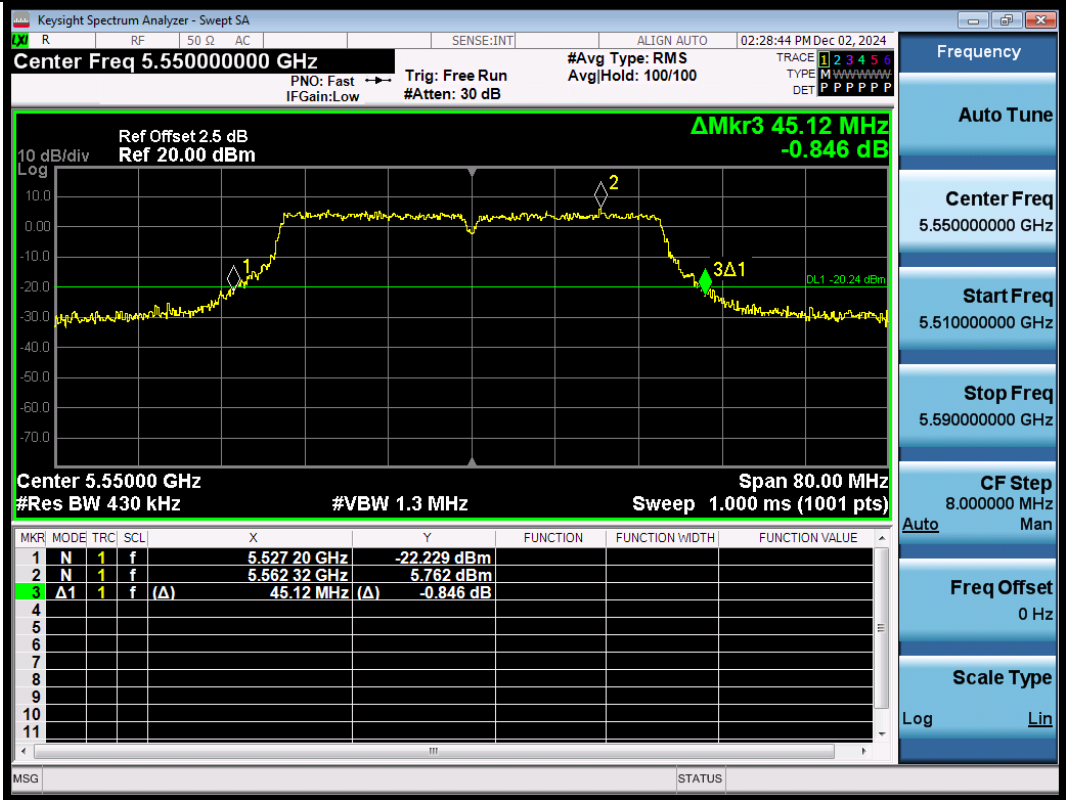
11N40SISO-Ant3-5550
