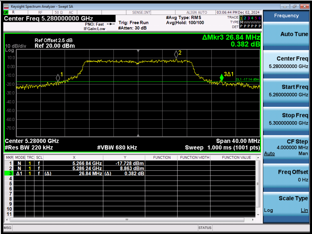
11AC20SISO-Ant3-5280
