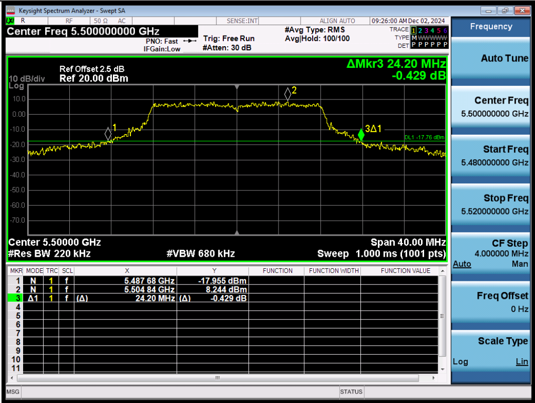
11A-Ant3-5500
