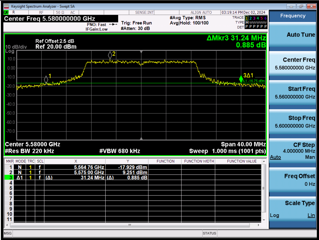
11AC20SISO-Ant3-5580
