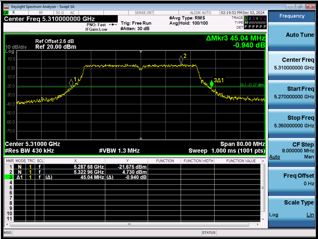
11N40SISO-Ant3-5310
