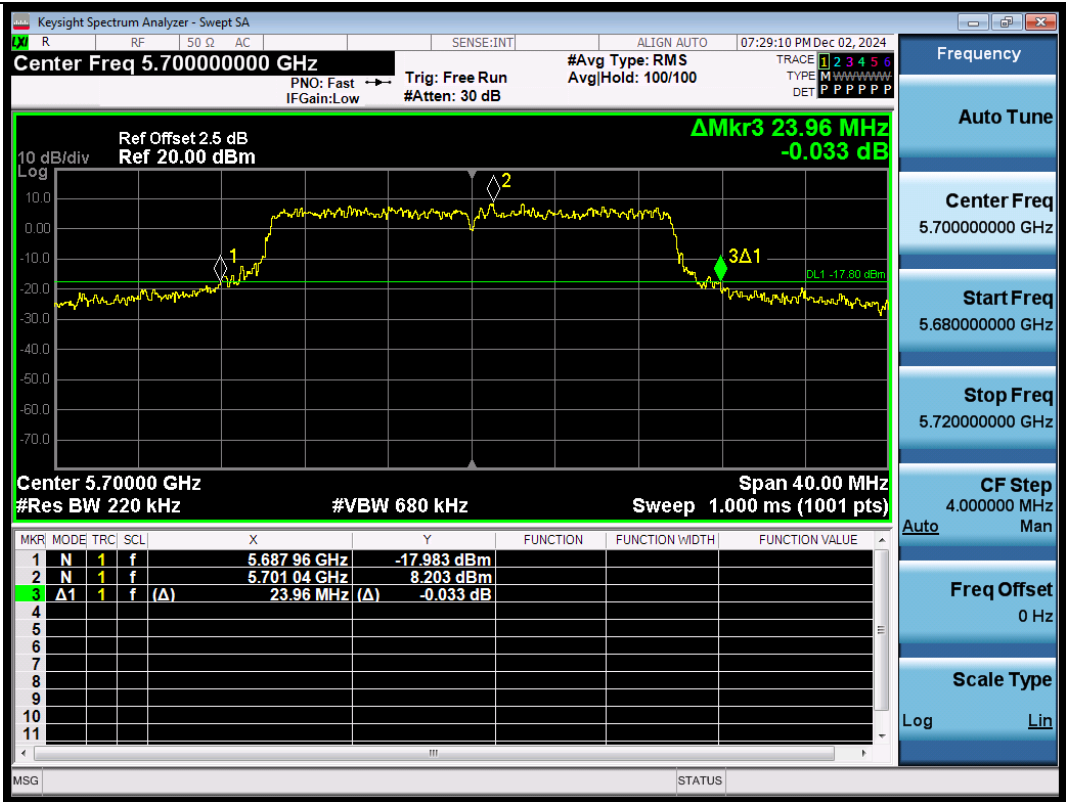
11AX20SISO-Ant3-5700
