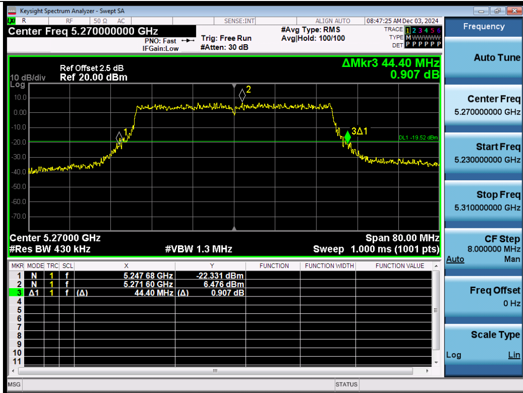
11AX40SISO-Ant3-5270
