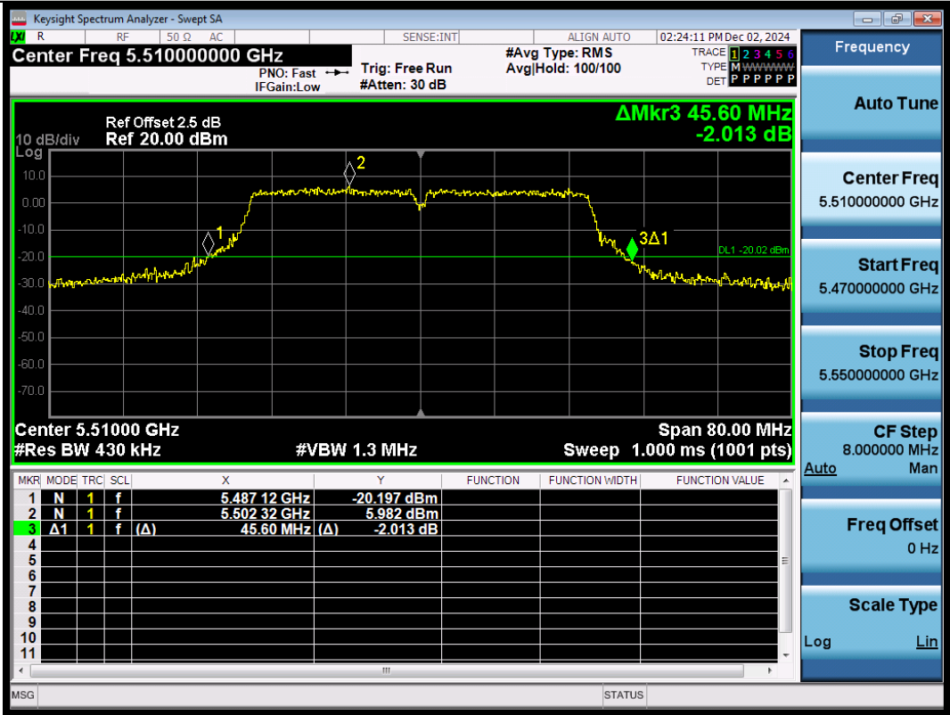
11N40SISO-Ant3-5510
