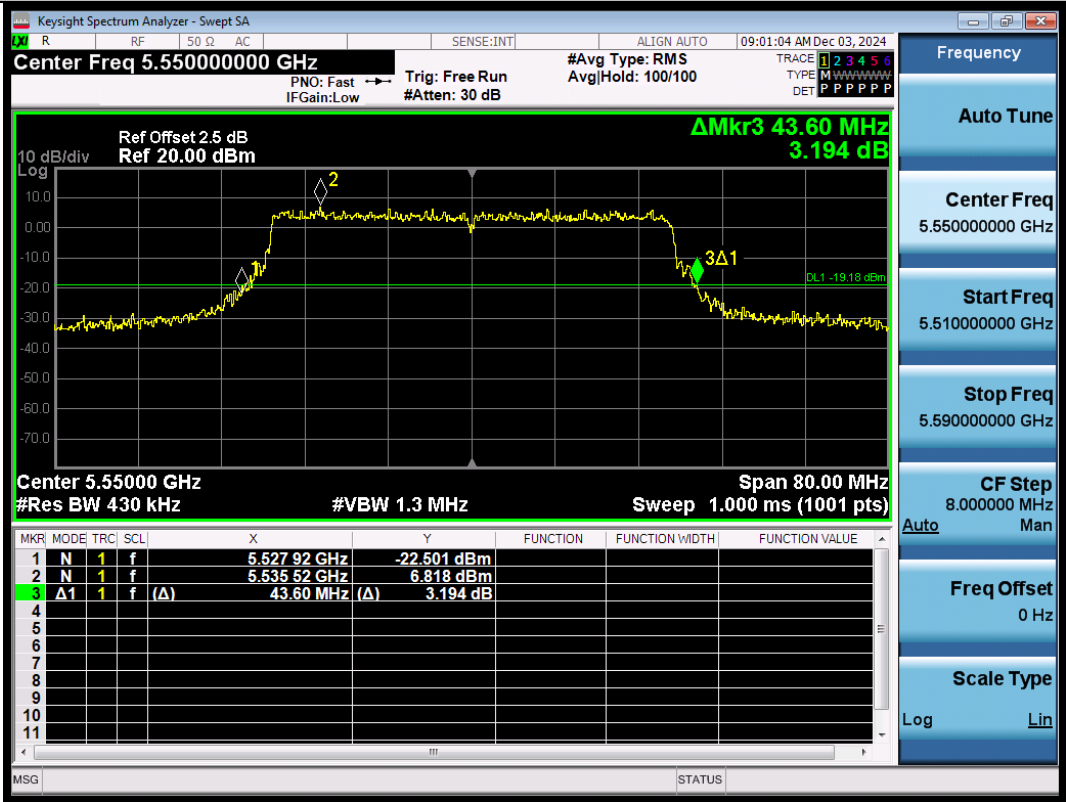
11AX40SISO-Ant3-5550
