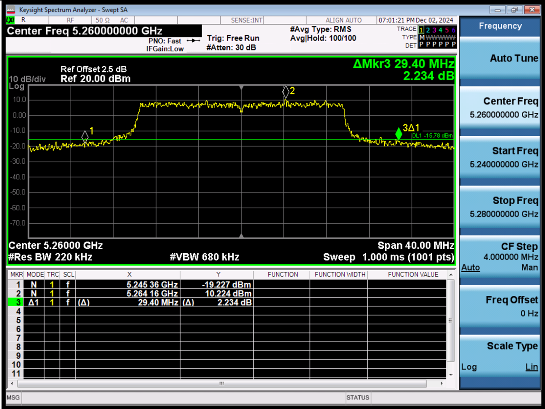
11AX20SISO-Ant3-5260
