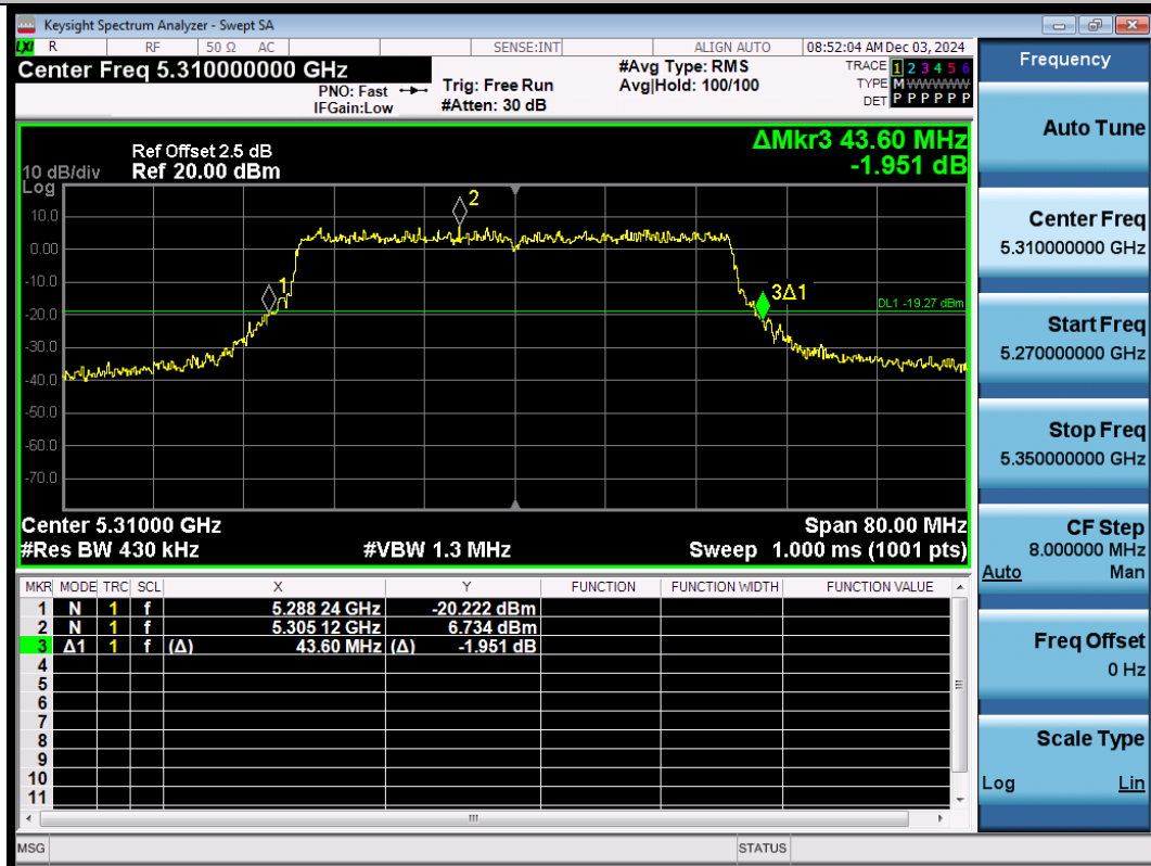
11AX40SISO-Ant3-5310
