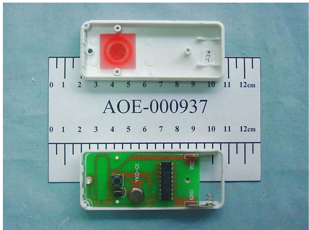
FIGURE 2 RF TIMER CONTROLLER (M/N: 5244341H) COVER REMOVED 2
