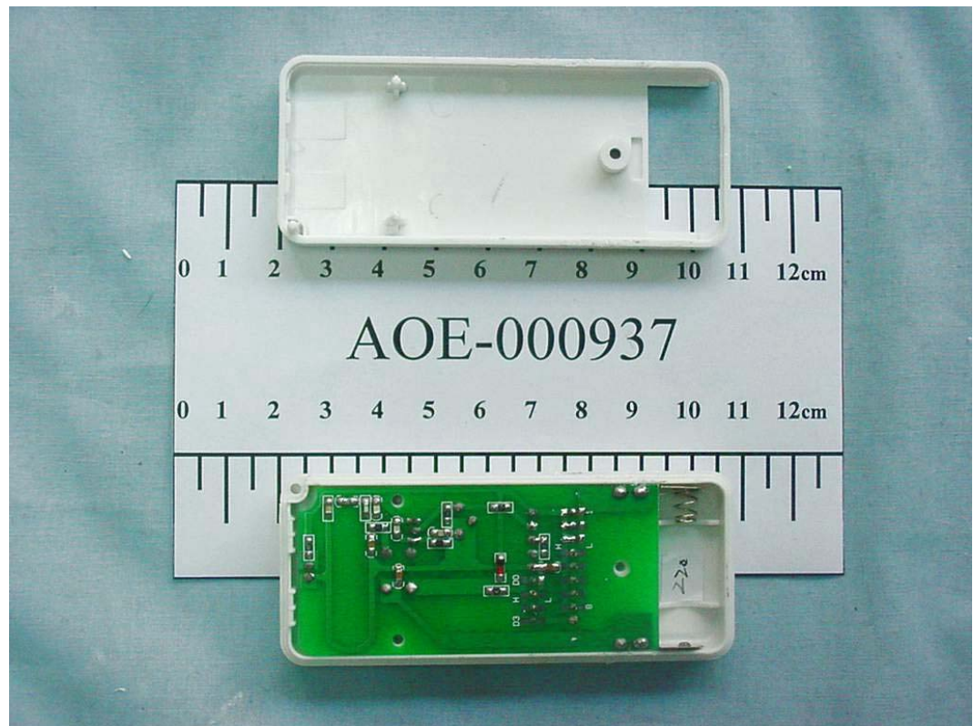
FIGURE 1 RF TIMER CONTROLLER (M/N: 5244341H) COVER REMOVED 1
