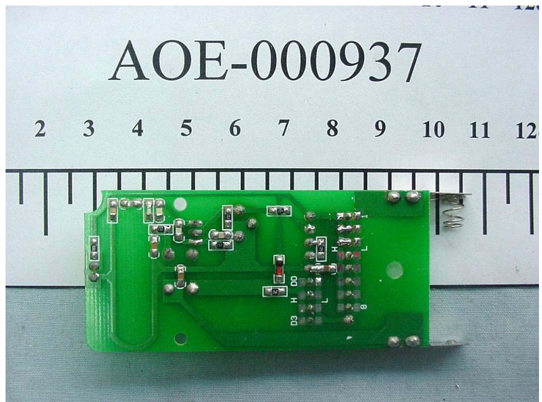
FIGURE 4 RF TIMER CONTROLLER (M/N: 5244341H) MAIN BOARD (SOLDERED SIDE)
