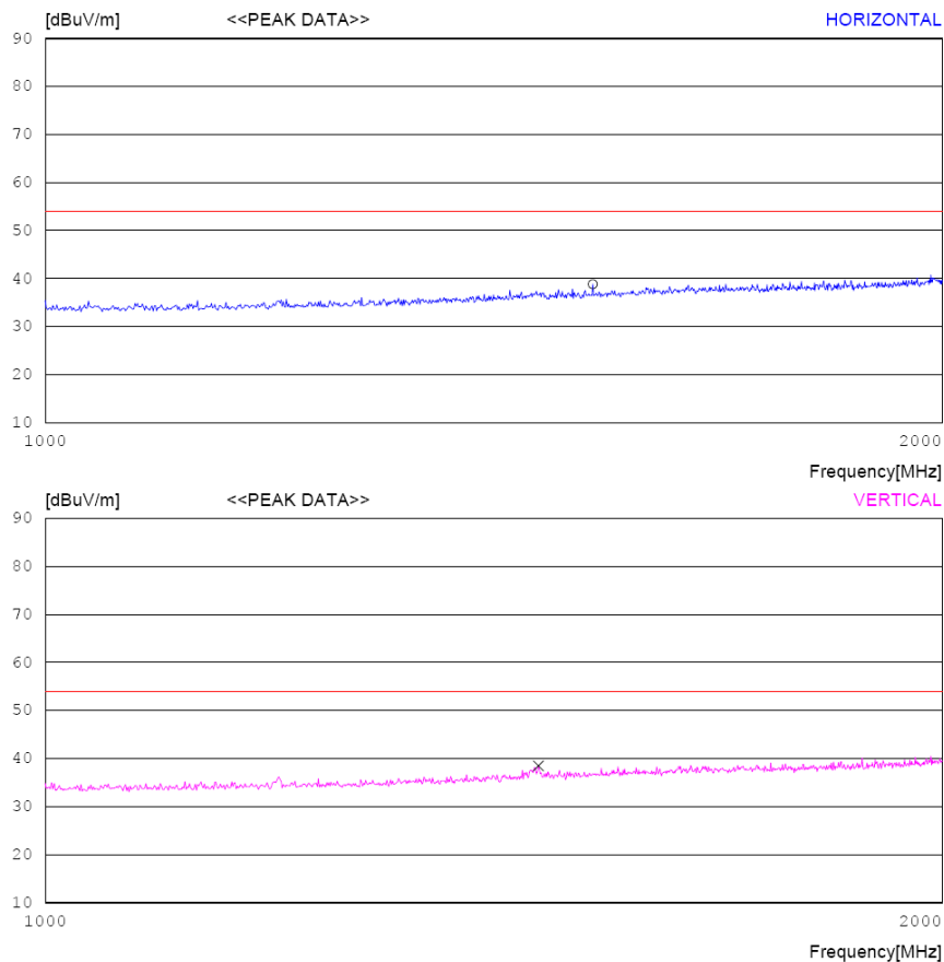
Radiated Emission Test 1 GHz - 2 GHz
