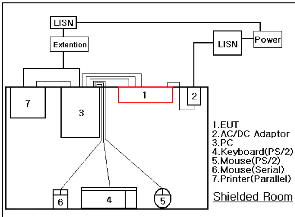
Conducted Emissions
