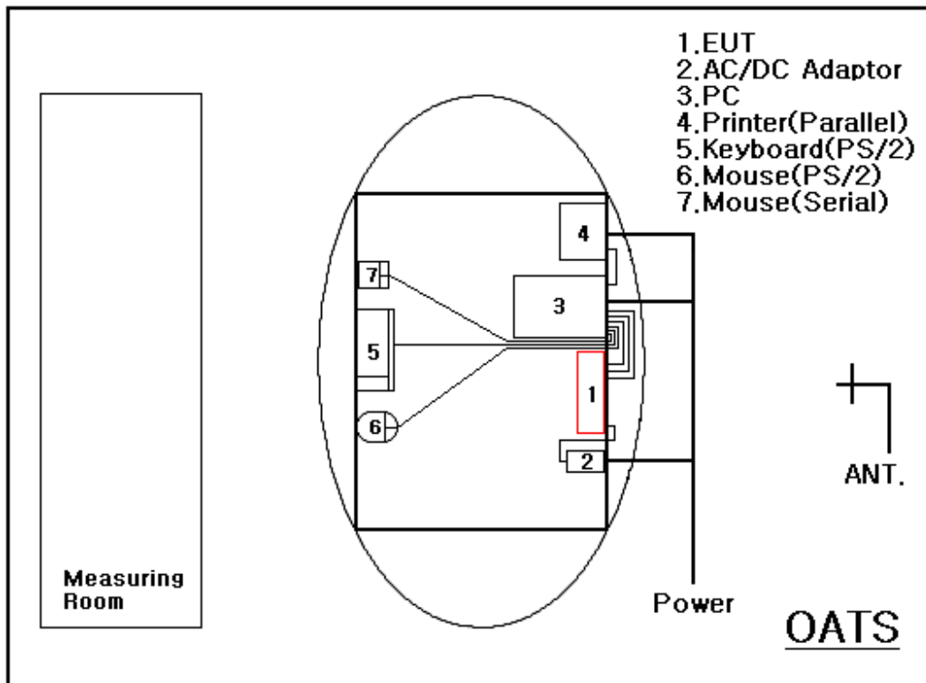
Radiated Emissions
