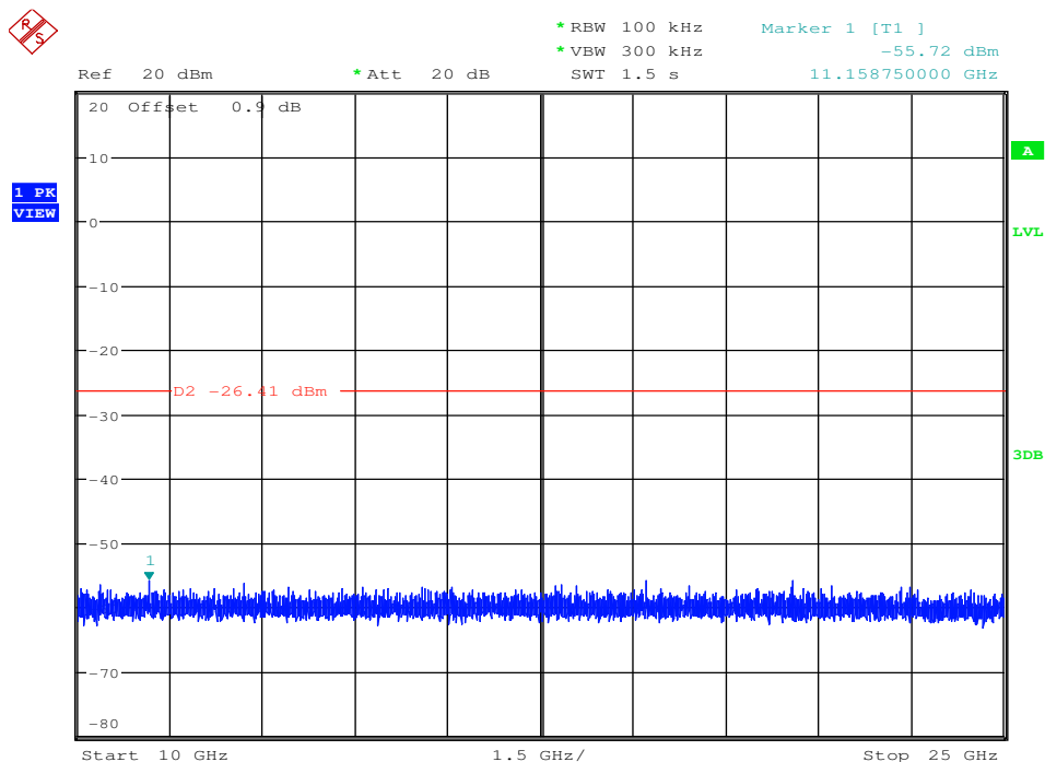
RF Conducted Spurious Emissions 11G 2462 Ant1
