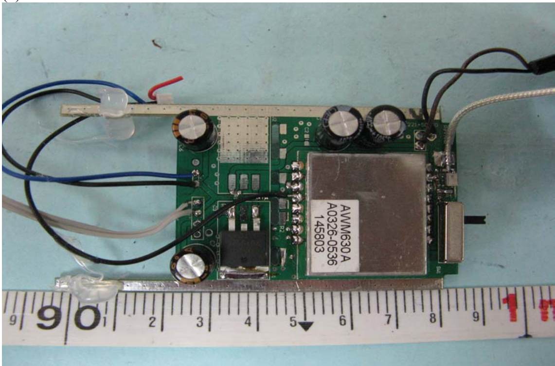
(8) Internal View of EUT
