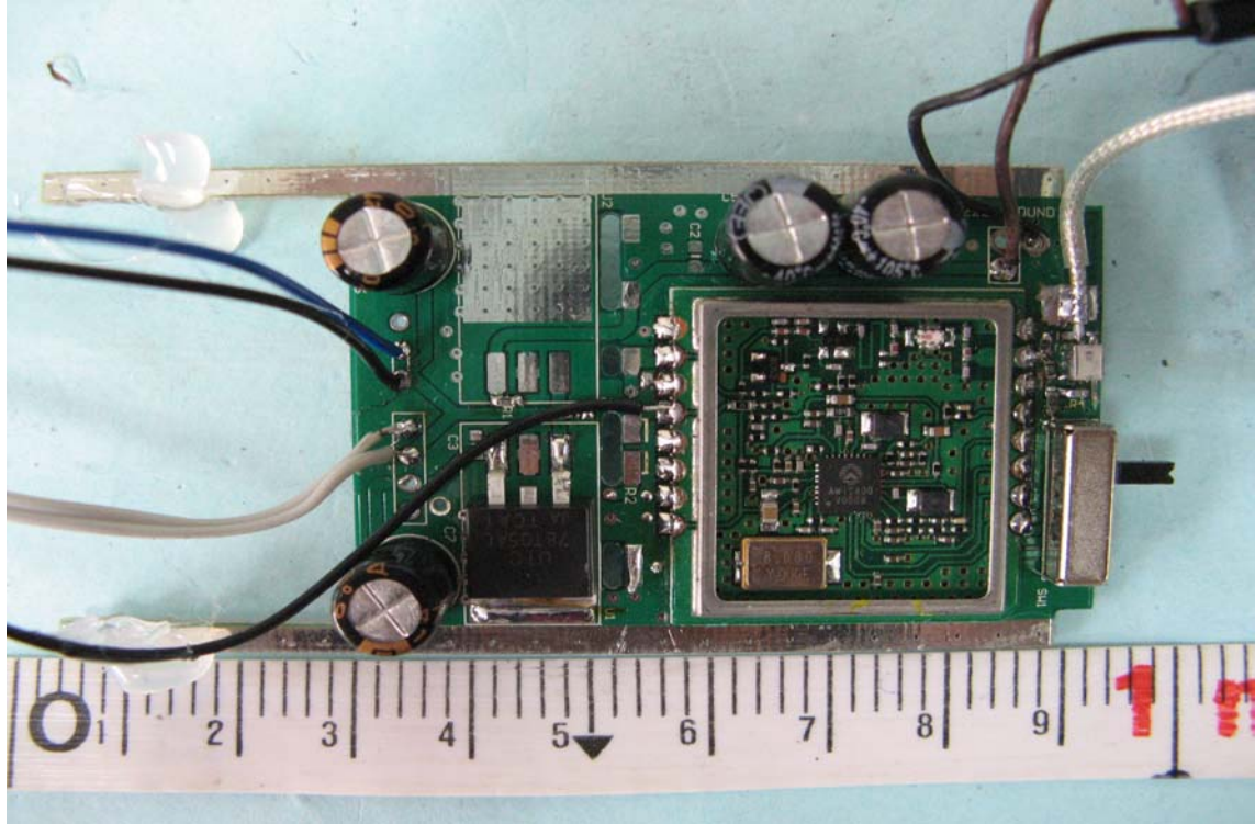
(9) Component View of PCB
