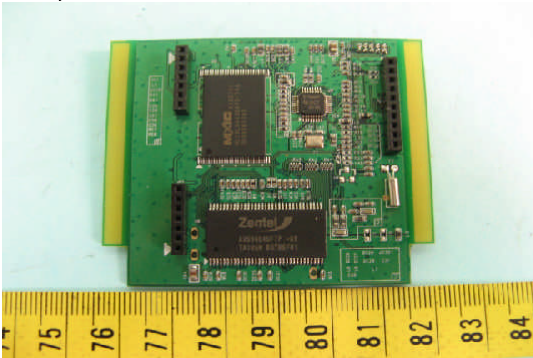
17. Component View of PCB
