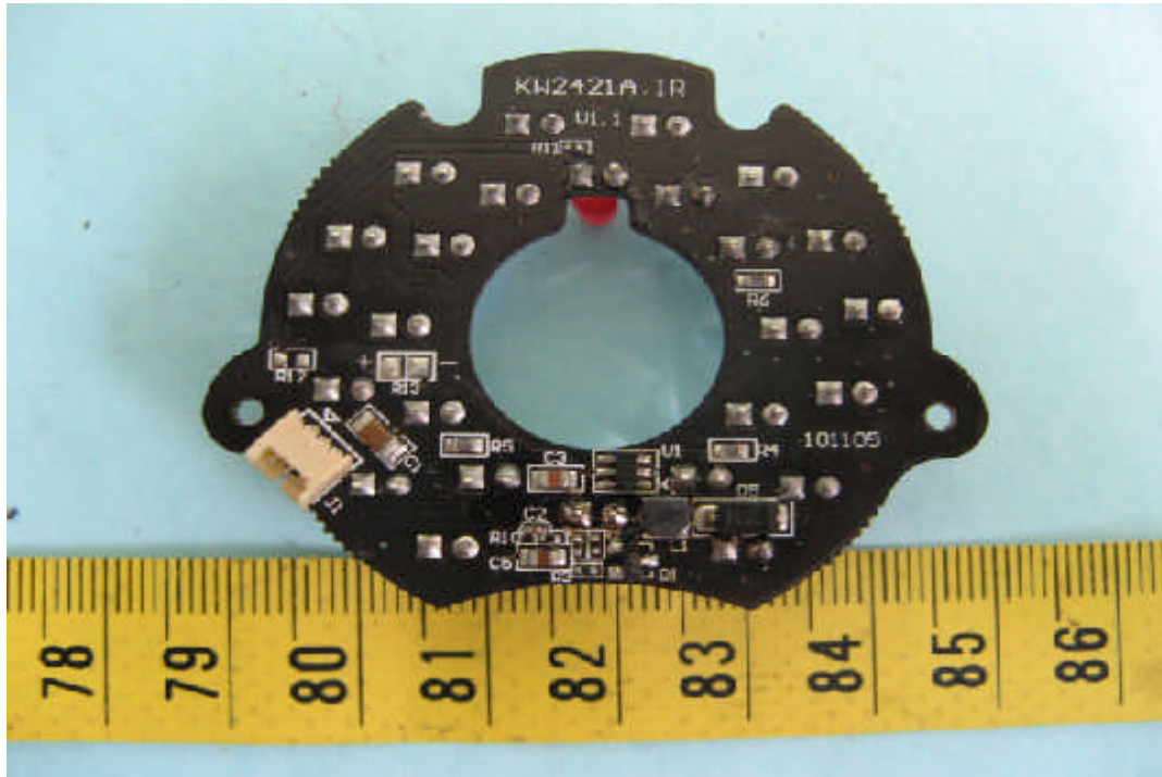
14. Component View of PCB
