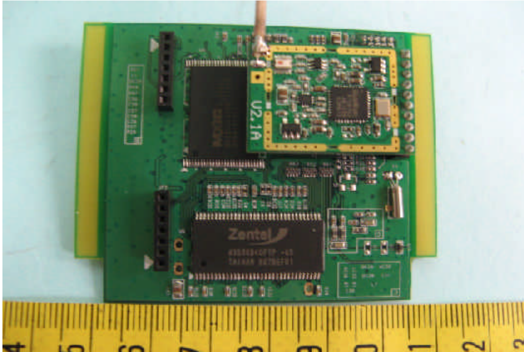
16. Component View of PCB
