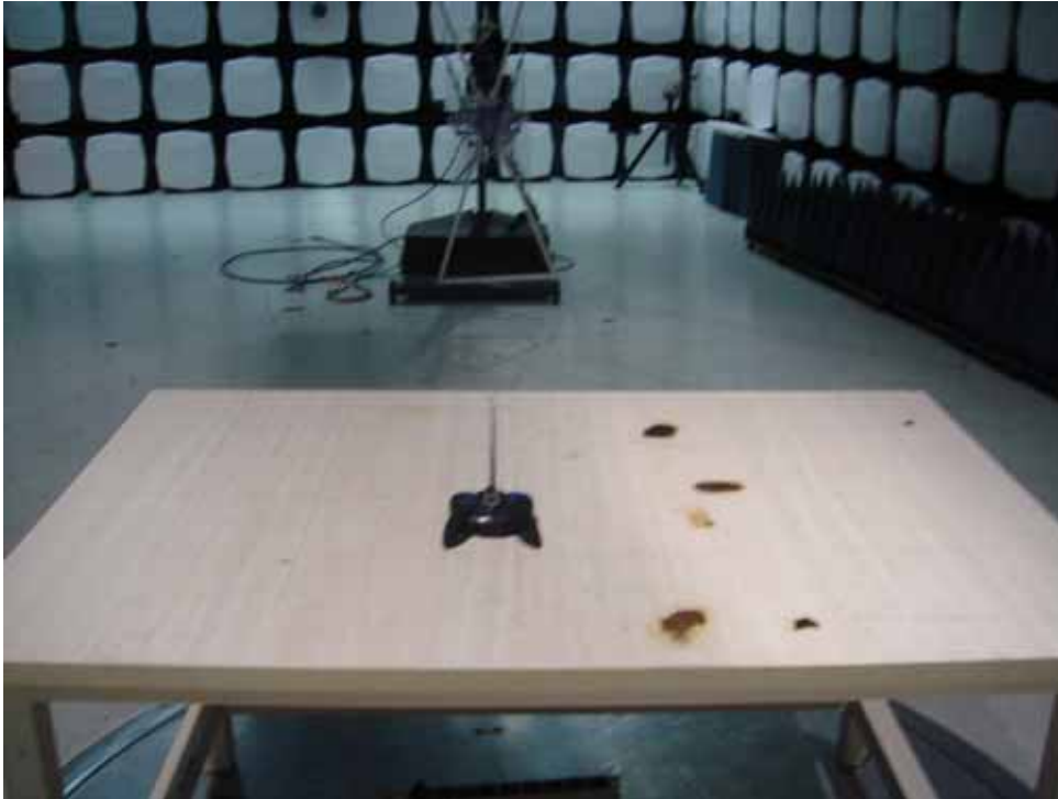
Radiation Emission Test setup
