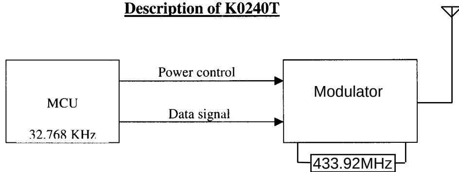
Figure 1. K0240T Block diagram
