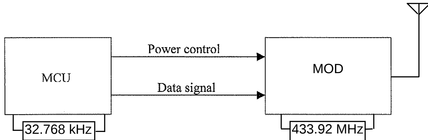
Figure 1. E0060-T Block diagram
