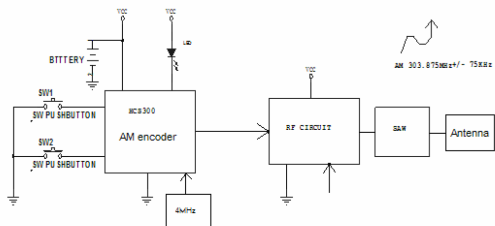
THE BLOCK DIAGRAM OF TRANSMITTER
