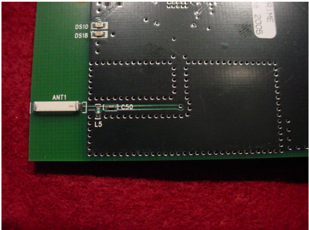
Figure 4: Internal – Bottom PCB Antenna View
