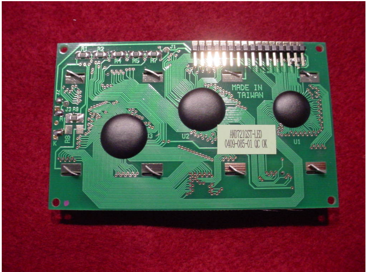
Figure 6: Internal – Bottom LCD View
