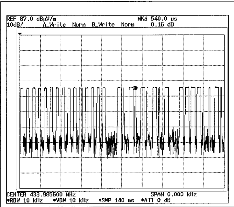
Duty Cycle 4
