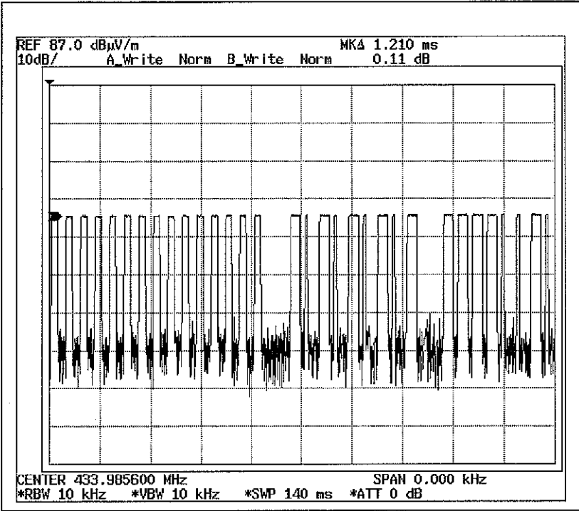
Duty Cycle 3
