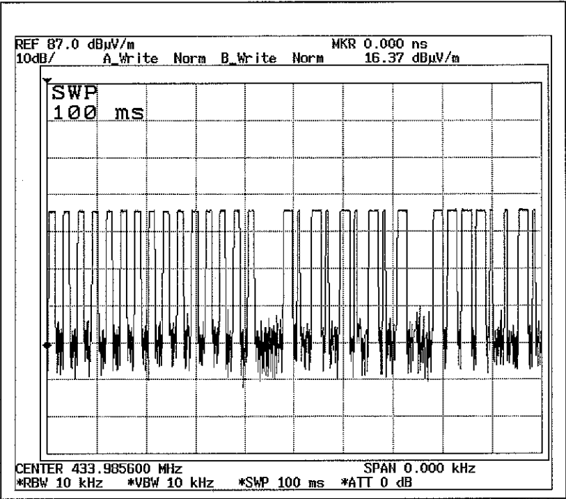
Duty Cycle 1
