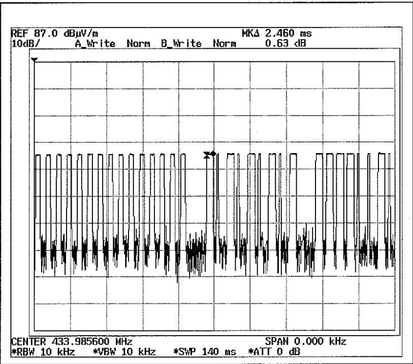
Duty Cycle 2
