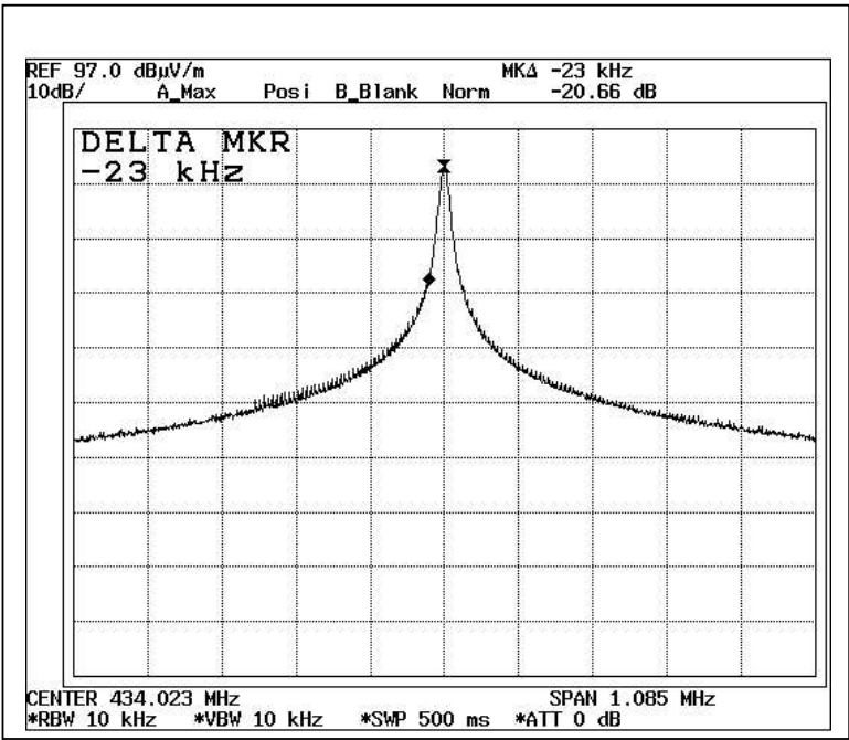
Bandwidth 2
