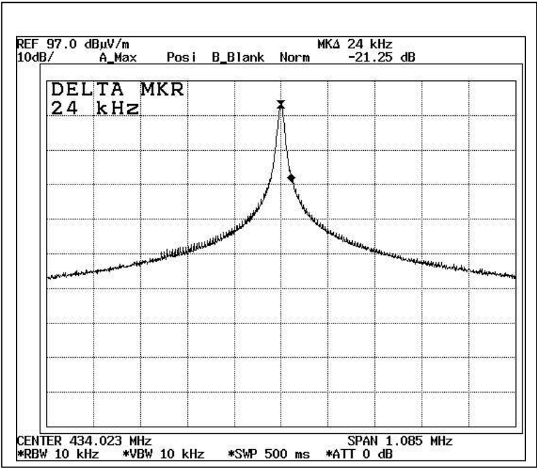
Bandwidth Plot
