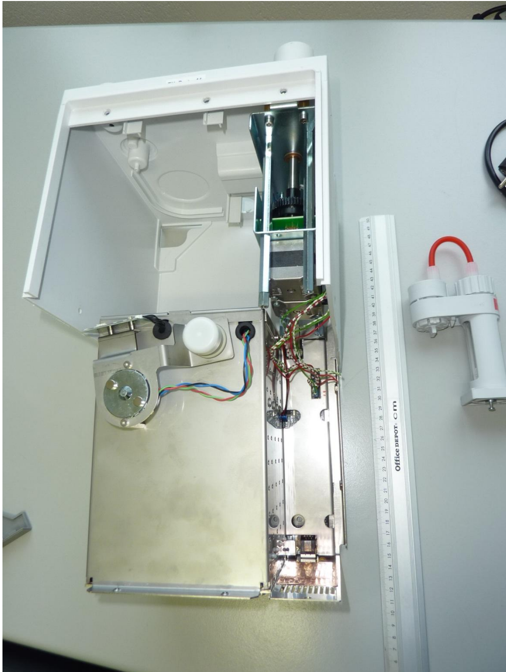
161791eut15.jpg: EUT (Excellence Titrator T9), internal view 1
