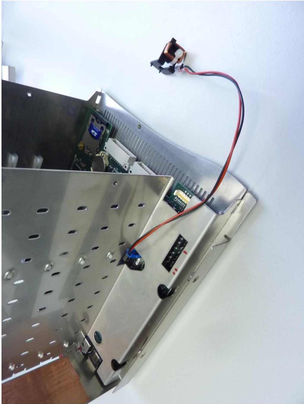
161791eut19.jpg: EUT (Excellence Titrator T9), internal view 3
