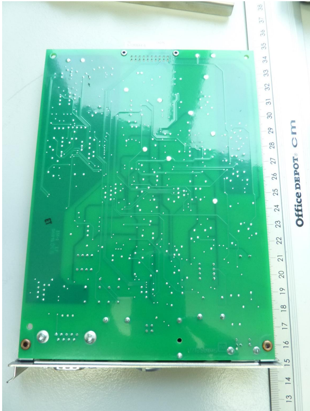
161791pcbD2.jpg: EUT (Excellence Titrator T9), PCB 4, bottom view
