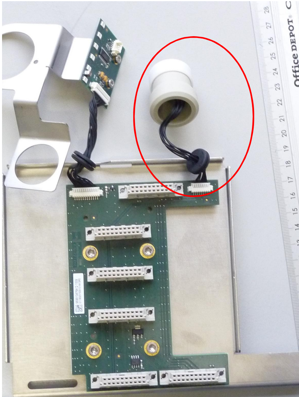
161791pcbA1.jpg: EUT (Excellence Titrator T9), PCB 1, top view 1
