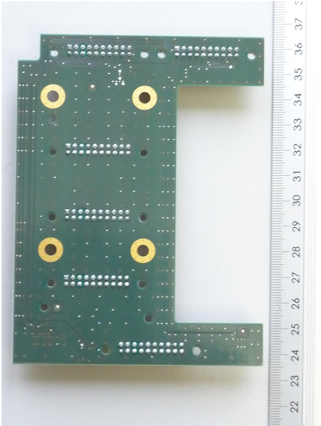
161791pcbA3.jpg: EUT (Excellence Titrator T9), PCB 1, bottom view
