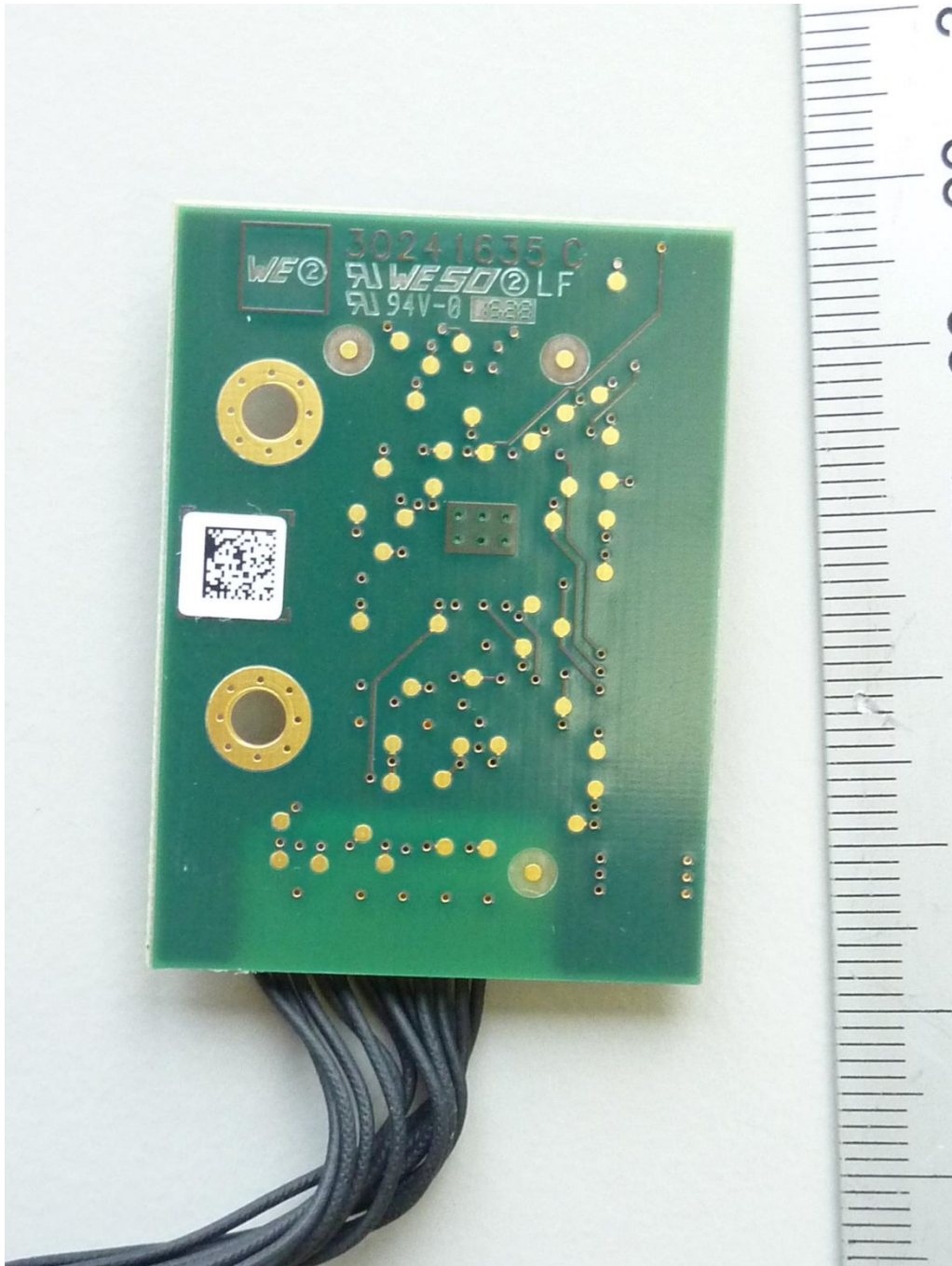
161791pcbB3.jpg: EUT (Excellence Titrator T9), PCB 2, bottom view
