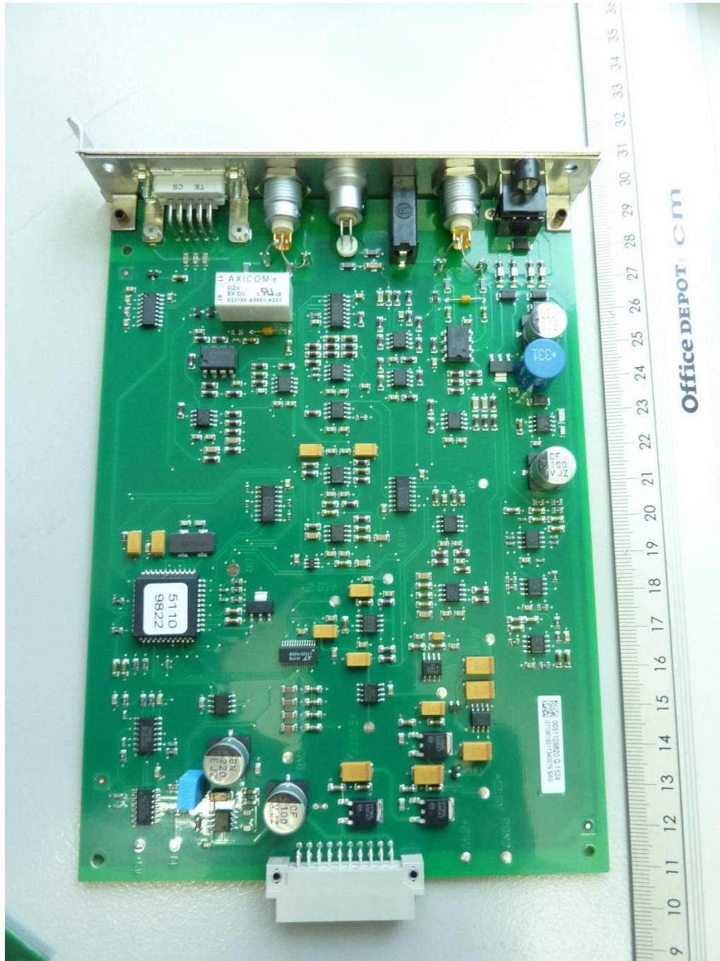
161791pcbD1.jpg: EUT (Excellence Titrator T9), PCB 4, top view
