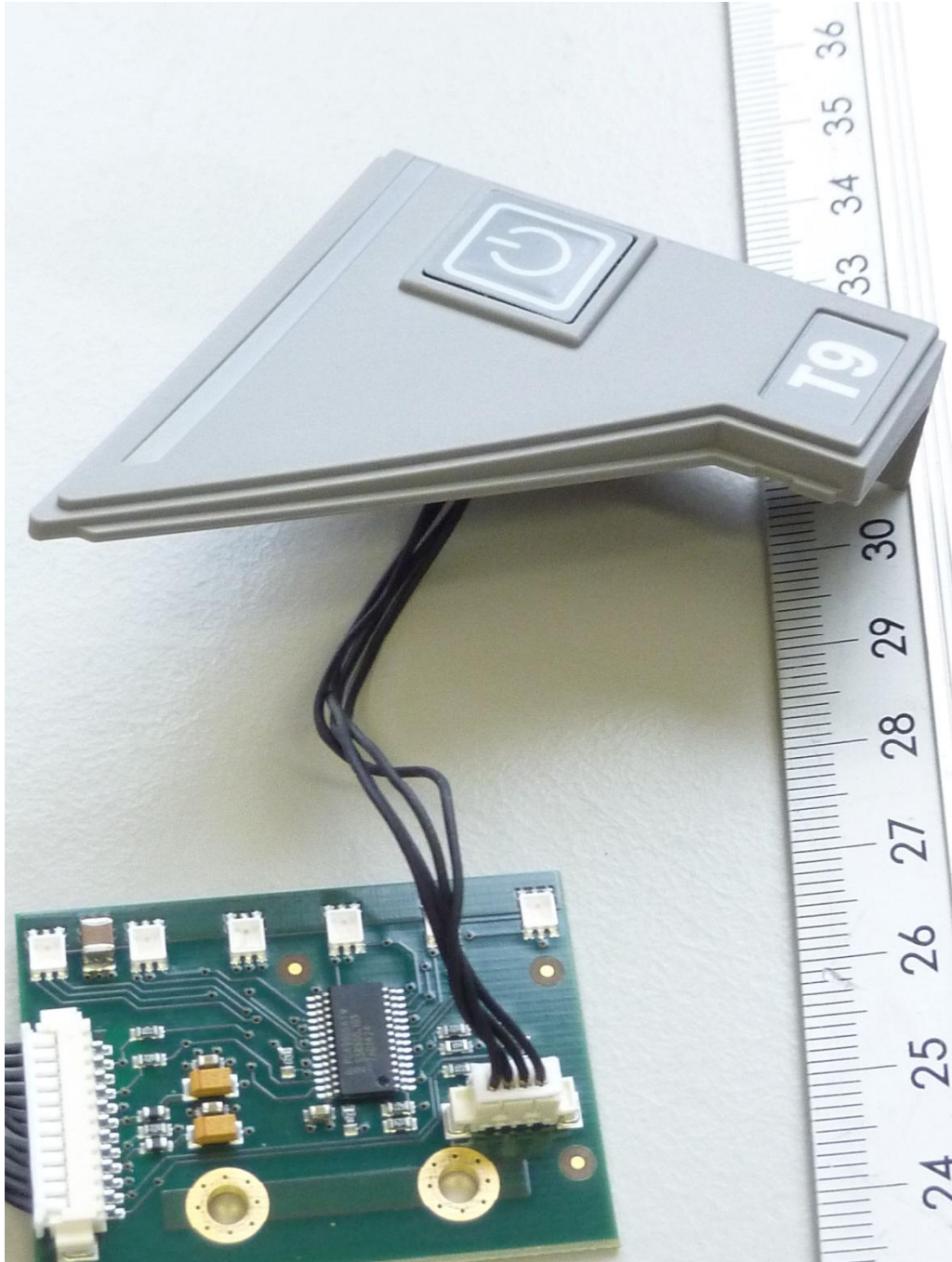
161791pcbB1.jpg: EUT (Excellence Titrator T9), PCB 2, top view 1
