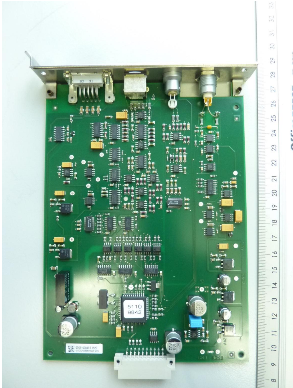
161791pcbC1.jpg: EUT (Excellence Titrator T9), PCB 3, top view
