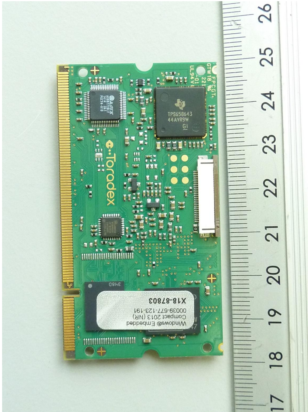
161791pcbF2.jpg: EUT (Excellence Titrator T9), PCB 6, bottom view
