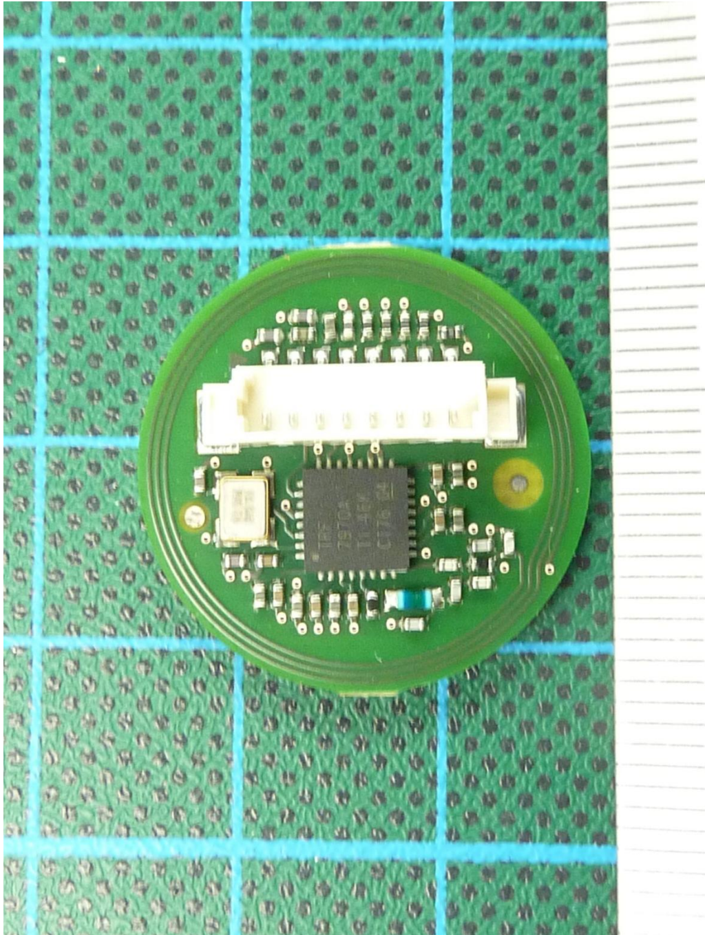
161791pcbG3.jpg: EUT (Excellence Titrator T9), PCB 7, 13.56 MHz RFID reader, top view
