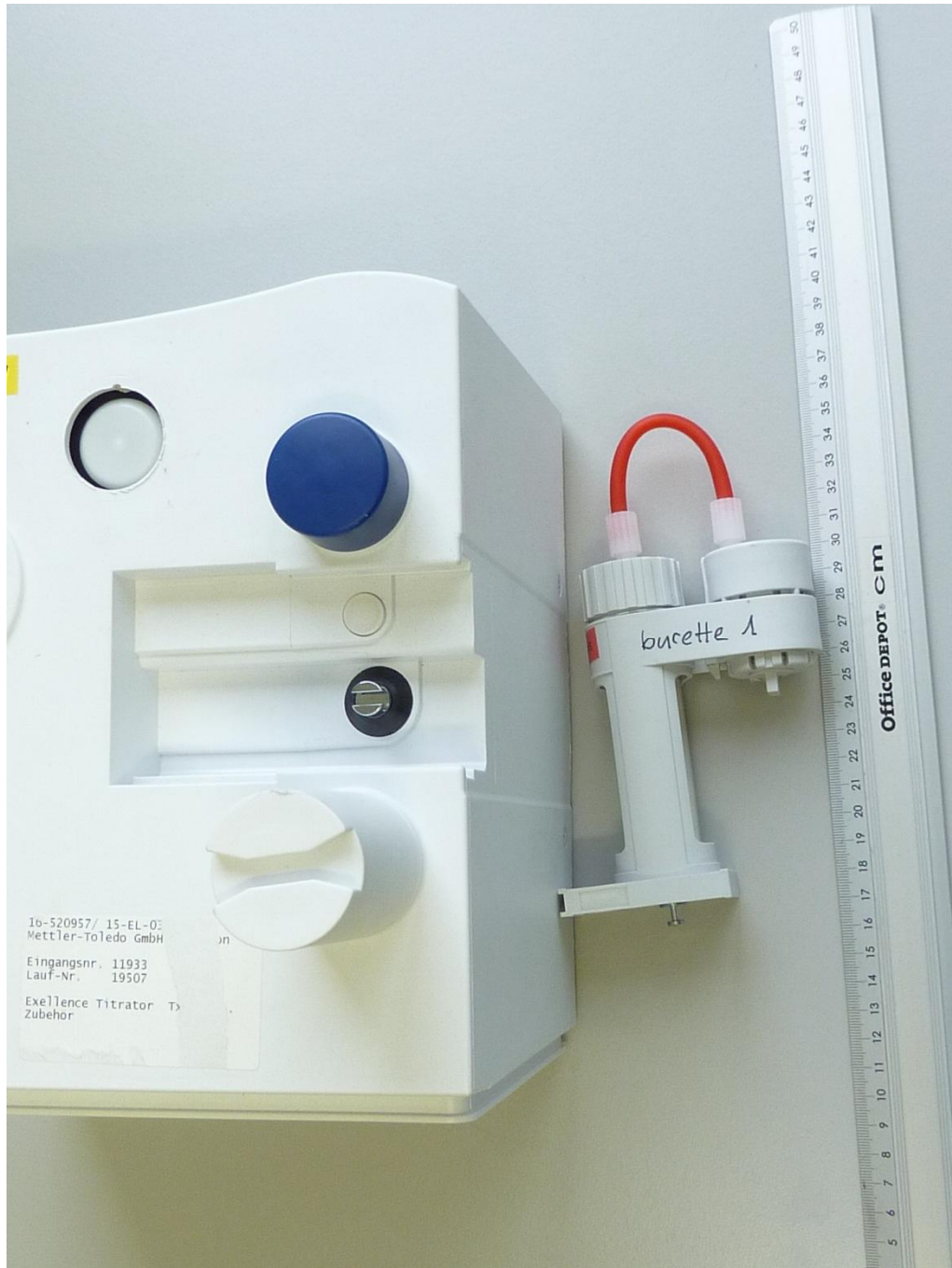
161791eut7.jpg: EUT (Excellence Titrator T9), top view, burette removed
