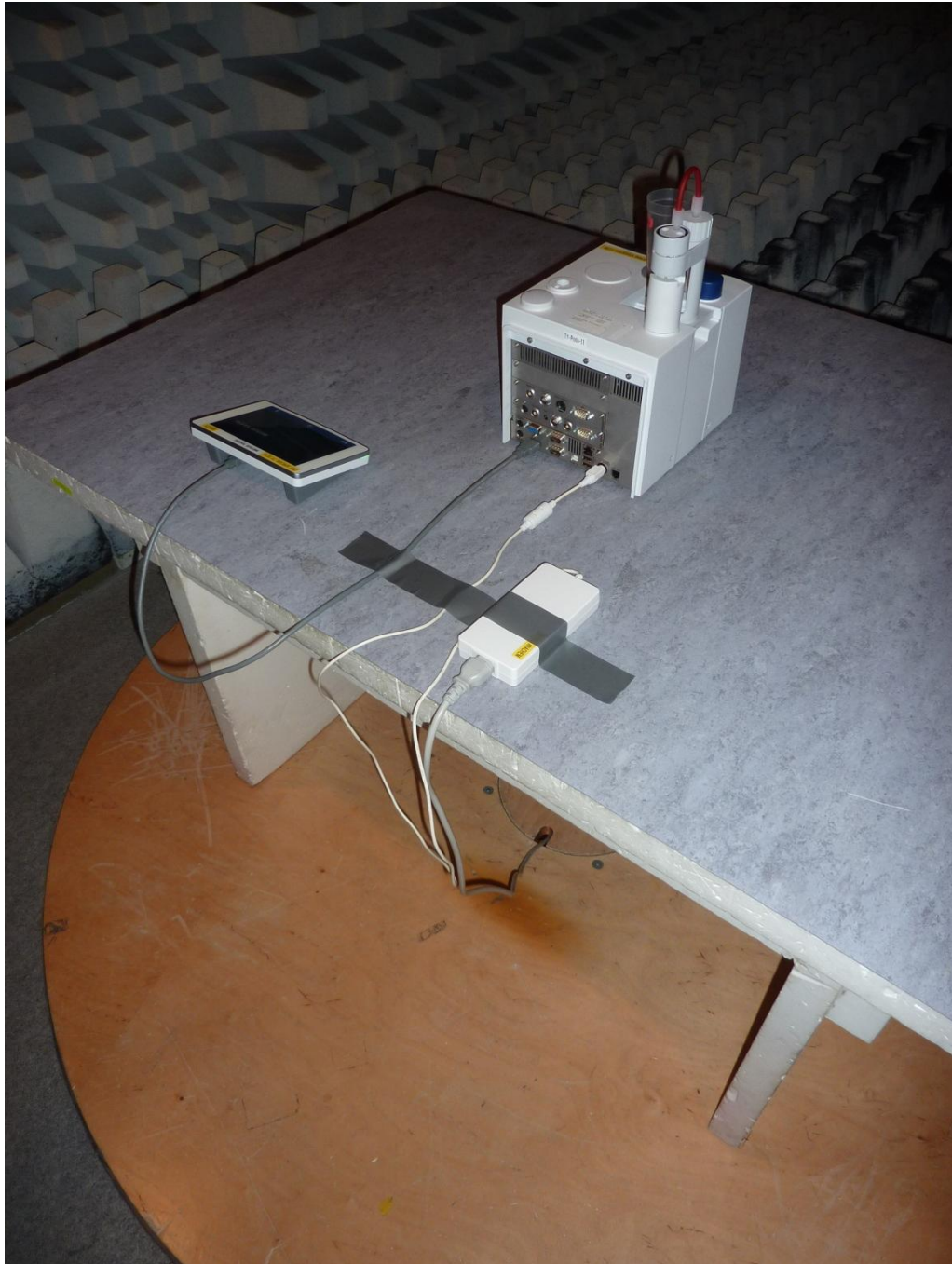
161791emiB1.jpg: EUT (Excellence Titrator T9), test setup fully anechoic chamber
