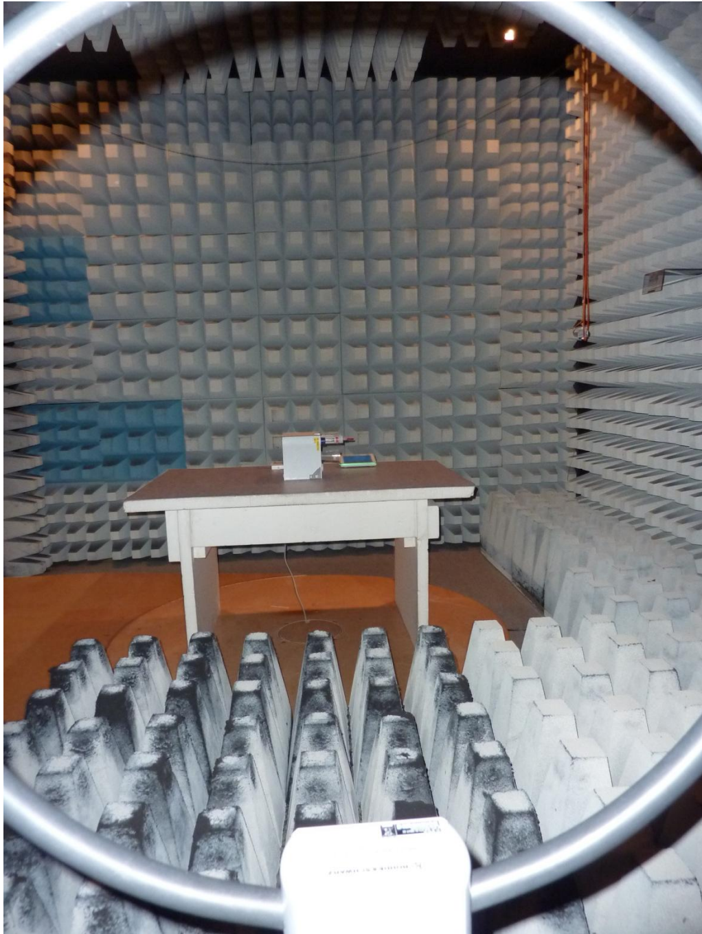
161791emiB2.jpg: EUT (Excellence Titrator T9), test setup fully anechoic chamber
