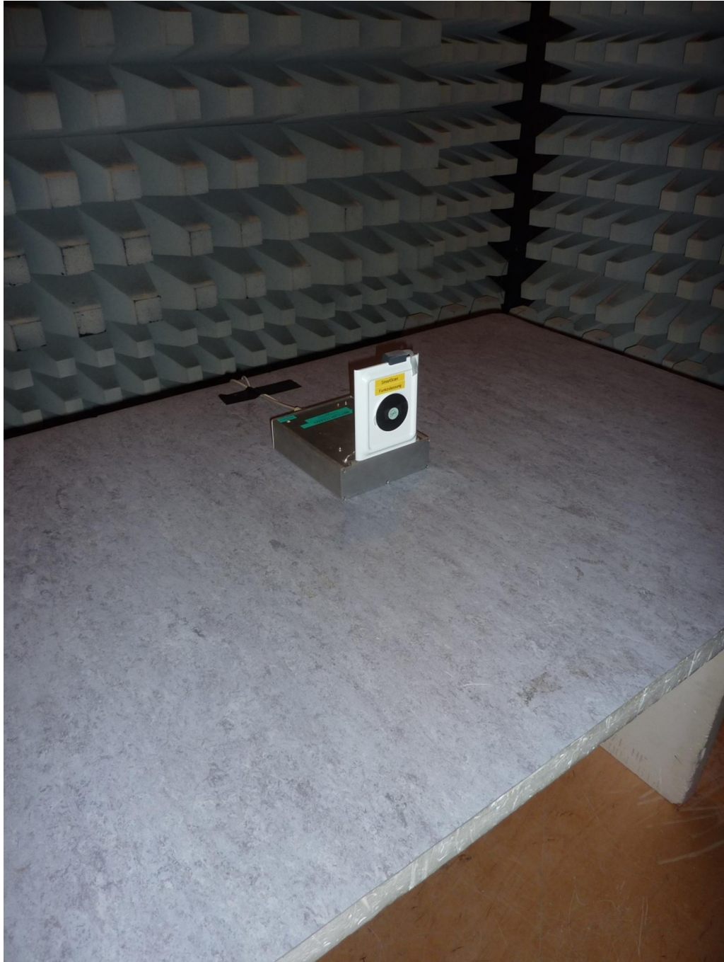
172416_7.jpg: SmartScan, test set-up fully anechoic chamber
