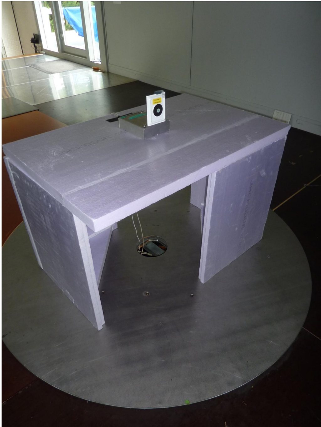
172416_14.jpg: SmartScan, test set-up open area test site
