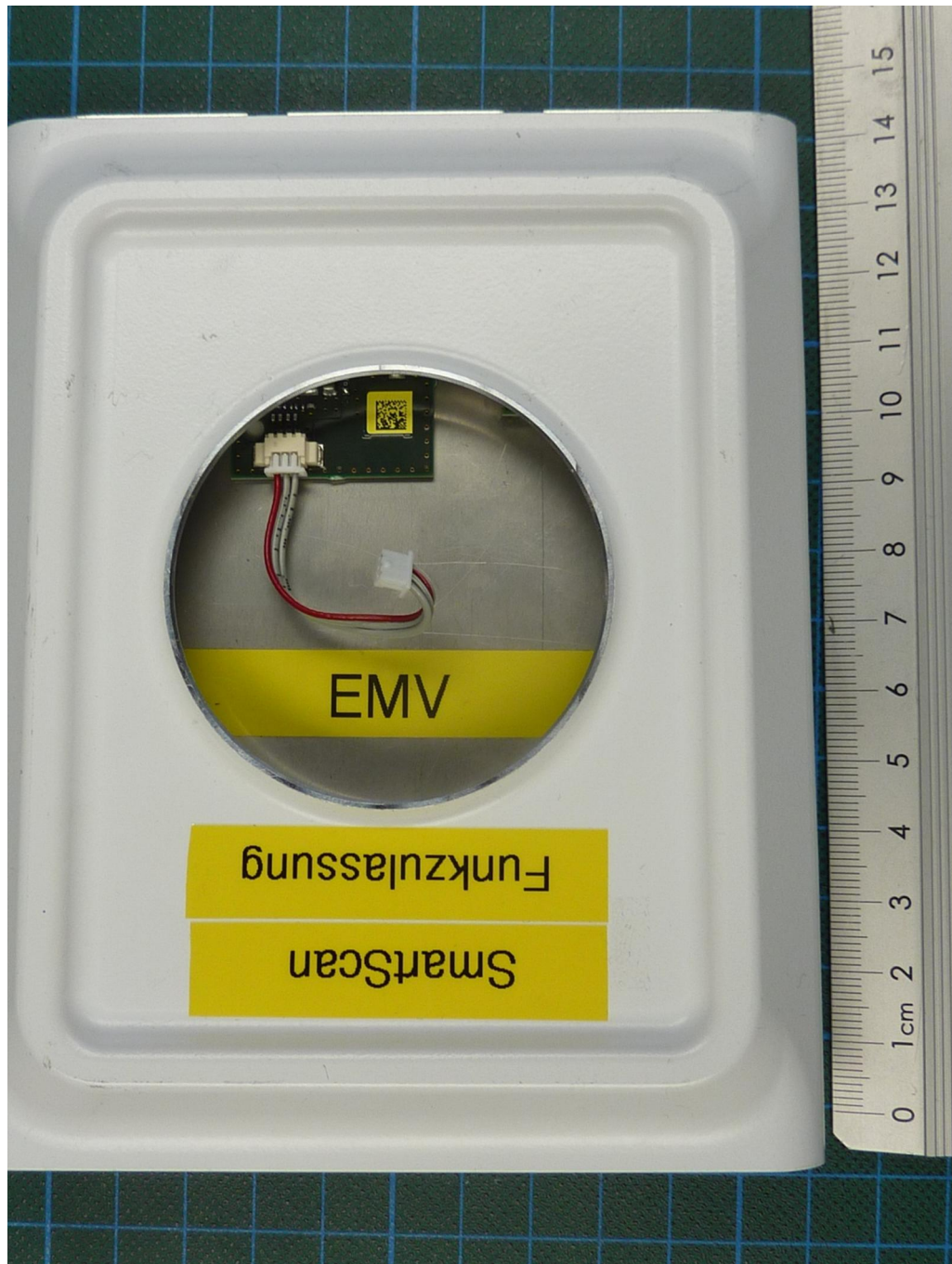
172416_n.jpg: SmartScan, internal view 1 (antenna removed)
