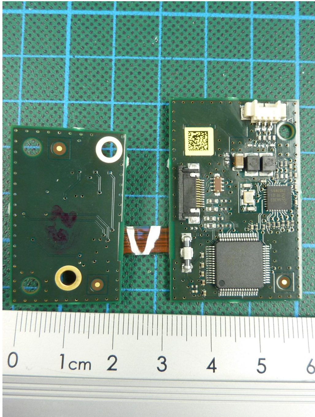
172416_p.jpg: SmartScan, PCB, top view
