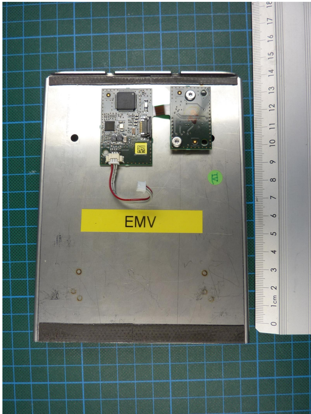
172416_I.jpg: SmartScan, internal view 2 (housing removed)
