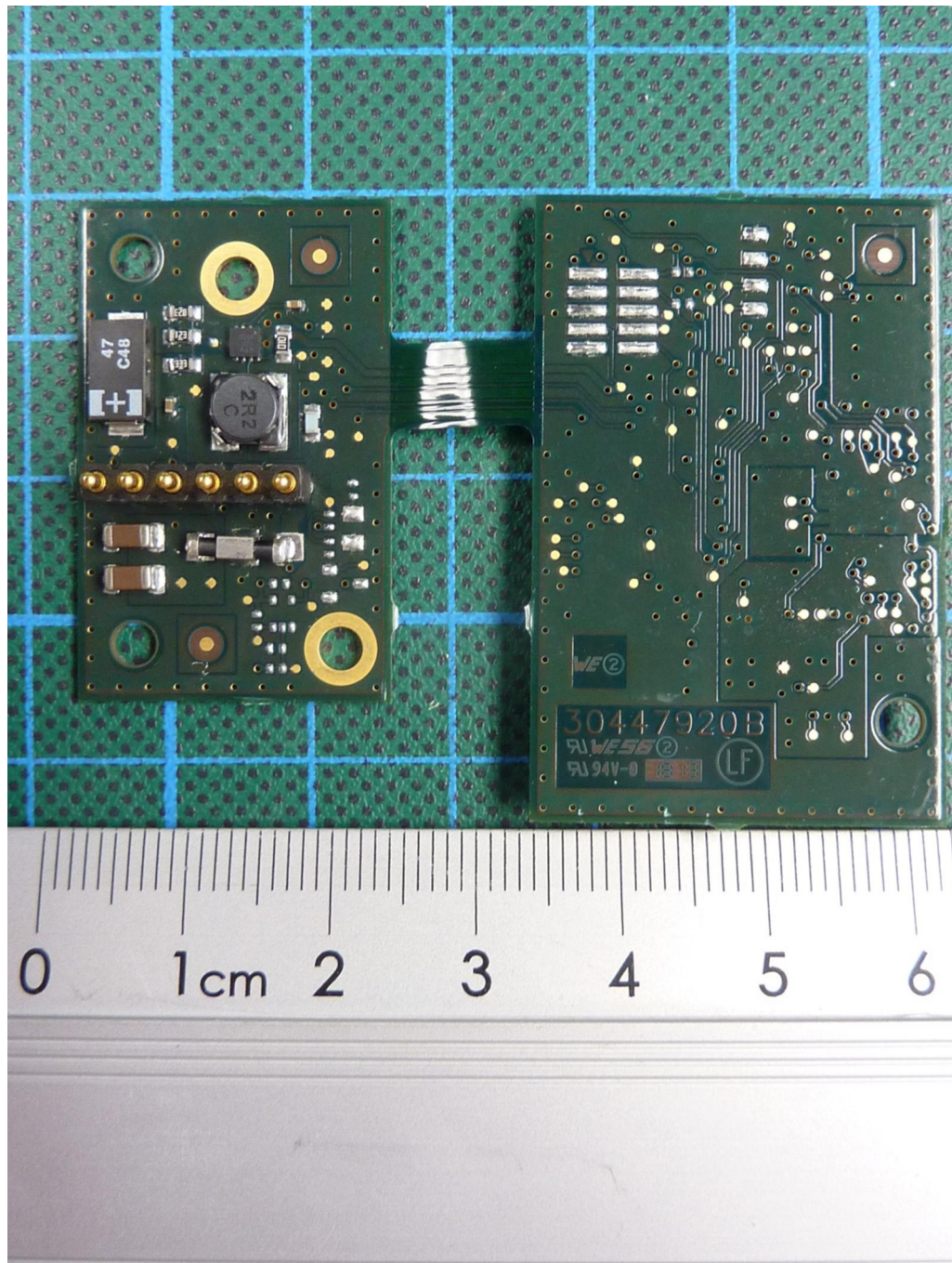
172416_q.jpg: SmartScan, PCB, bottom view
