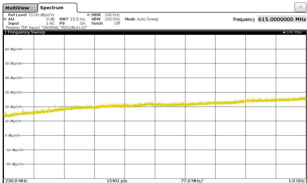
181223_205.png: Spurious emissions from 230 MHz to 1 GHz
