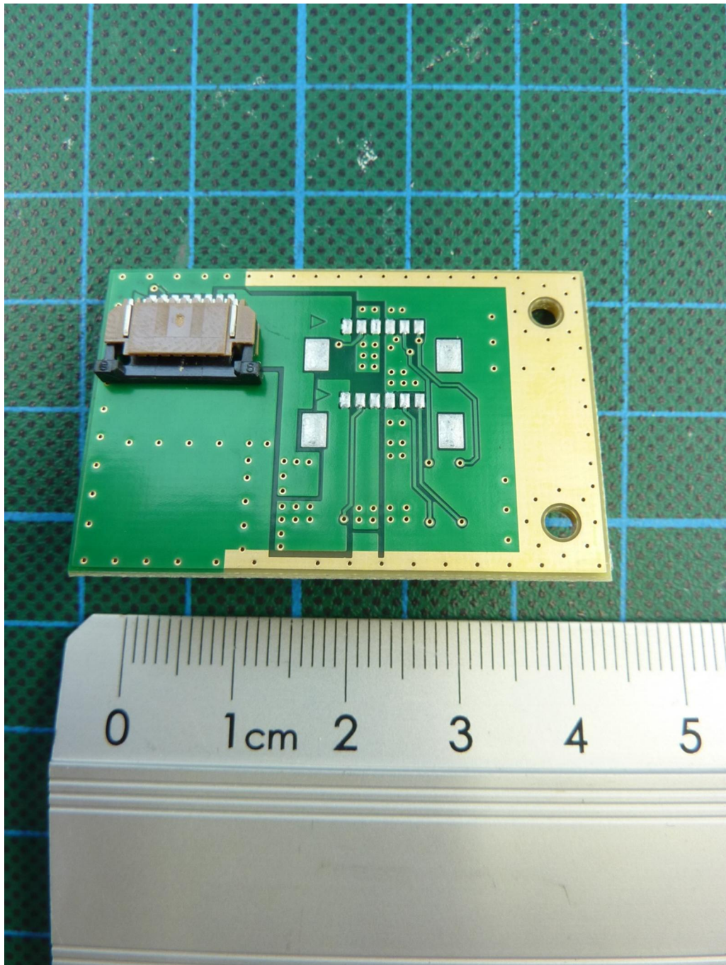
181223_15.jpg: QLX3 liquid module, connector PCB, bottom view
