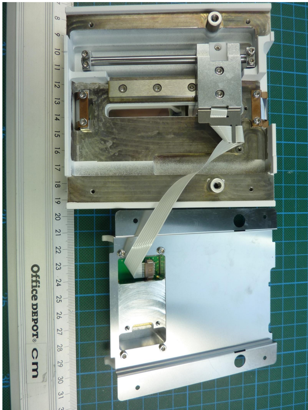
181223_12.jpg: QLX3 liquid module, housing opened
