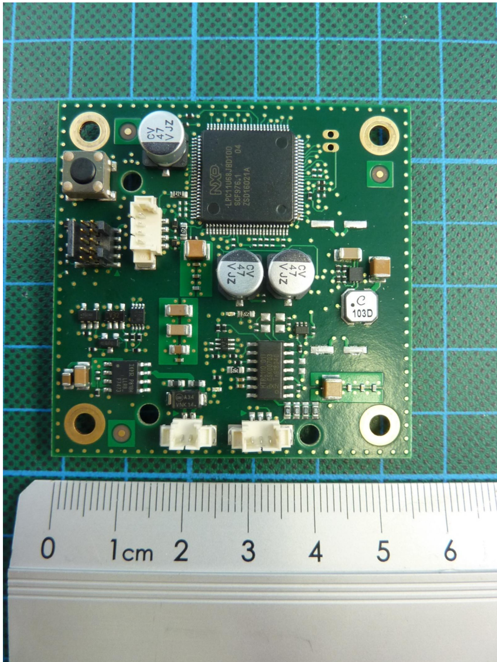
181223_9.jpg: QLX3 liquid module, reader PCB, top view
