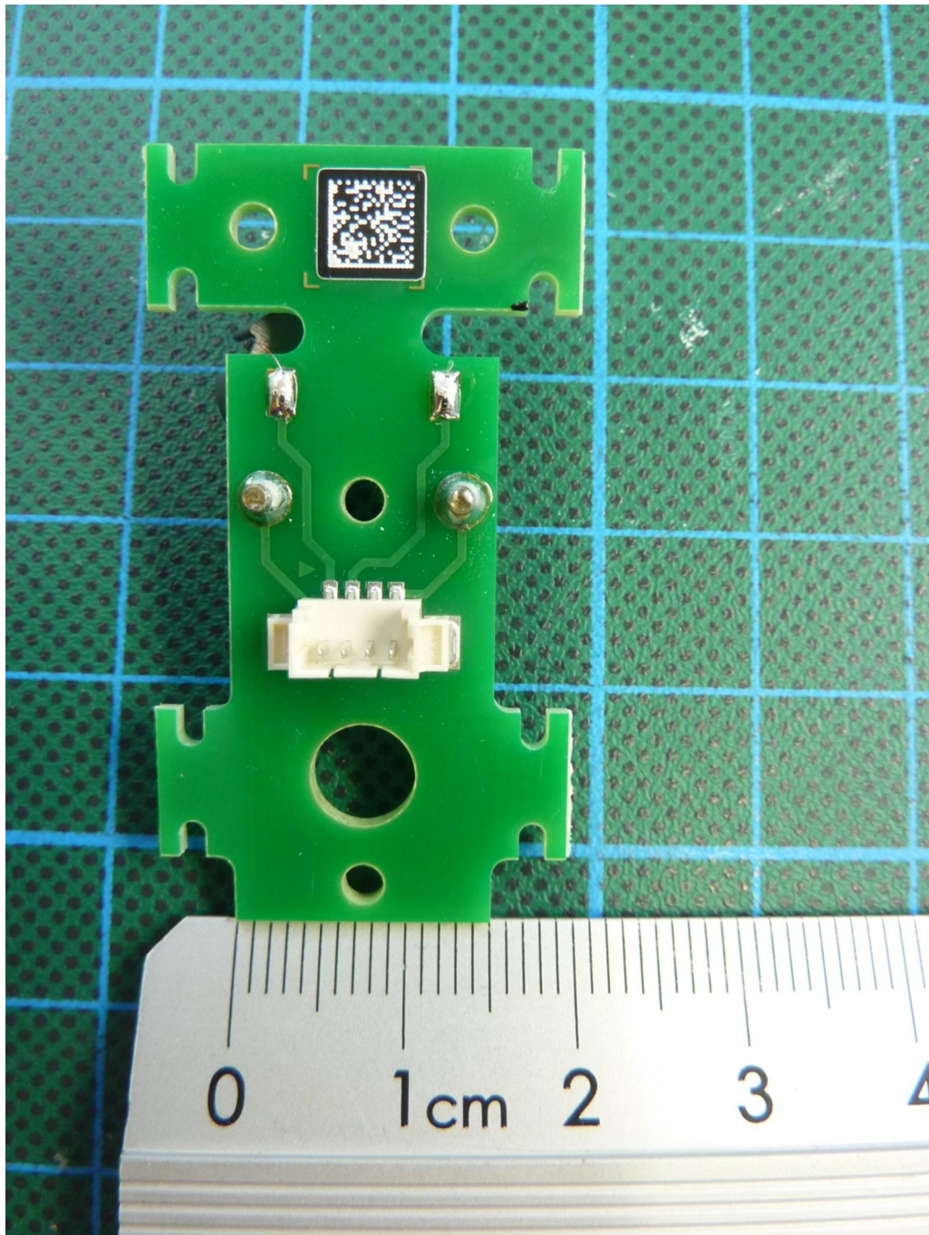
181223_11.jpg: QLX3 liquid module, antenna PCB, bottom view
