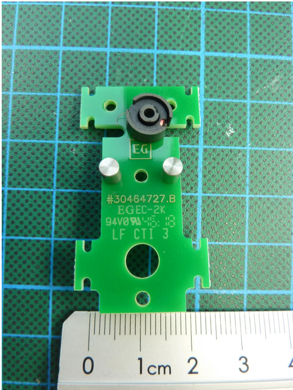
181223_10.jpg: QLX3 liquid module, antenna PCB, top view
