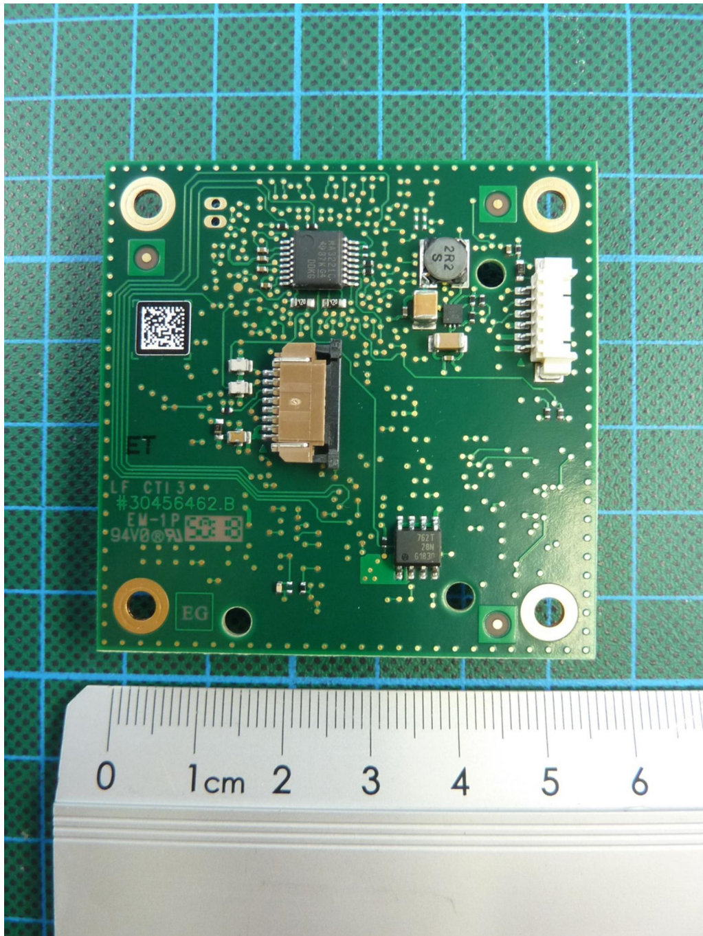
181223_8.jpg: QLX3 liquid module, reader PCB, bottom view
