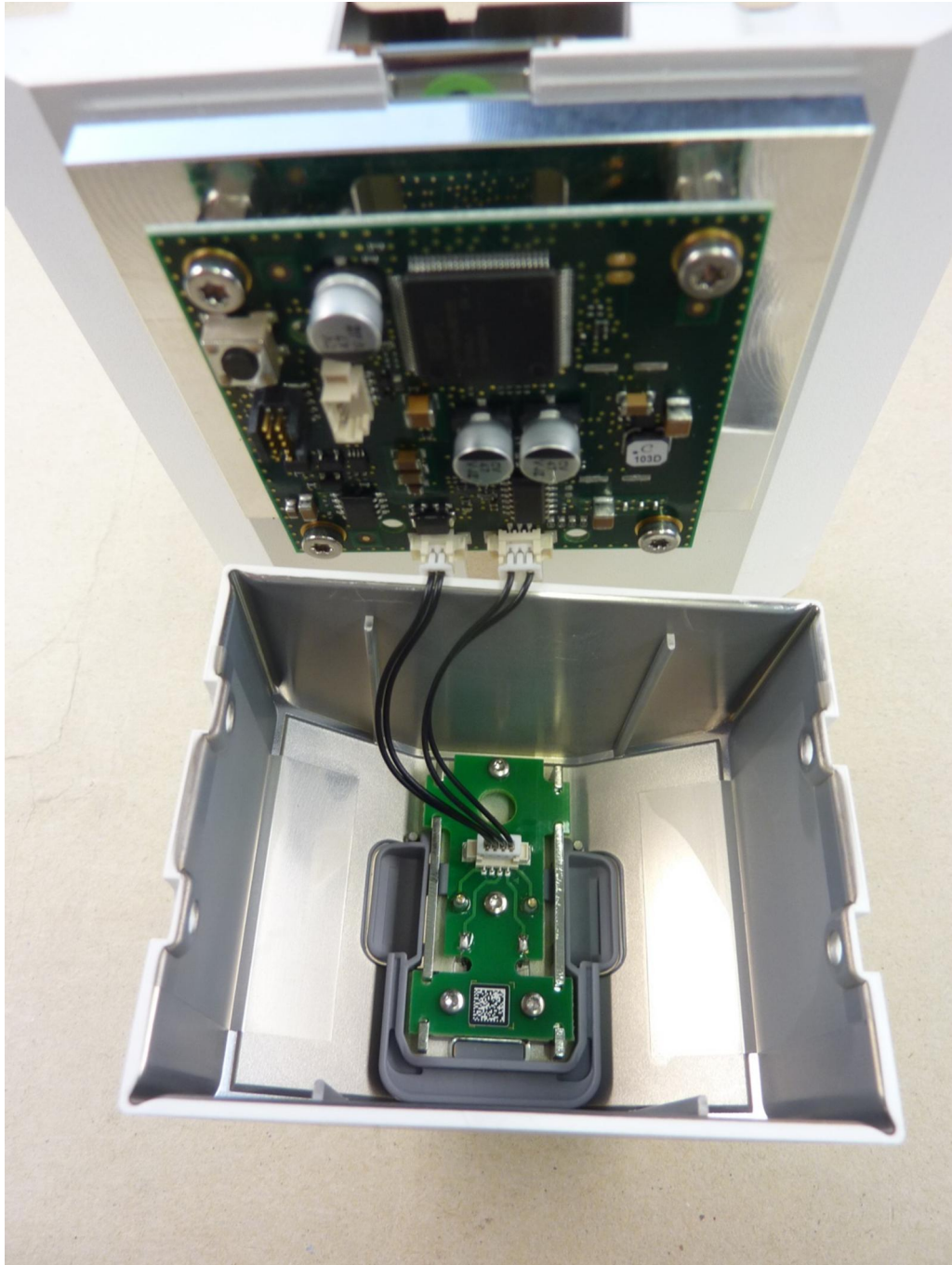
181223_5.jpg: QLX3 liquid module, internal view, front cover opened
