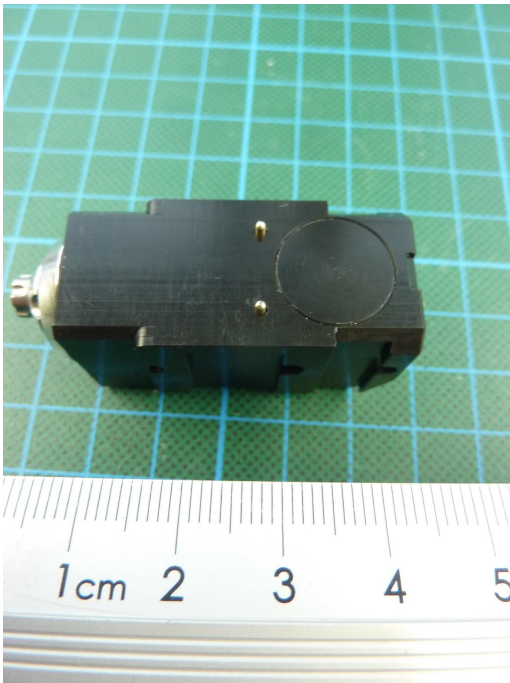
181223_19.jpg: Dosing head QL001 (with TAG), rear view
