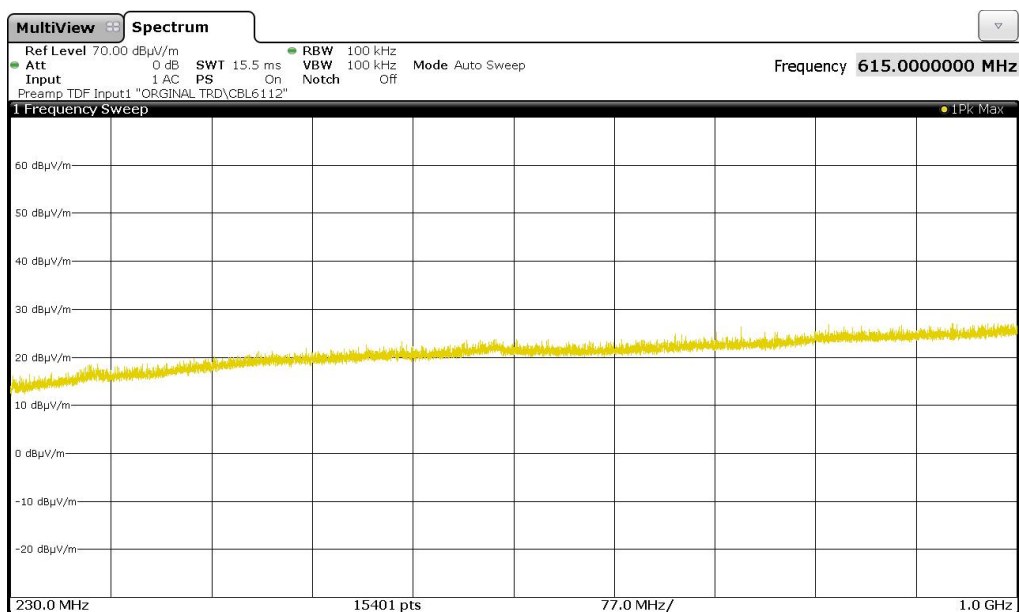
182314_205.png: Spurious emissions from 230 MHz to 1 GHz
