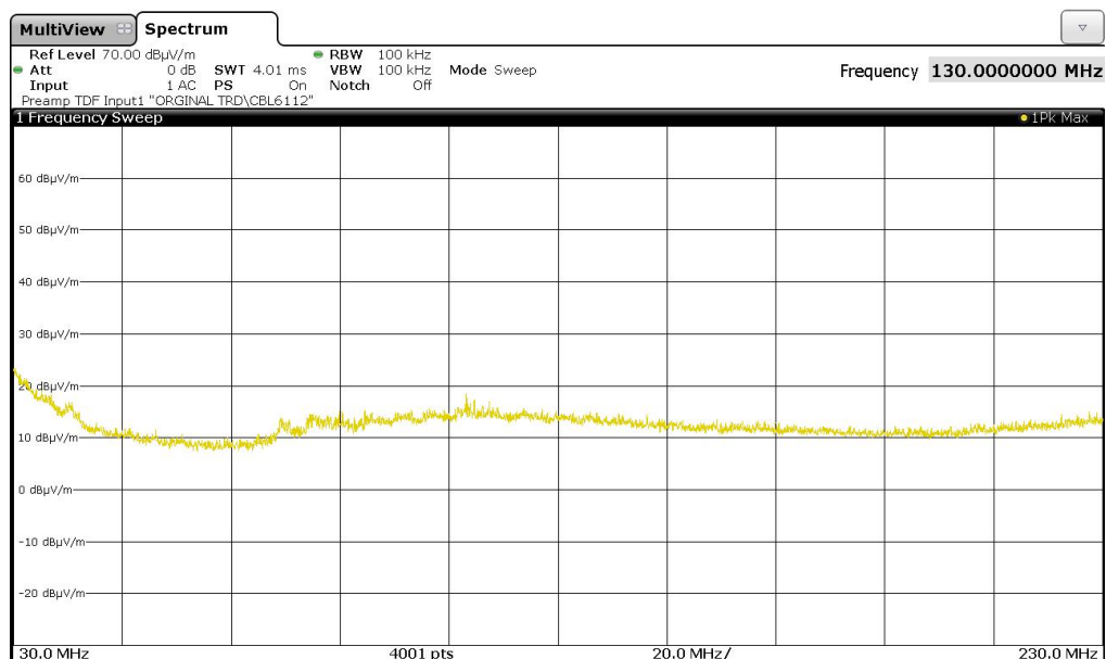
182314_204.png: Spurious emissions from 30 MHz to 230 MHz
