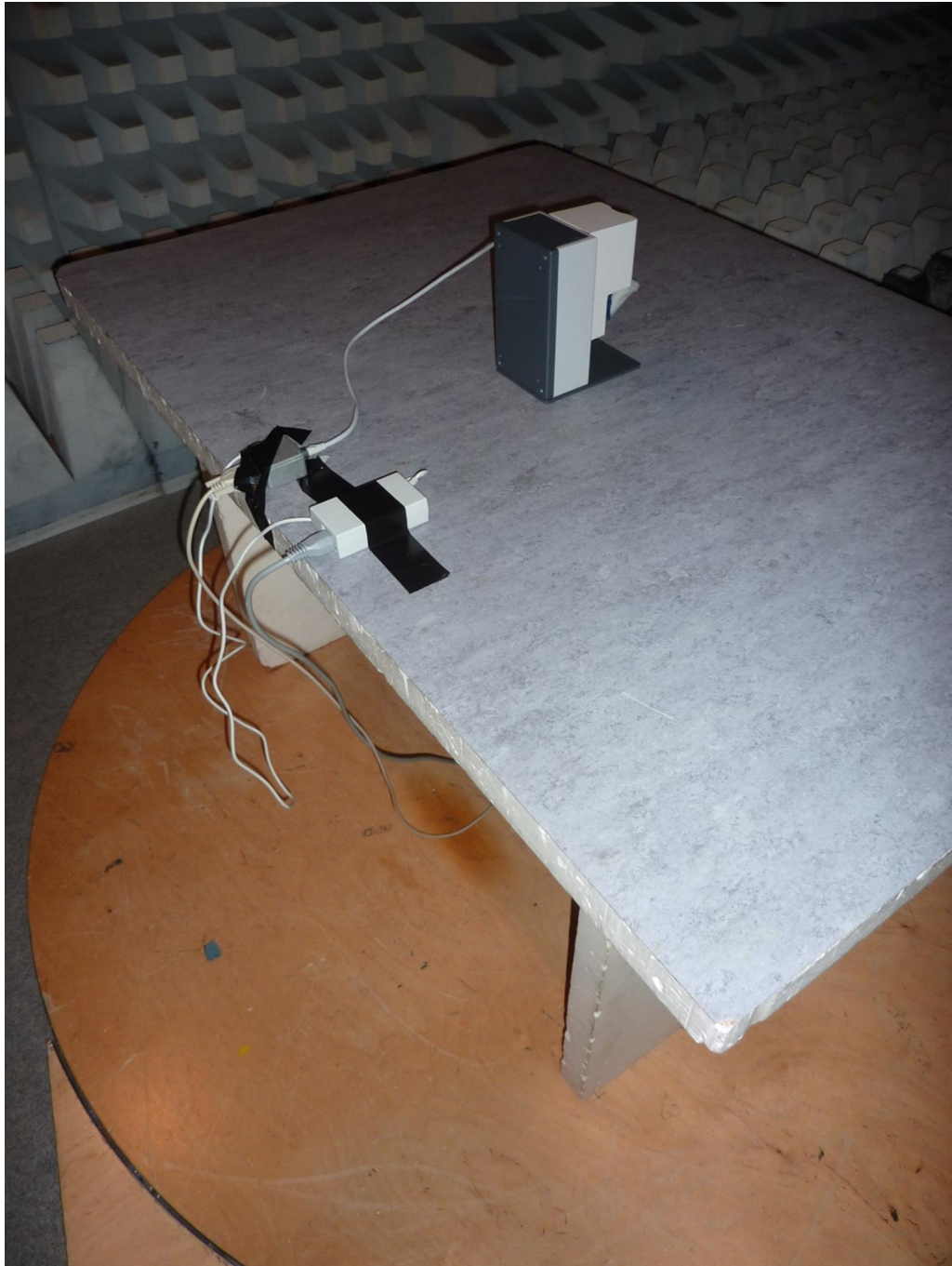
182314_g.jpg: dosing module, test setup fully anechoic chamber
