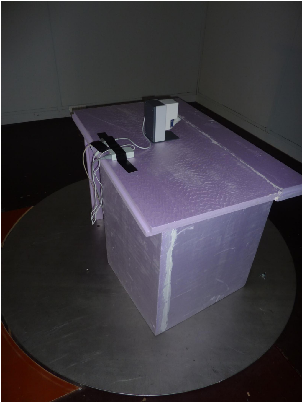
182314_n.jpg: dosing module, test setup open area test site
