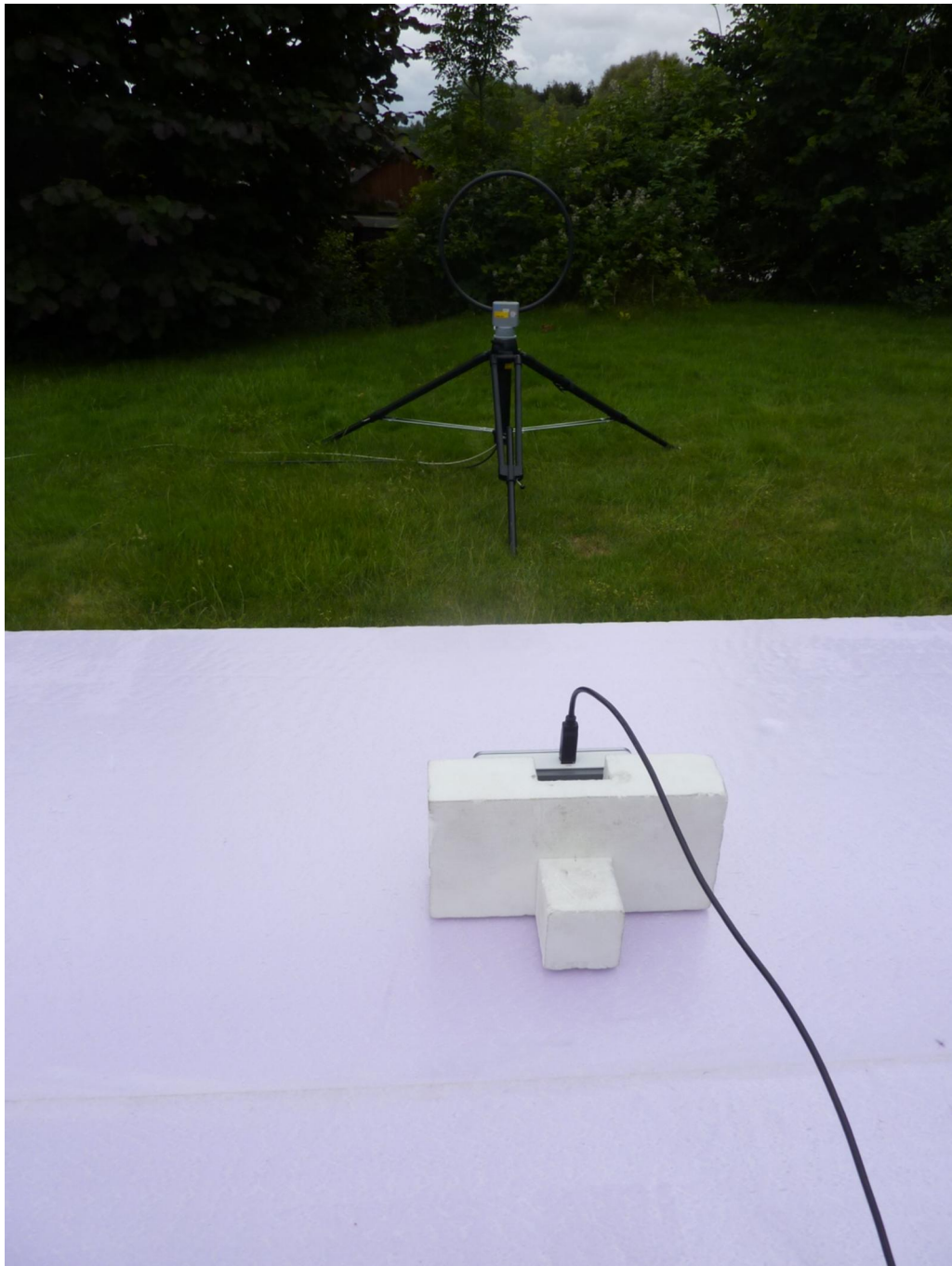
172414_16.jpg: EasyScan USB, test set-up open area test site
