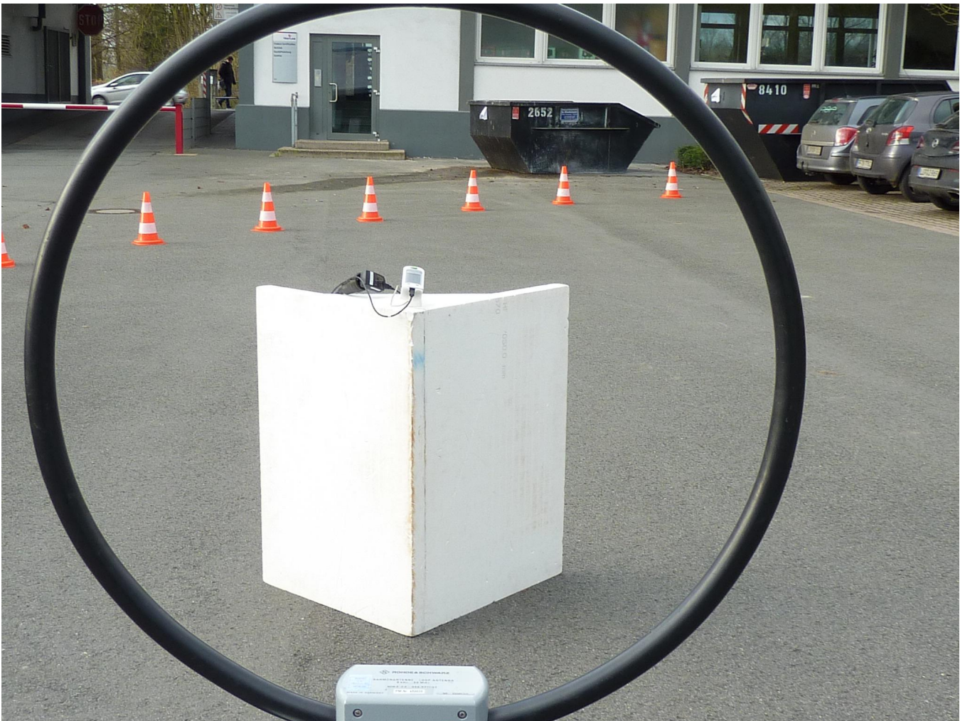
172251_209_04: test setup outdoor test site magnetic field strength
