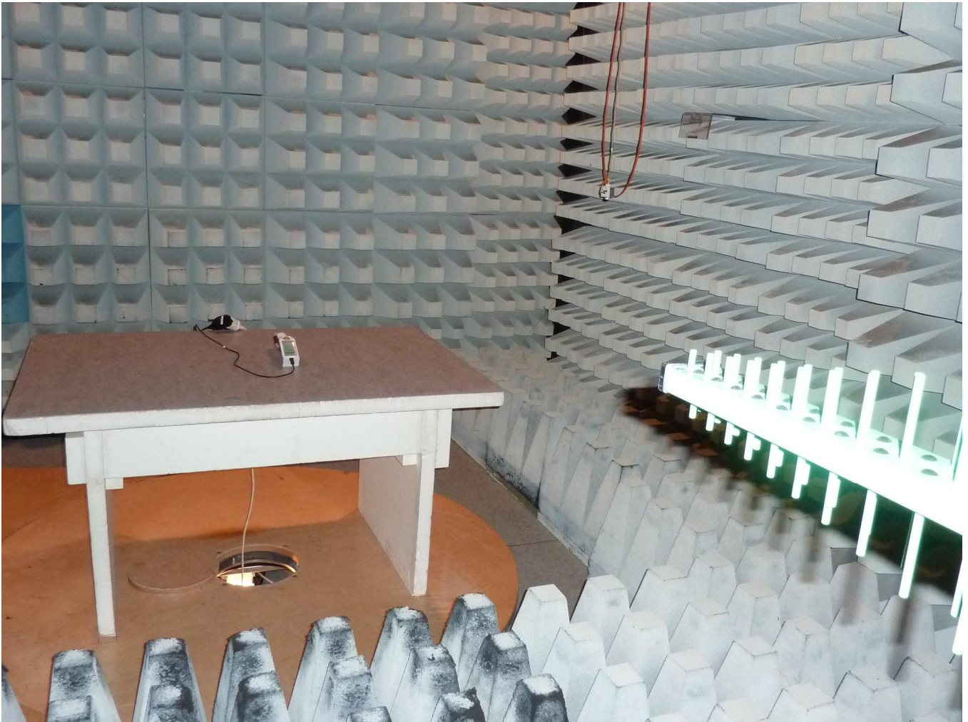
172251_209_05: test setup electric field strength fully anechoic chamber
