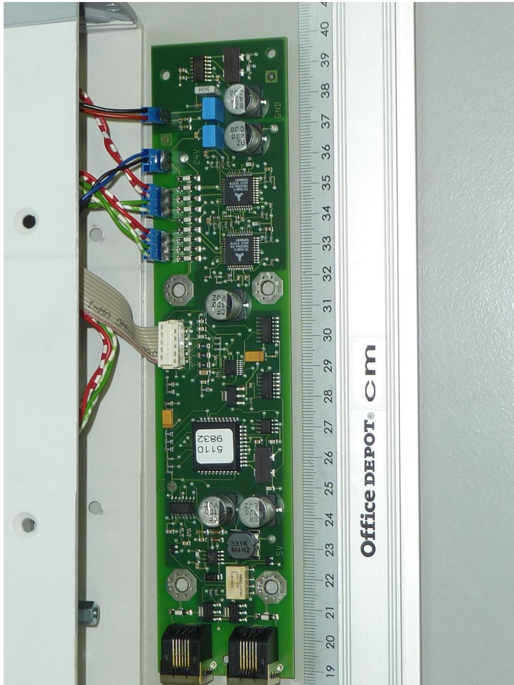
161791pcbH2.jpg: EUT (125 kHz RFID Module), PCB, top view
