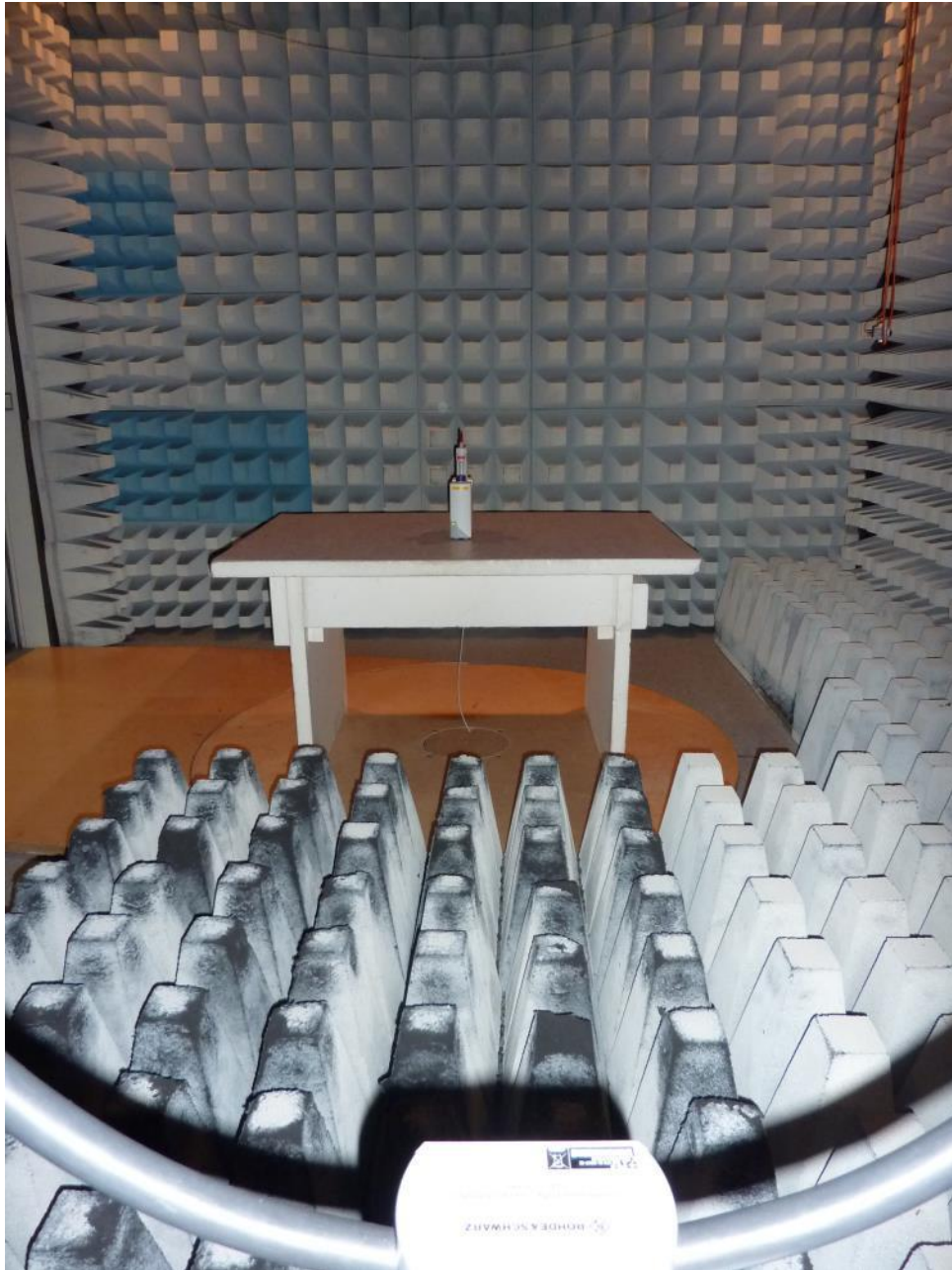
161791emiC1.jpg: Host (Dosing Unit), test setup fully anechoic chamber
