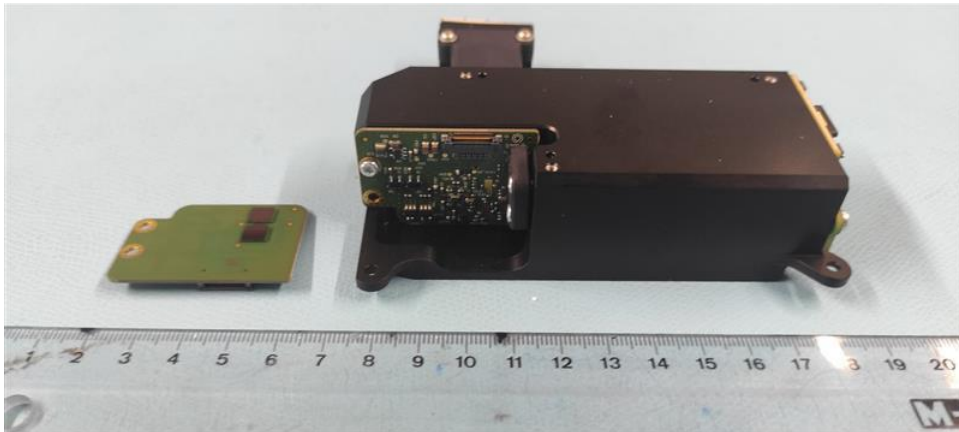
Microscope sensor PCB front and back
