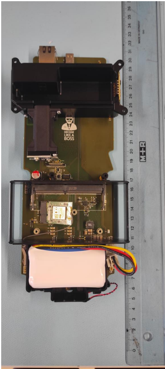
Positioning of all PCBs
