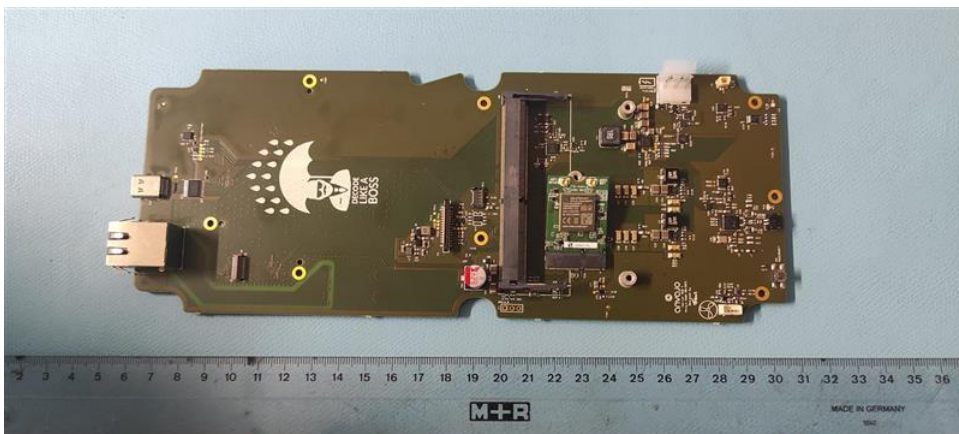
Carrier PCB
