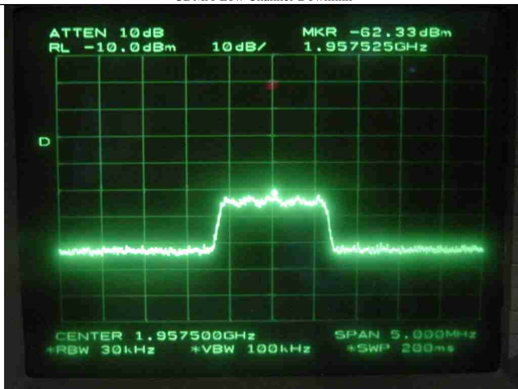
CDMA-Middle Channel-Downlink
