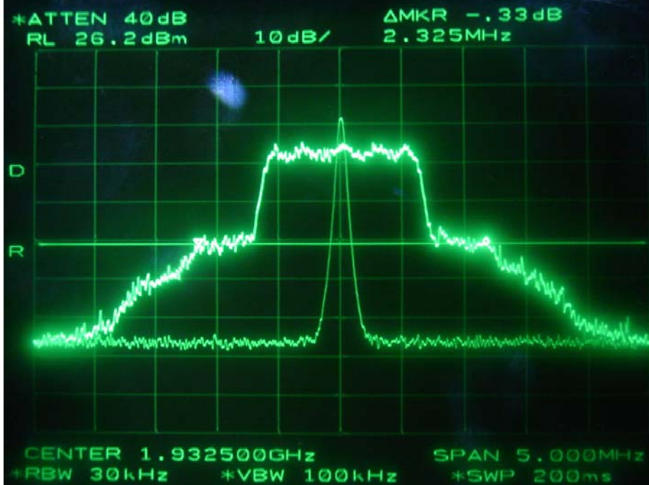
Low Channel-Downlink
