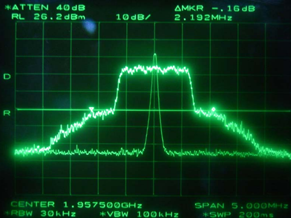
Middle Channel-Downlink
