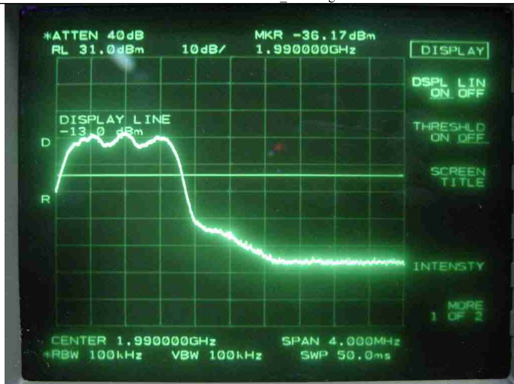
CDMA-Downlink_Bandedge
