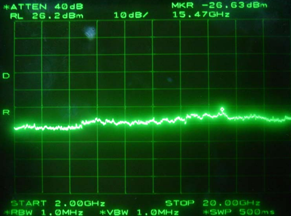
Downlink-High Channel
