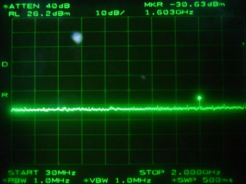
Downlink-High Channel
