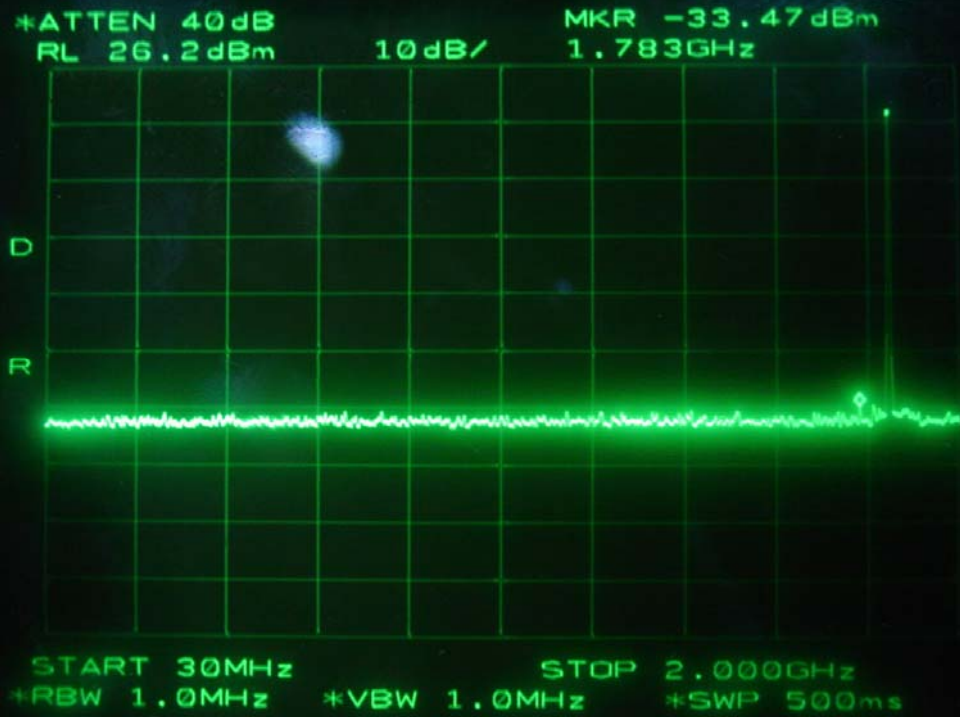
CDMA-Low Channel-Uplink
