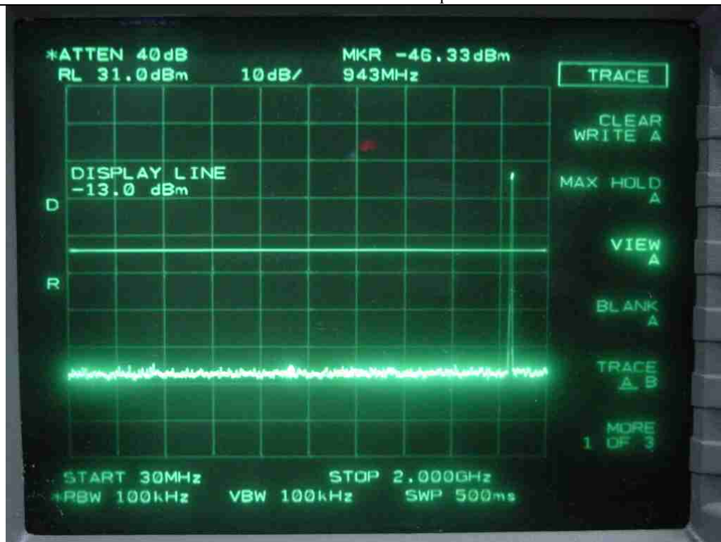
CDMA-Low Channel-Uplink
