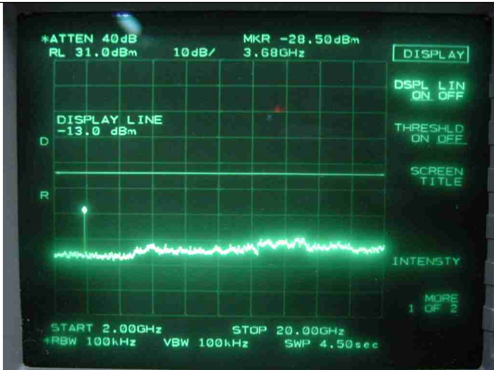
CDMA-Low Channel-Uplink
