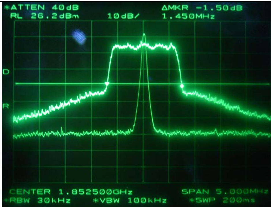
Uplink-Low Channel
