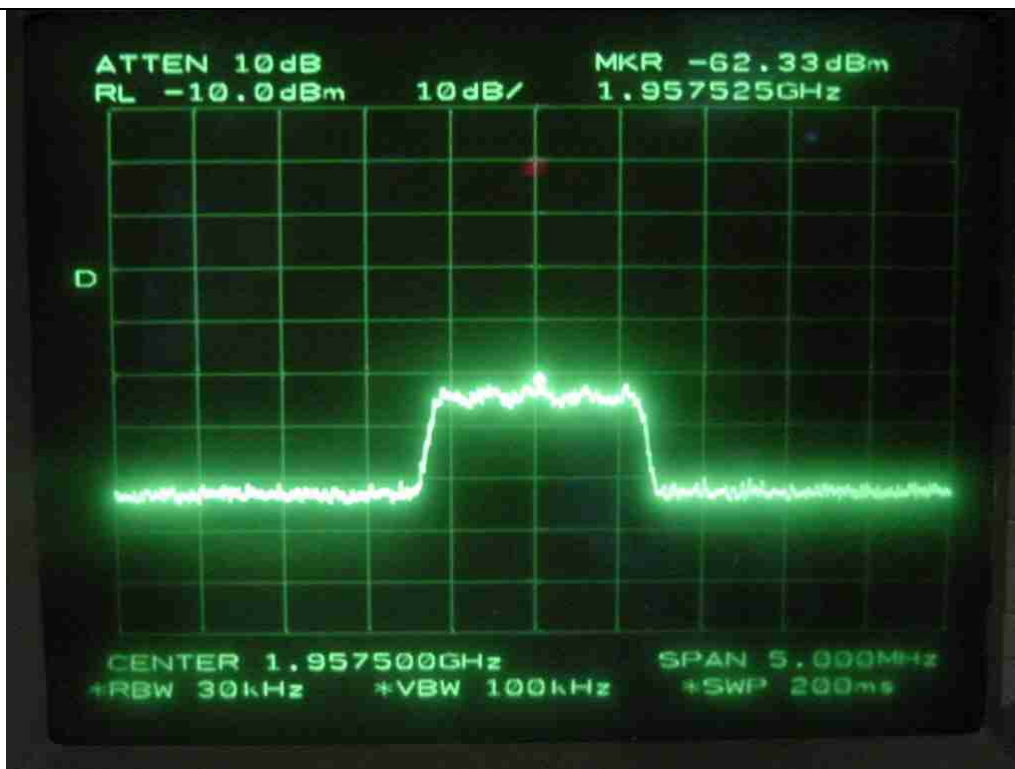
CDMA-High Channel-Downlink
