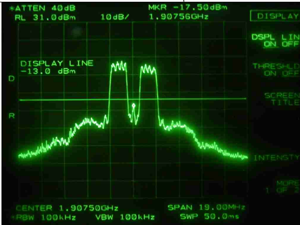
CDMA-High Channel-Uplink
