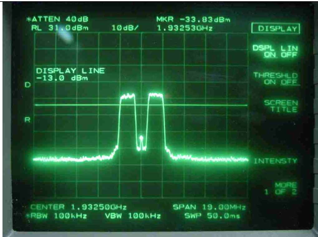
CDMA-Low Channel-Downlink
