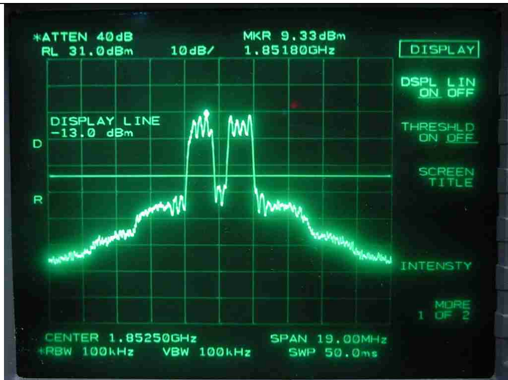
CDMA-Low Channel-Uplink
