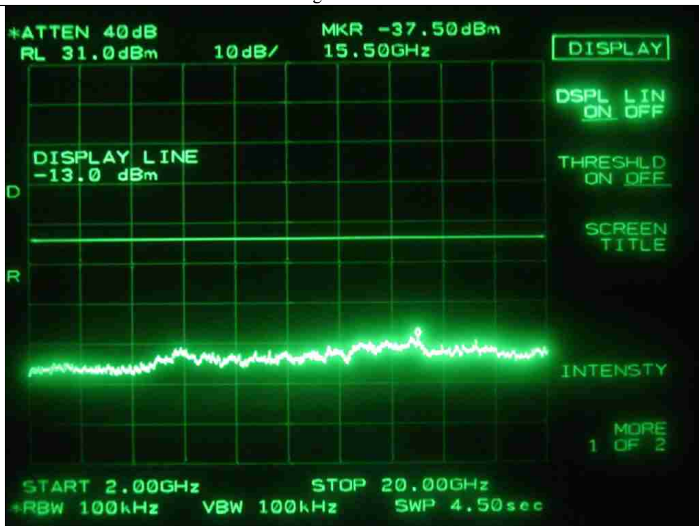
CDMA-High Channel-Downlink
