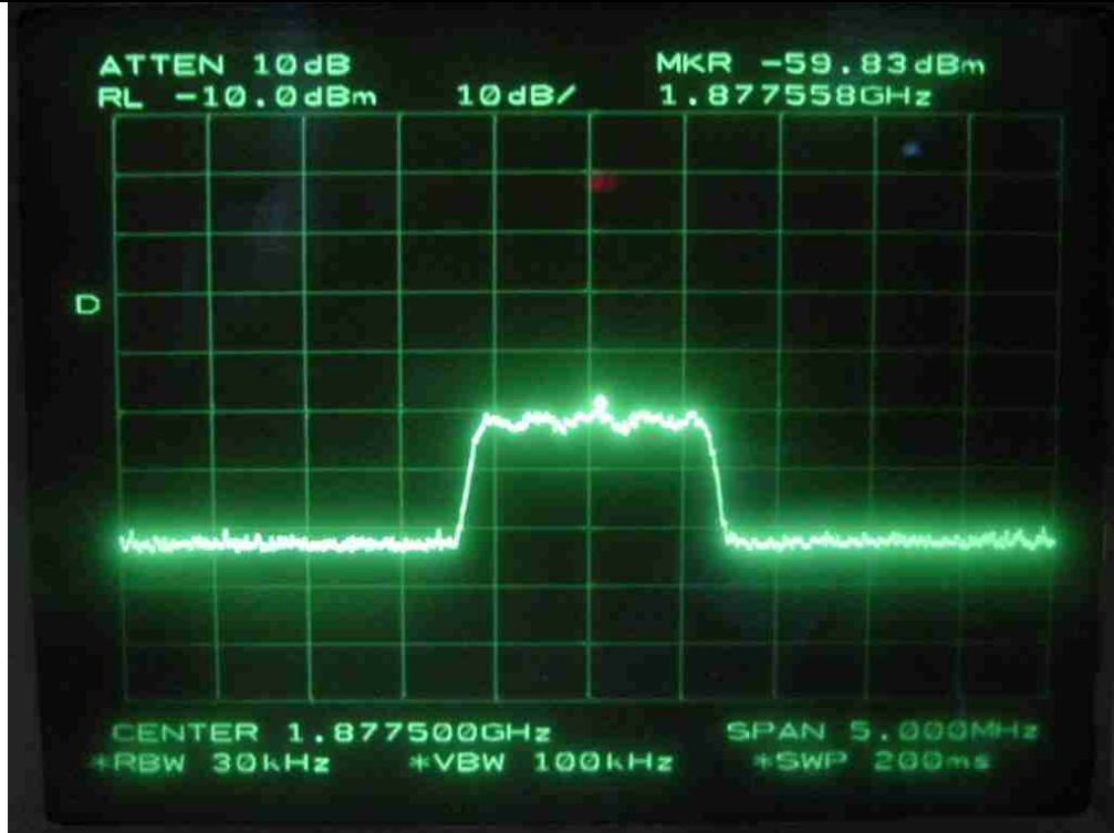
CDMA-Middle Channel-Uplink-Input
