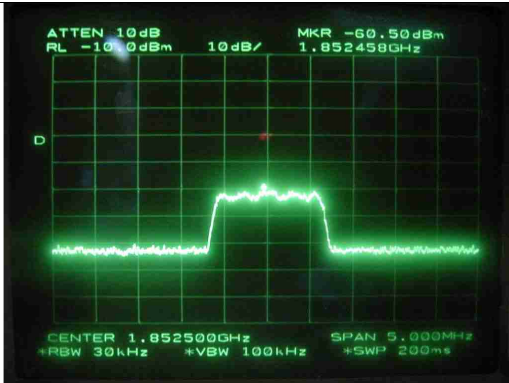
CDMA-Low Channel-Uplink-Input
