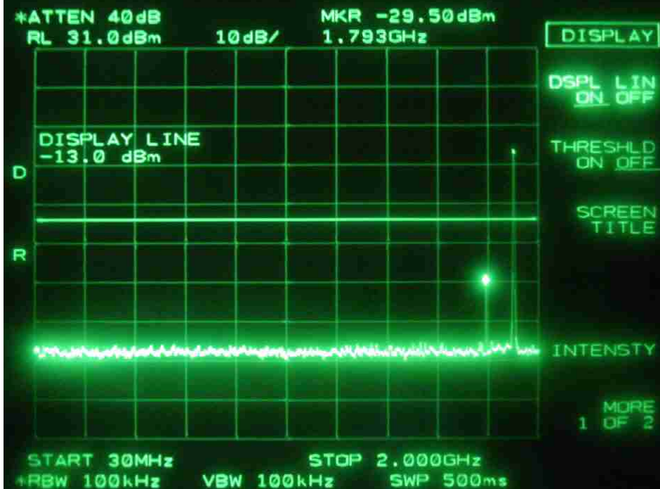
CDMA-High Channel-Uplink
