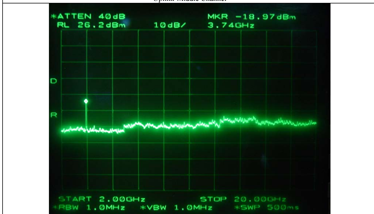
Uplink-Middle Channel
