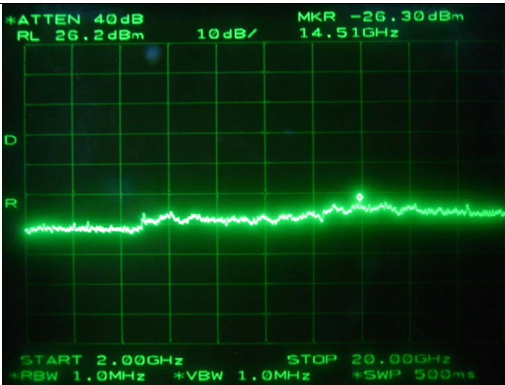
Downlink-Low Channel
