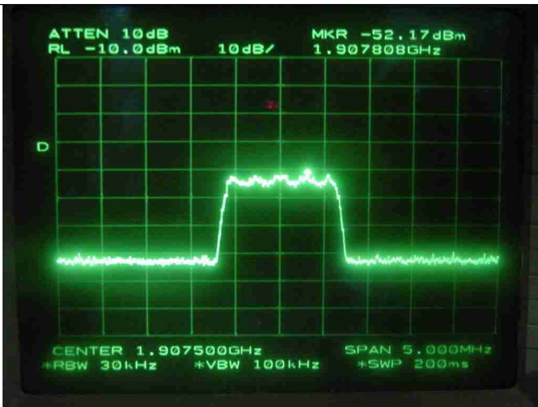
CDMA-High Channel-Uplink-Input
