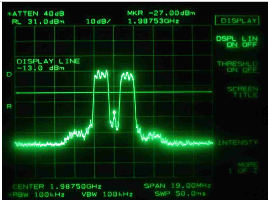
CDMA-High Channel-Downlink
