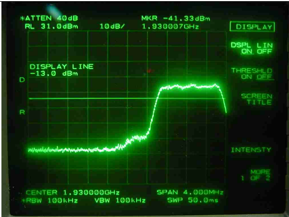
CDMA-Downlink_Bandedge
