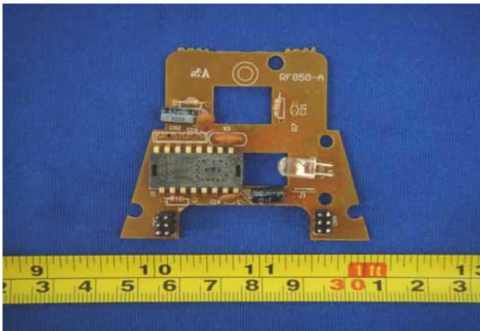
PCB(2) - Component View
