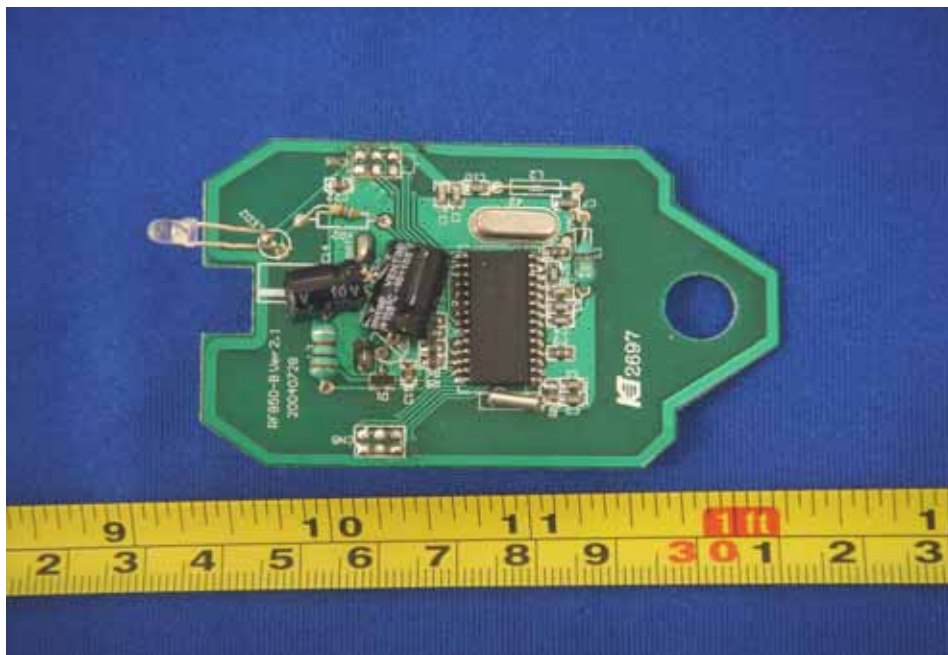
PCB(1) - Solder View
