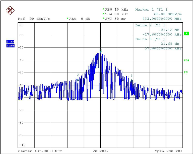
Bandwidth Plot
