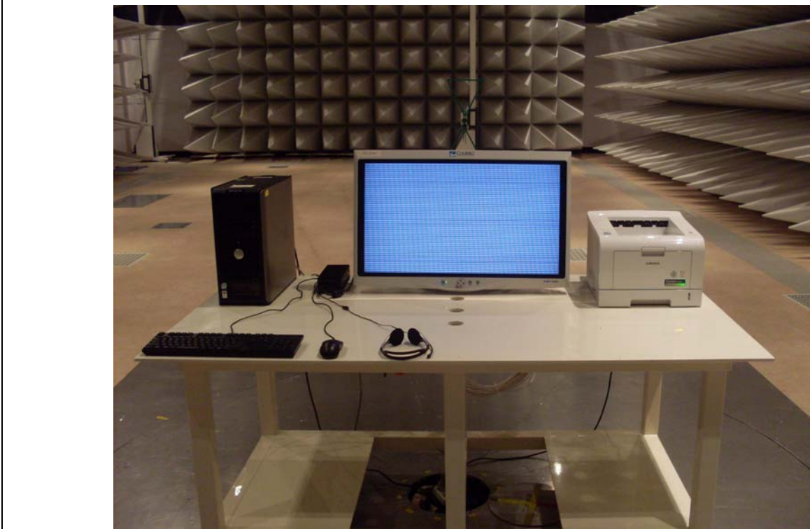
Figure 5. Photo of Radiated emission test setup for 30MHz to 1GHz
