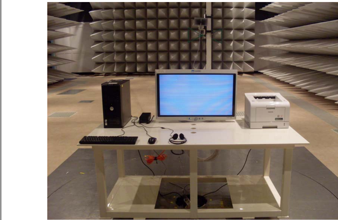
Figure 6. Photo of Radiated emission test setup for 1.0 GHz to 2.0 GHz
