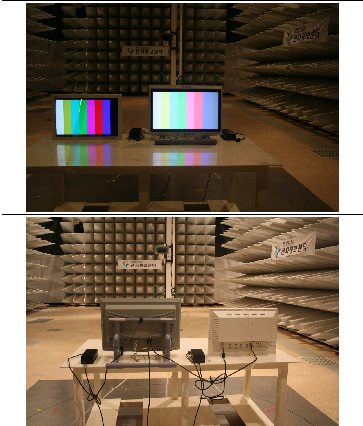
Figure 6. Photo of Radiated emission test setup: SDI In/Out Mode, 1.0 GHz to 2.0 GHz
