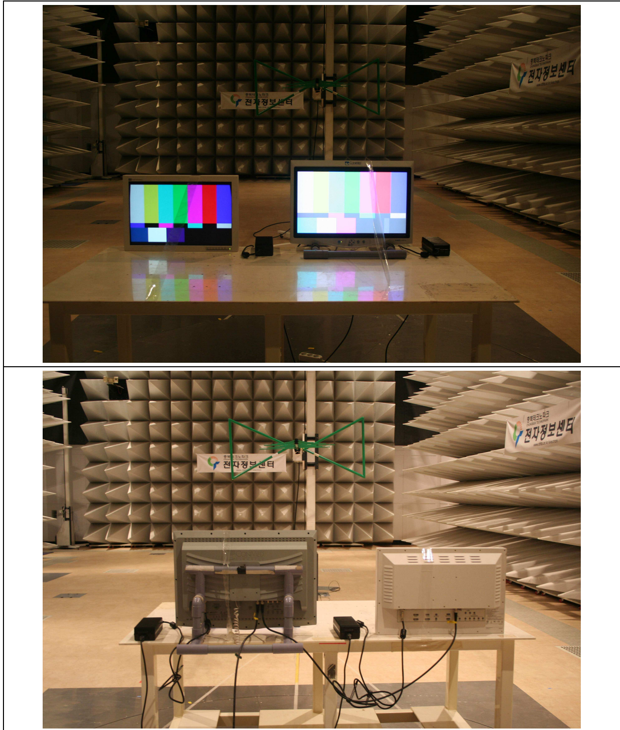
Figure 4. Photo of Radiated emission test setup: SDI In/Out Mode, 30 MHz to 1000 MHz
