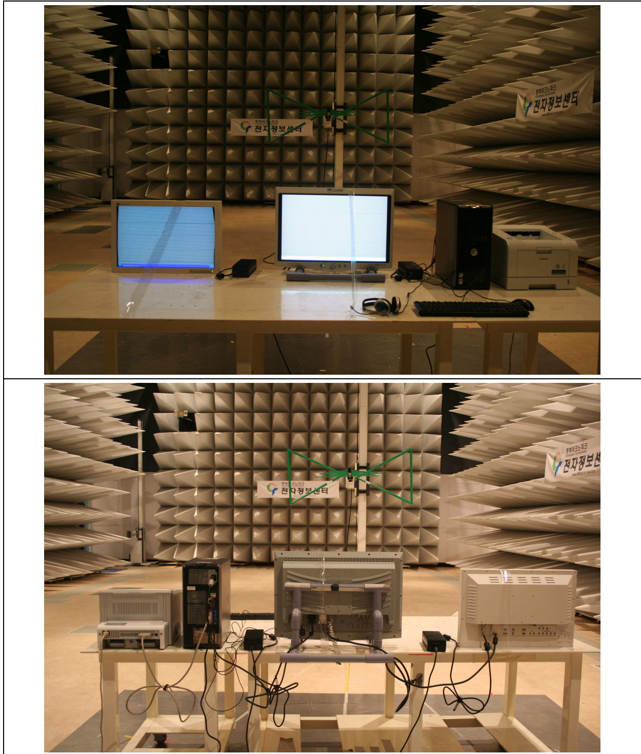
Figure 3. Photo of Radiated emission test setup: DVI In/Out Mode, 30 MHz to 1000 MHz
