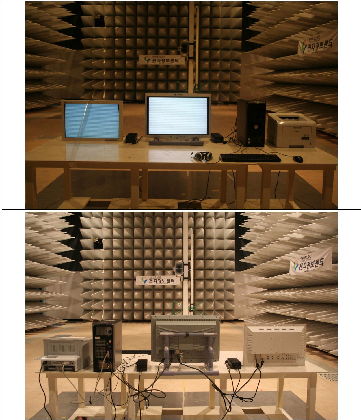
Figure 5. Photo of Radiated emission test setup: DVI In/Out Mode, 1.0 GHz to 2.0 GHz
