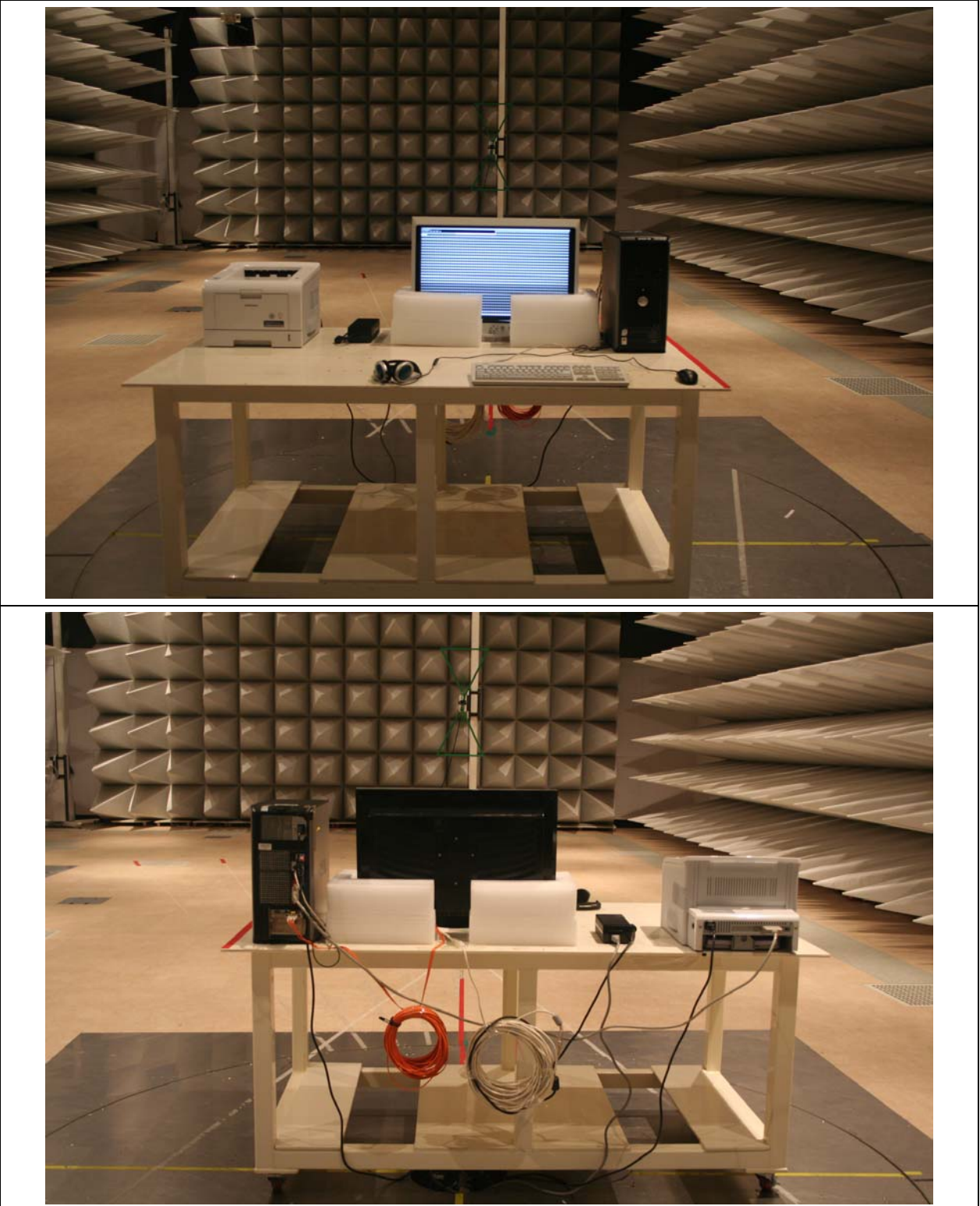
Figure 3. Photo of Radiated emission test setup for Optical DVI Mode, 30MHz to 1GHz
