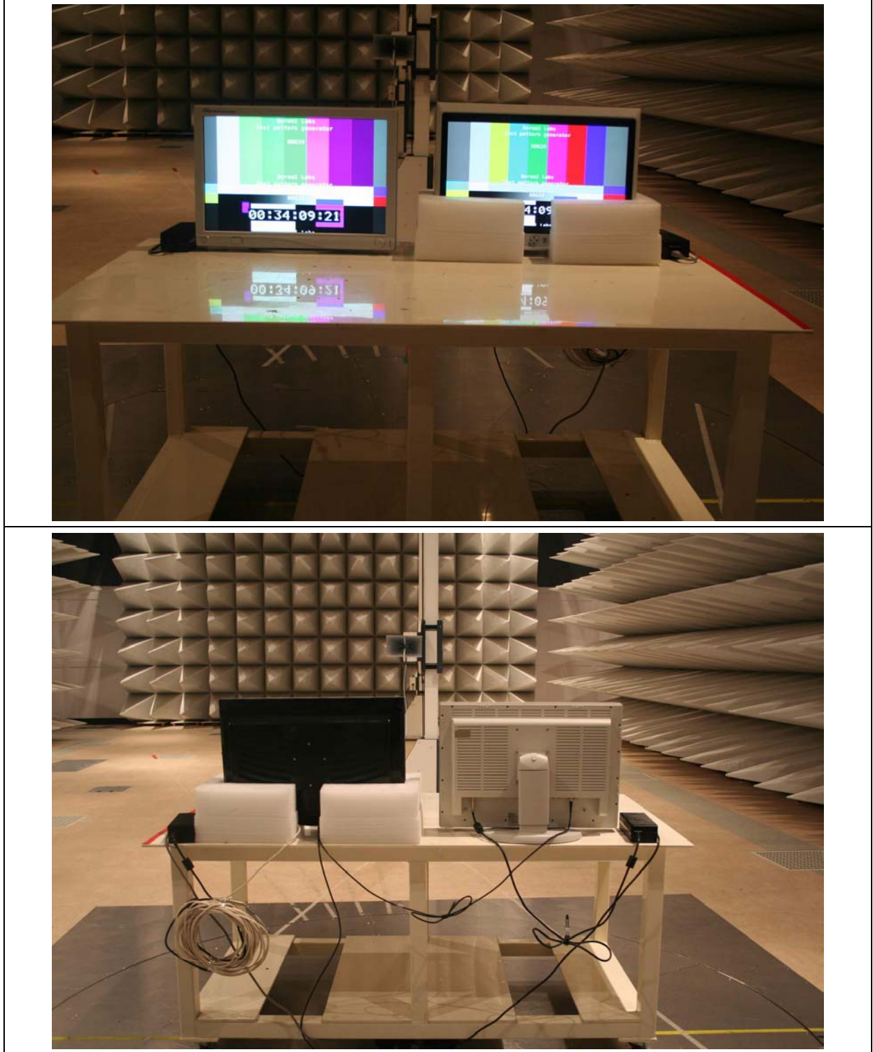
Figure 6. Photo of Radiated emission test setup for SDI In/Out Mode, 1GHz to 2GHz
