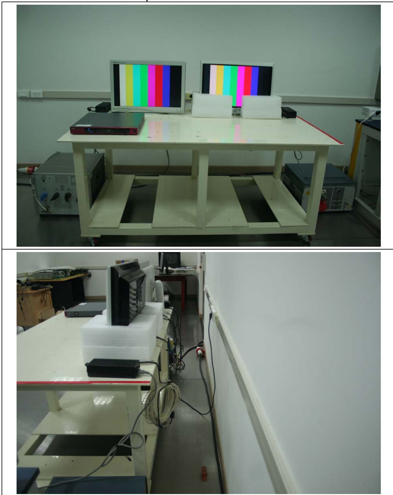
Figure 2. Conducted Emission Test Setup for SDI In/Out Mode
