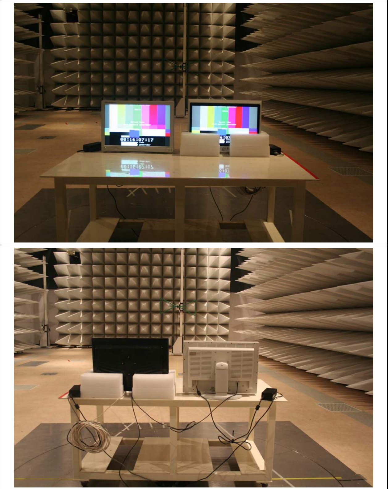
Figure 5. Photo of Radiated emission test setup for SDI In/Out Mode, 30MHz to 1GHz
