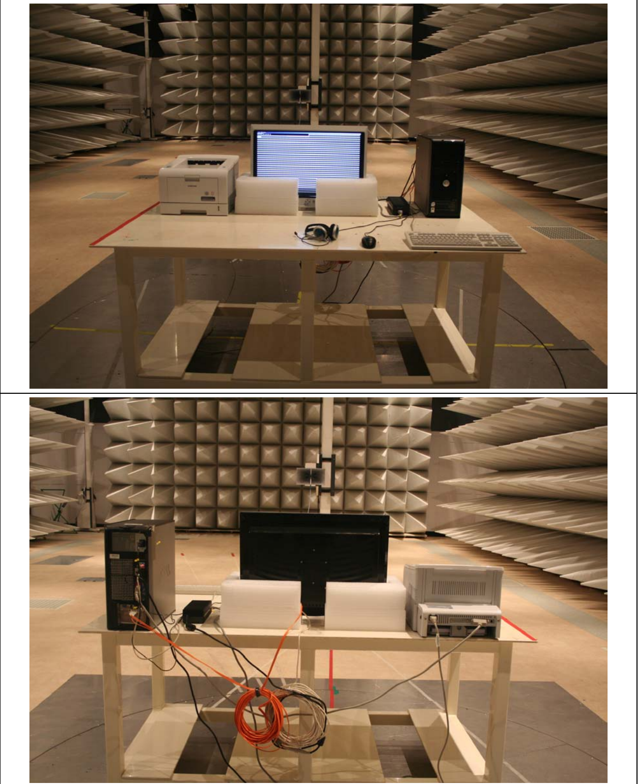
Figure 4. Photo of Radiated emission test setup for Optical DVI Mode, 1GHz to 2GHz
