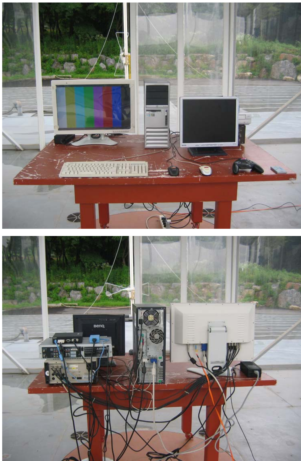
Figure 4 Photo of Radiated emission test setup: SDI Mode
