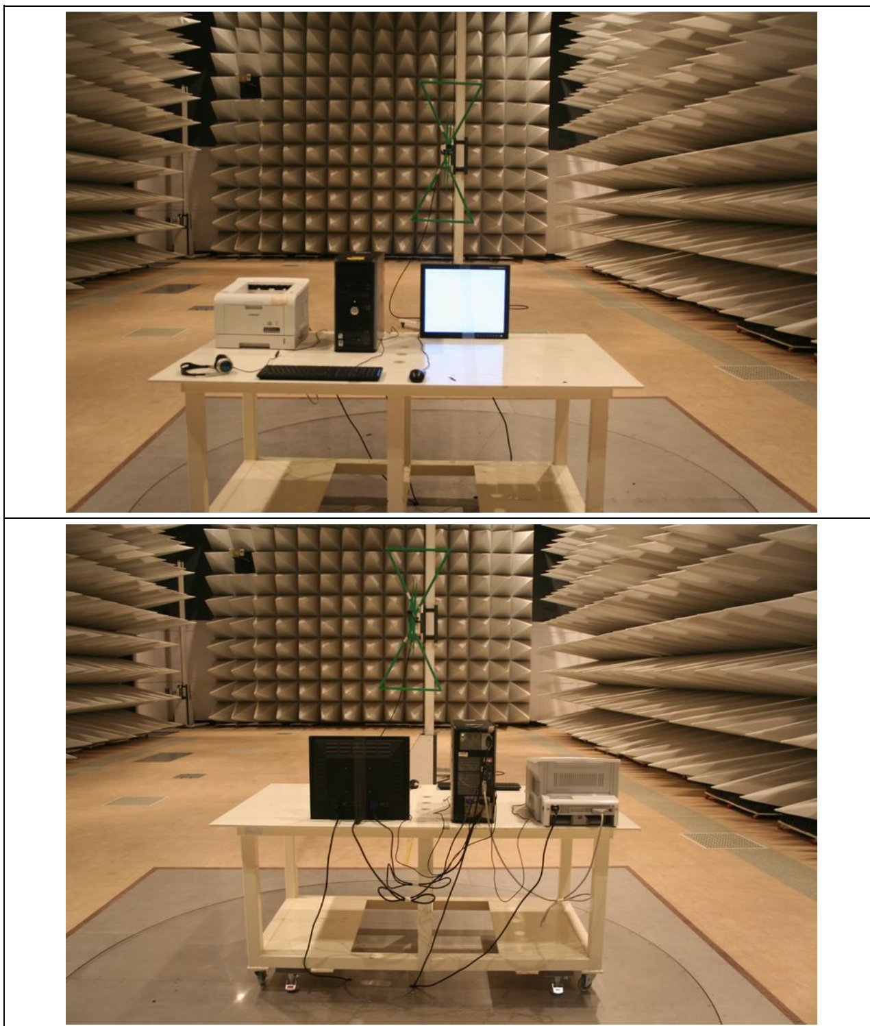
Figure 2. Photo of Radiated emission test setup for 30MHz to 1GHz
