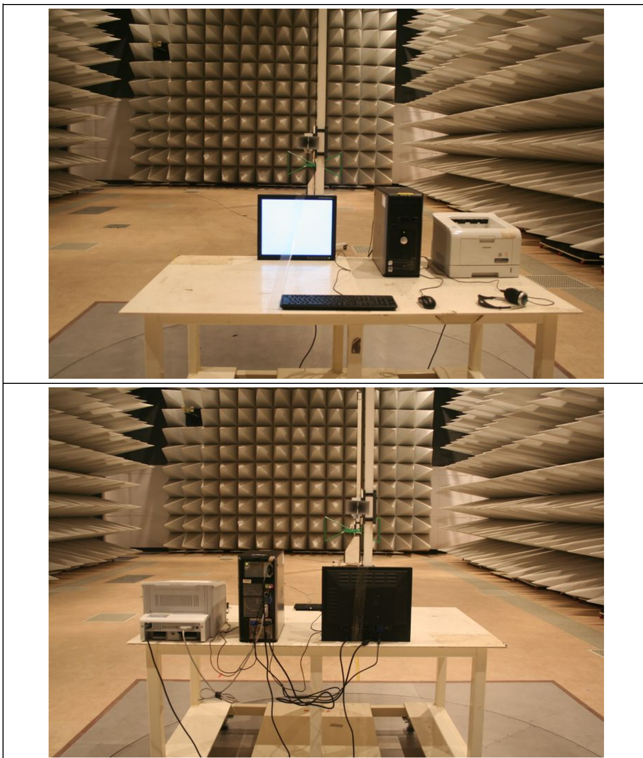
Figure 3. Photo of Radiated emission test setup for 1GHz to 2GHz
