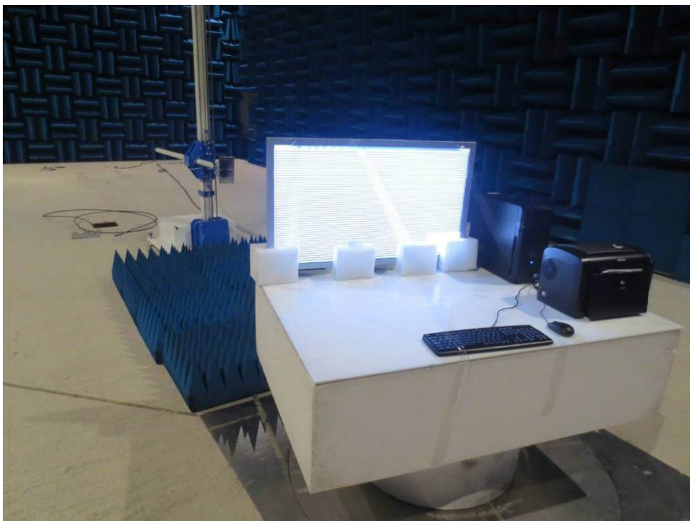
Figure 3. Radiated Emission Test Setup for Above 1GHz
