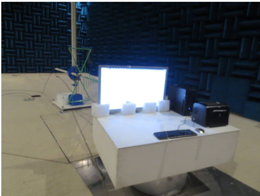
Figure 2. Radiated Emission Test Setup (30 MHz ~ 1 GHz)
