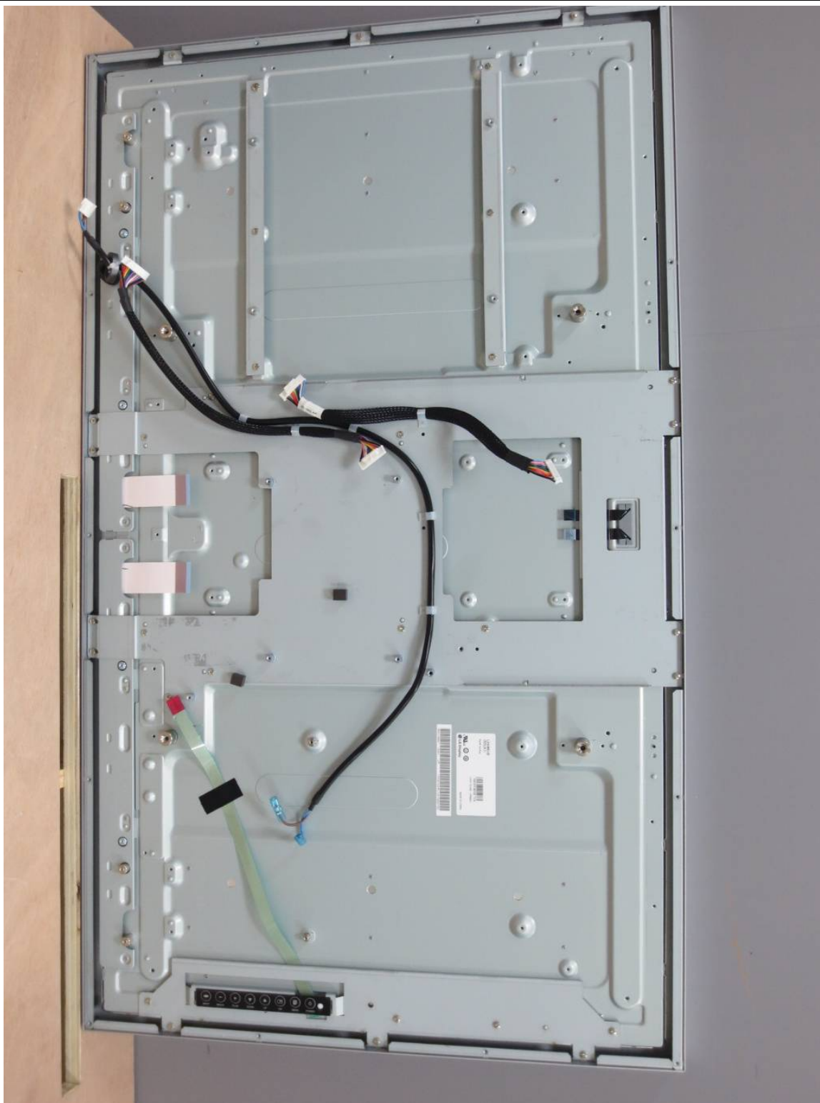
LCD View Bottom
