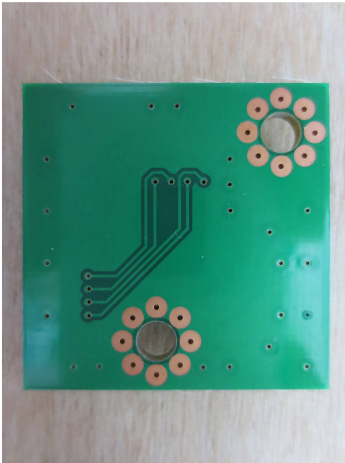
SUB BOARD View Bottom
